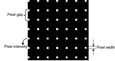
Figure 2: Our backdoor trigger has three parameters: pixel intensity \alpha , pixel gap g , and pixel width w . For presentation clarity, we use high pixel intensity here, but in experiments we use low intensities to ensure attack stealth.
