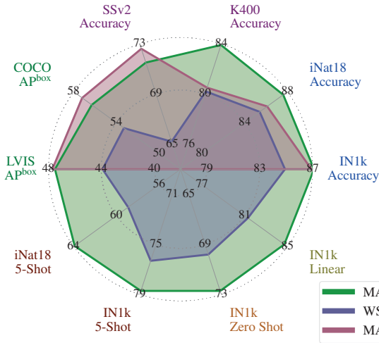
Figure 6: MAE initialization for medium scale data. Results for a ViT-L trained on IN21k with MAE, WSP, and MAE→WSP. MAE pre-pretraining improves WSP results by a wide margin.
