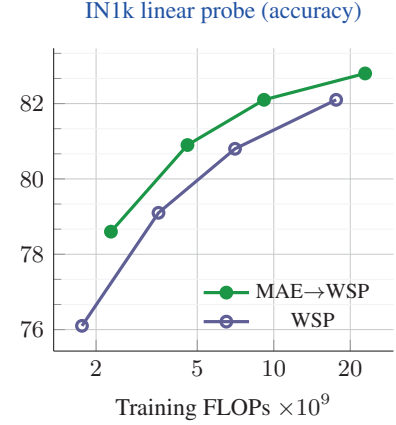
Figure 5: MAE→WSP is more FLOPs efficient than WSP. Across a wide range of training FLOP profiles for a ViT-B computed by varying WSP (and MAE) epochs, MAE→WSP outperforms a baseline WSP only model.
