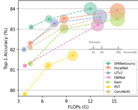
Figure 5: ImageNet-1K validation accuracy vs. FLOPs/Params for SPANets and other comparative models. The size of each bubble is proportional to the number of parameters in a variant within a model family.
