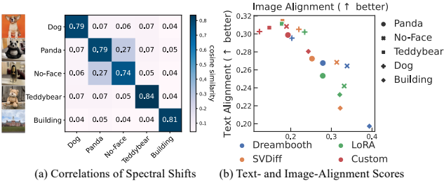
Figure 9. (a) Correlation of individually learned spectral shifts for different subjects. The cosine similarities between the spectral shifts of two subjects are averaged across all layers and plotted. The diagonal shows average similarities between two runs with different learning rates. (b) Text- and image-alignment for single-subject generation. The generated image is denoted as \tilde{x} . The text-alignment is measured by the CLIP score [46, 12] \cos(\tilde{x}, c) , and the image-alignment is defined as 1 - \mathcal{L}_{\text{LPIPS}}(\tilde{x}, x^*) [78].
