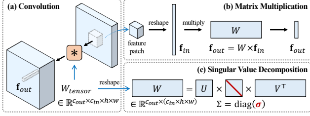
Figure 2. Performing singular value decomposition (SVD) on weight matrices. In an intermediate layer of the model, (a) the convolutional weights W_{\text{tensor}} (b) serve as an associative memory [8]. (c) SVD is performed on the reshaped 2-D matrix W .
