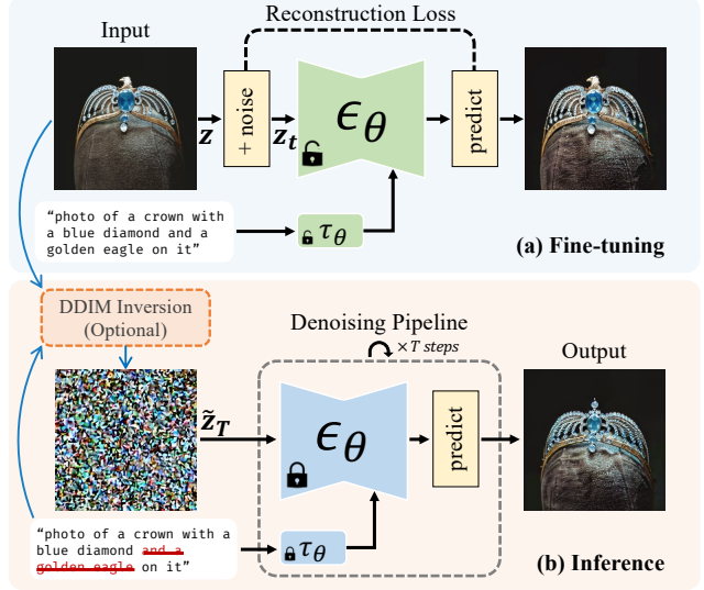
Figure 4. Pipeline for single image editing with a text-to-image diffusion model. (a) The model is fine-tuned with a single image-prompt pair, where the prompt describes the input image without a special token. (b) During inference, desired edits are made by modifying the prompt. For edits with no significant structural changes, the use of DDIM inversion [59] has been shown to improve the editing quality.
