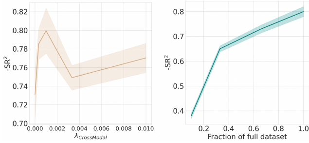
Figure 5: Plot indicating (left) necessity of the cross-modal alignment and (right) data required to train ProbVLM.
