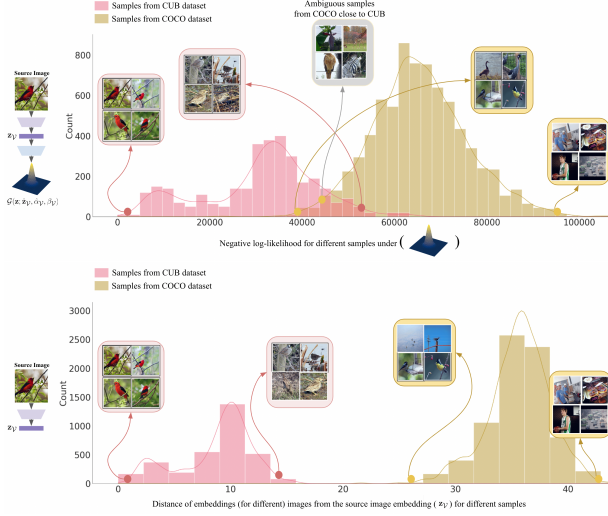
Figure 4: Visualizing the uncertainties of the vision encoder captured by ProbVLM. Fixing an image from CUB, we obtain the predicted embedding distribution and compute the likelihood of all other samples in CUB and COCO. We observe that the images in COCO are similar/ambiguous to CUB overlap (Top). However, deterministic embeddings lead to a separation between the two datasets (Bottom).
