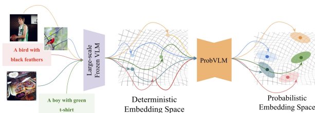
Figure 1: We provide probabilistic embeddings for deterministic pre-trained vision-language models that are frozen . By capturing the ambiguity inherently present in the inputs, we obtain well-calibrated uncertainty estimates.
