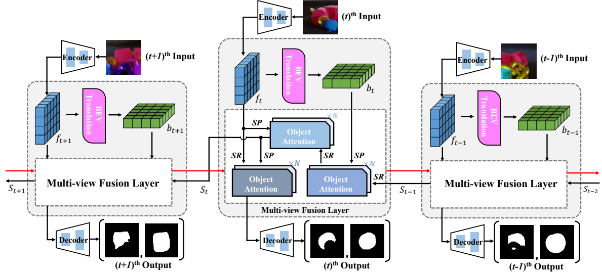
Figure 2: A schematic illustration of our method. The novelty of this architecture mainly lies in the BEV translation network and the multi-view fusion layer. The SP and SR represent the shape provider and receiver (see Section 3.1 for detail), respectively.
