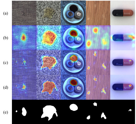
Figure 5. Qualitative comparisons with other methods: (a) the anomalous images, (b) the anomalous maps generated by PatchCore, (c) the anomalous maps of DRAEM, (d) our anomalous maps, and (e) the ground truth.
