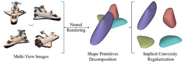
Figure 1. We propose a shape primitive decomposition method from multi-view images with a novel Implicit Convexity Regularization scheme (ICR), which theoretically guarantees the convexity of implicit primitives. Our method generates shape primitives that satisfy simplicity, semantics preserving and fidelity.
