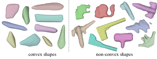
Figure 2. Convexity is a subconcept of simplicity, since a convex shape is generally regarded as simple, while a non-convex shape tends to be more complex.
