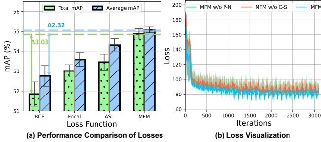
Figure 4: MLT-MLC results using different losses.
