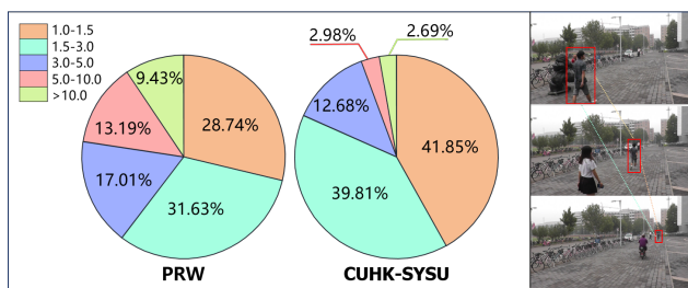
Figure 1. The scale variation of the same person on PRW and CUHK-SYSU datasets.
