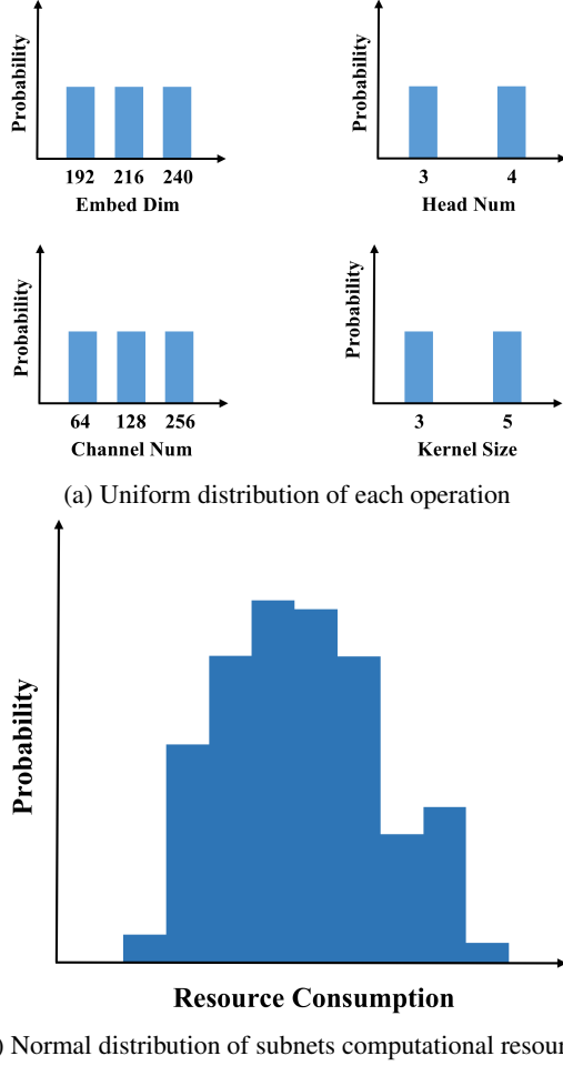
Figure 2: During supernet training, operations are sampled from a uniform distribution in each iteration. The subnet consists of the sampled operations and its computational resource follows an approximated normal distribution.
