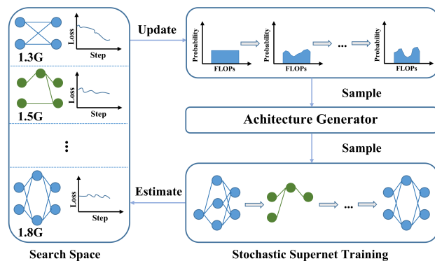
Figure 1: A conceptual overview of our ShiftNAS. Focusing on the computational resource (e.g. FLOPs), ShiftNAS split a search space into several parts where subnets have close computational complexity. In stochastic supernet training, ShiftNAS first samples computational complexity according to probability, then an architecture generator samples the subnet with desired computational complexity. The probability distribution is dynamically updated with stochastic training by estimating the performance variation of each sub-space.
