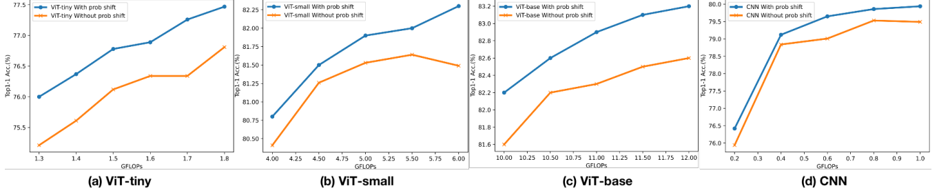
Figure 4: The effectiveness of probability shift. FLOPs/Accuracy tradeoffs of ShiftNAS with and without probability shift on search space (a) ViT-tiny; (b) ViT-small; (c) ViT-base; (d) CNN.
