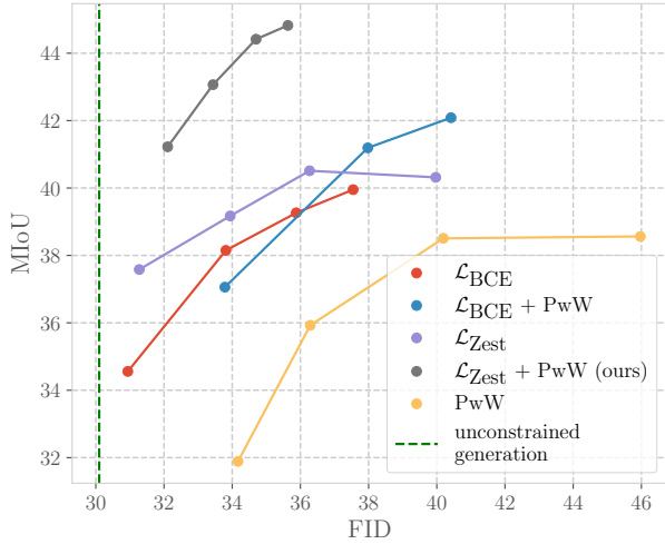
Figure 7. Trade-off in Eval-filtered setting between FID (lower is better) and mIoU (higher is better) of PwW and ZestGuide using different losses. In dotted green is shown the FID for unconstrained text-to-image generation. Using \mathcal{L}_{\text{Zest}} in combination with PwW (our default setting) gives the best trade-off.
