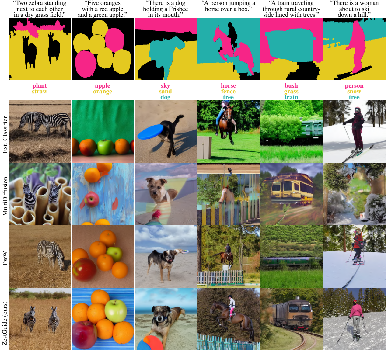
Figure 5. Qualitative comparison of ZestGuide to other methods based on LDM, conditioning on COCO captions and up to three segments.
