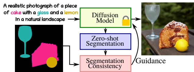
Figure 1. In ZestGuide the image generation is guided by the gradient of a loss computed between the input segmentation and a segmentation recovered from attention in a text-to-image diffusion model. The approach does not require any additional training of the pretrained text-to-image diffusion model to solve this task.
