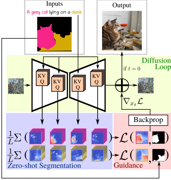
Figure 3. ZestGuide extracts segmentation maps from text-attention layers in pretrained diffusion models, and uses them to align the generation with input masks via gradient-based guidance.
