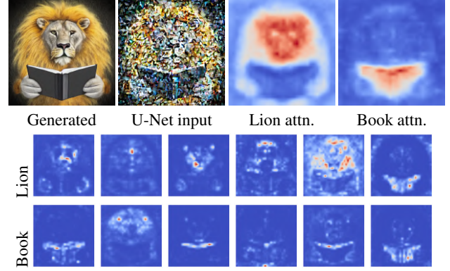
Figure 4. Top, from left to right: image generated from the prompt “A lion reading a book.”, the noisy input to the U-Net at t = 20 , cross-attention averaged over different heads and U-Net layers for “Lion” and “Book”. Bottom: individual attention heads.
