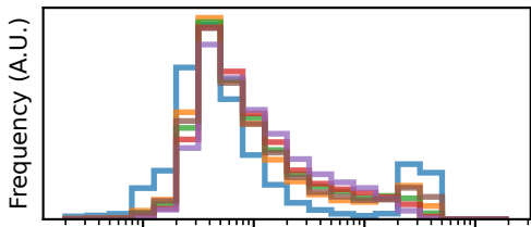
Domain sizes
