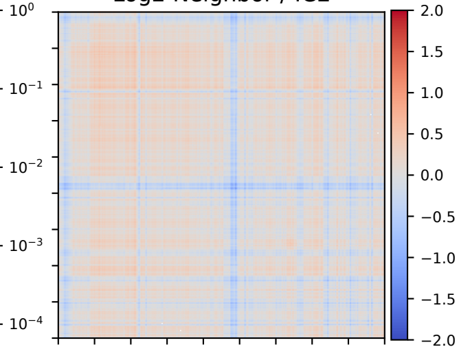
Log2 Neighbor / ICE
