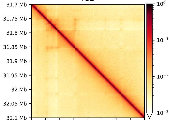
Contact density
