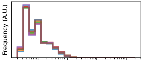
Linker sizes
