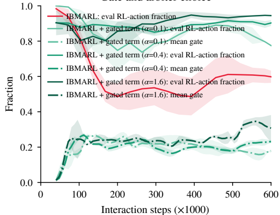
Gate and arbiter choice
