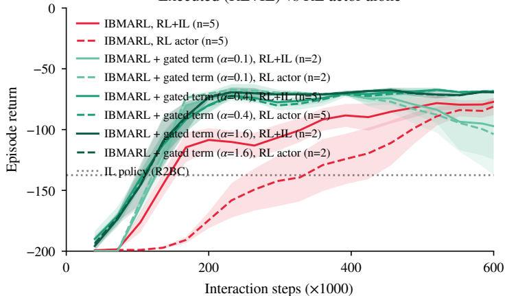
Executed (RL+IL) vs RL actor alone
