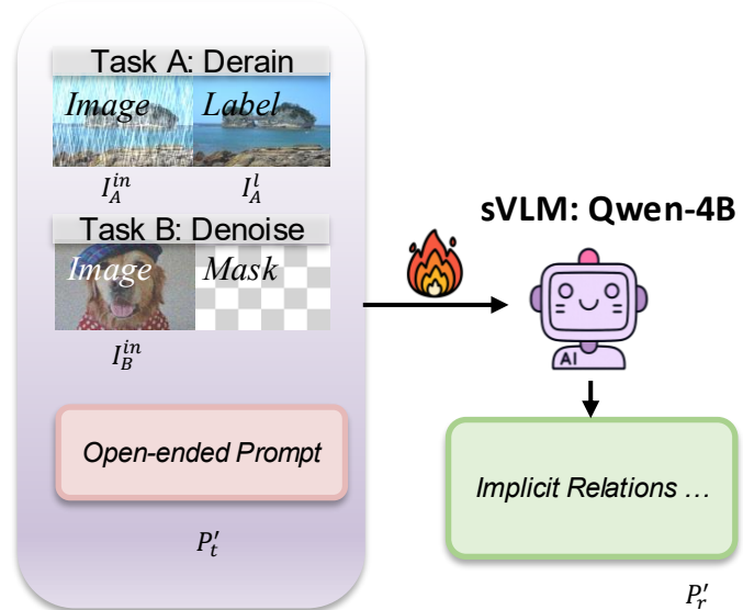
(B) VLM-sVLM Knowledge Transfer
