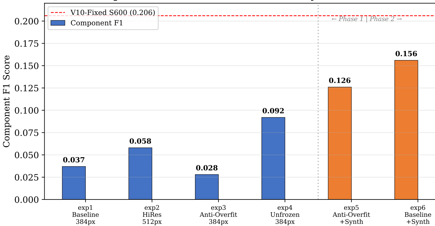
Component F1: Phase 1 vs Phase 2 (+Synthetic Data)
