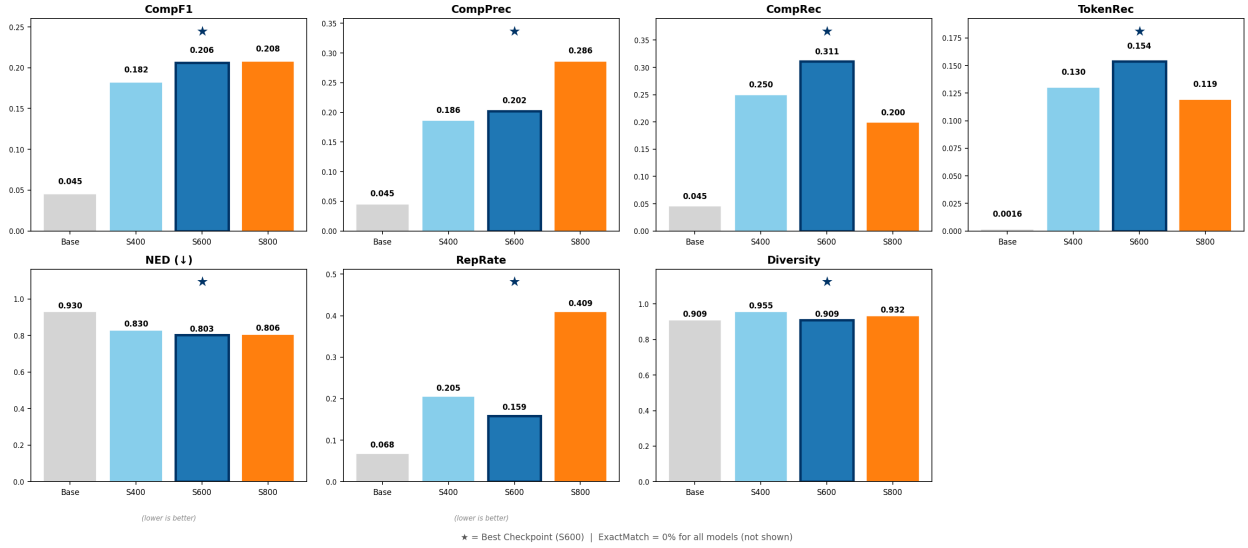
Figure 2: Phase 1 benchmark visualization across seven metrics (ExactMatch omitted: 0% for all). S600 (blue, starred) achieves the best balance. S800 (orange) shows clear overfitting.
