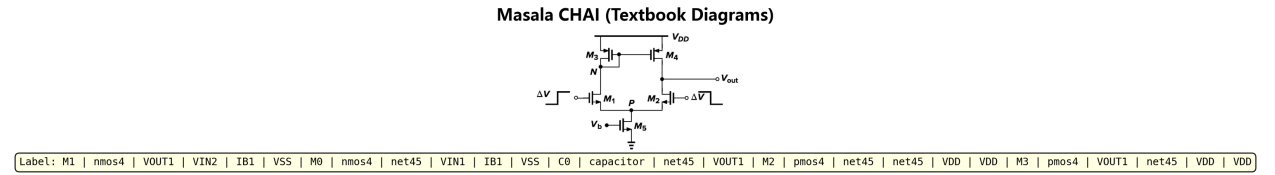
Figure 2: Dataset Source 2: Masala-CHAI — textbook circuit diagrams with standard SPICE netlist ground truth, covering analog, digital, and mixed-signal educational scenarios.
