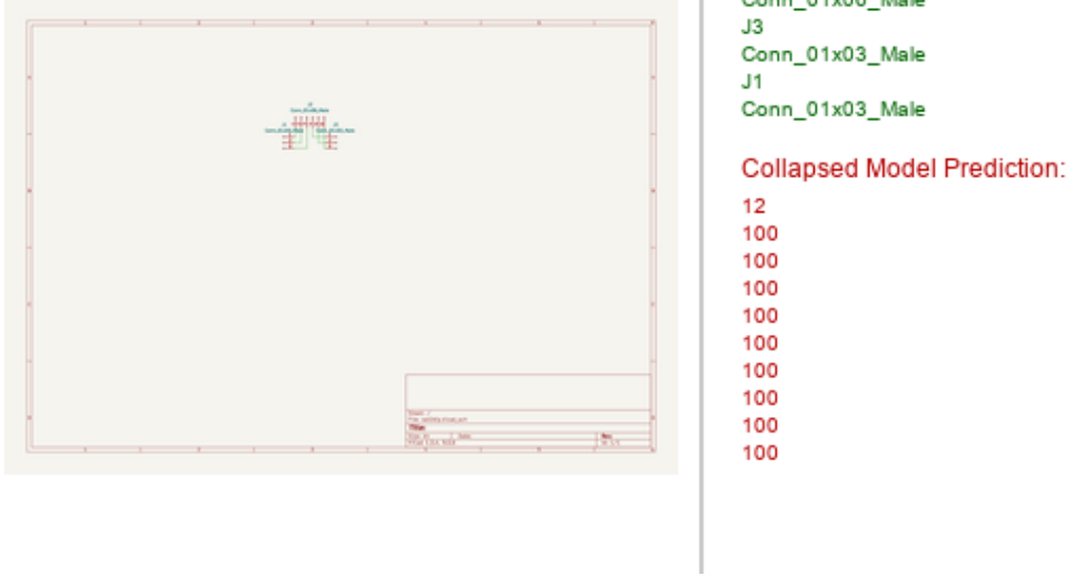
Figure 4: Old model (V4, +Projector LoRA r = 16 ) output: all 50 test samples produce the identical “12 100 100...” sequence, with an output diversity of only 4%, representing a typical modality collapse.
