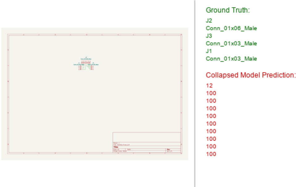
Figure 4: Old model (V4, +Projector LoRA r = 16 ) output: all 50 test samples produce the identical “12 100 100...” sequence, with an output diversity of only 4%, representing a typical modality collapse.
