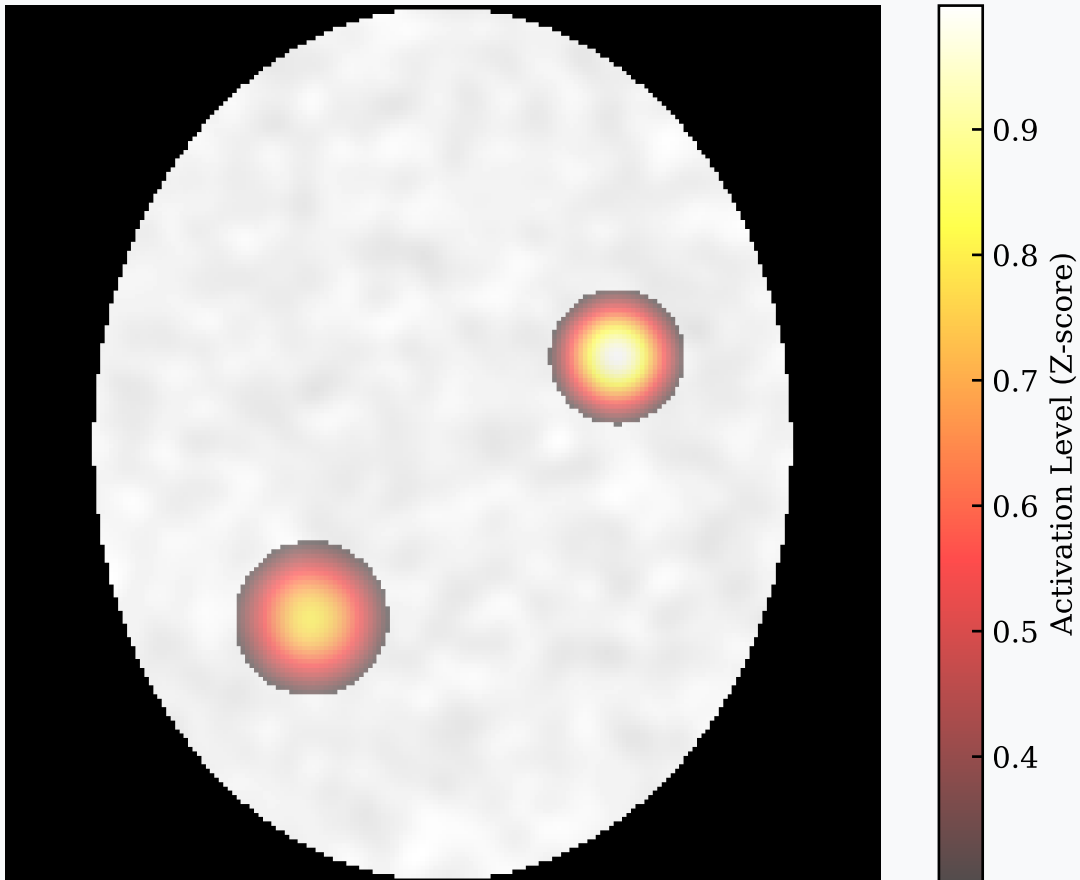
Simulated fMRI Activation Overlay
