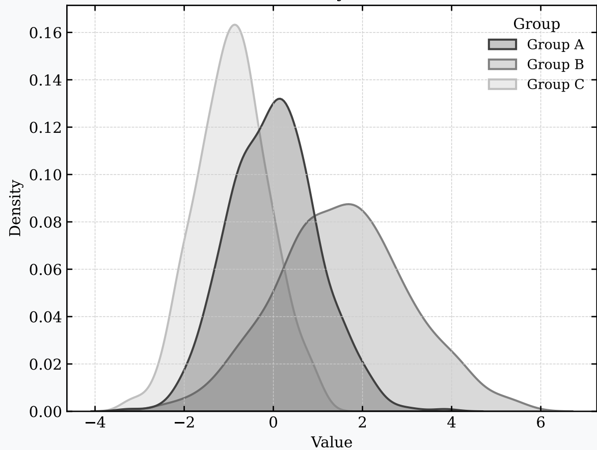
Kernel Density Estimation
