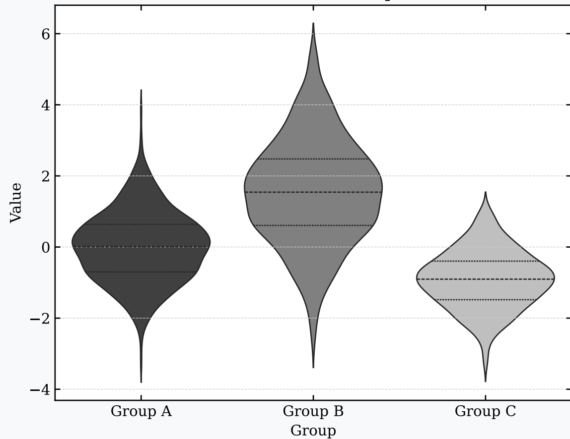
Violin Plot of Groups
