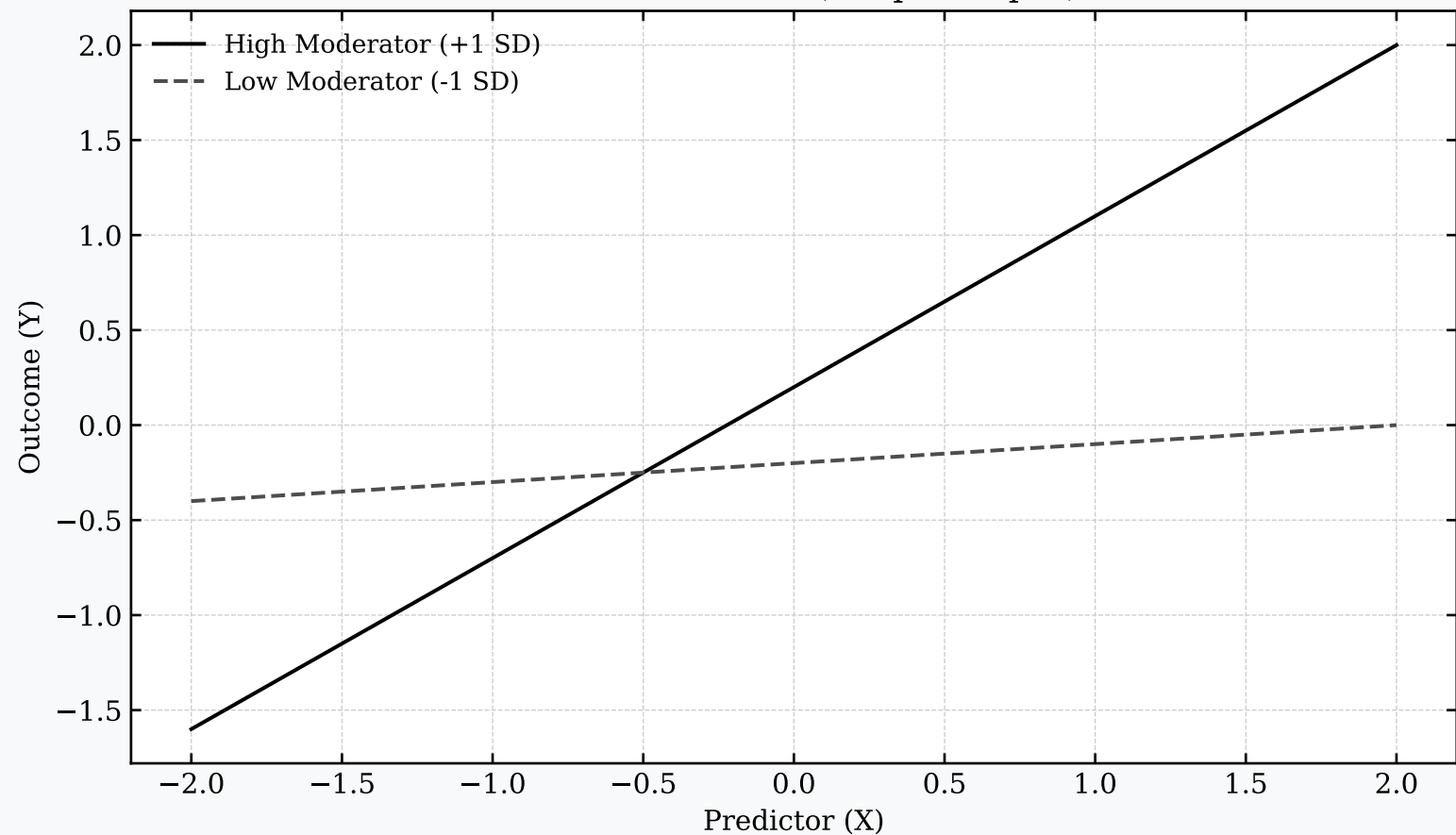
Interaction Effect (Simple Slopes)
