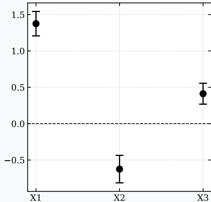
Regression Coefficients (95% CI)
