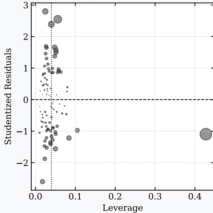
Leverage vs. Studentized Residuals (Size = Cook's D)
