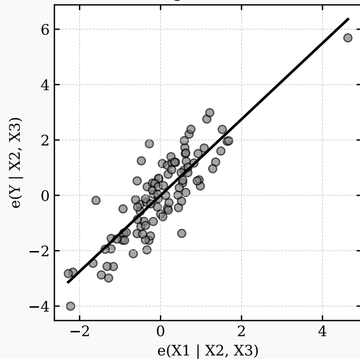
Partial Regression Plot (X1)
