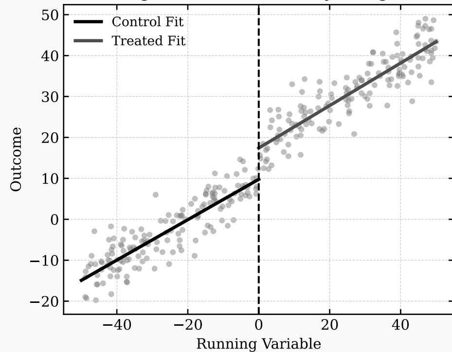
Regression Discontinuity Design
