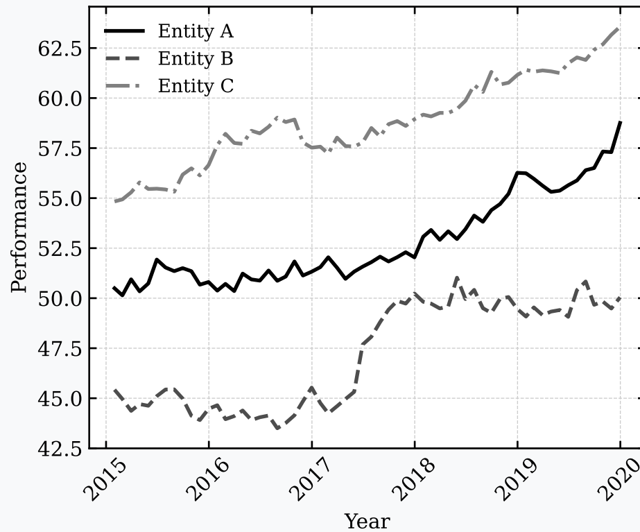
Panel Data Trends
