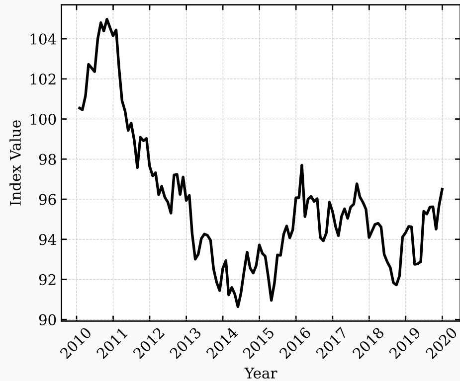
Macroeconomic Time Series
