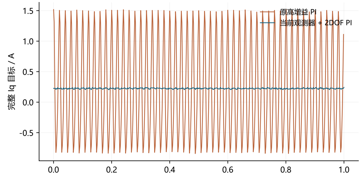
+3000 rpm 稳态
