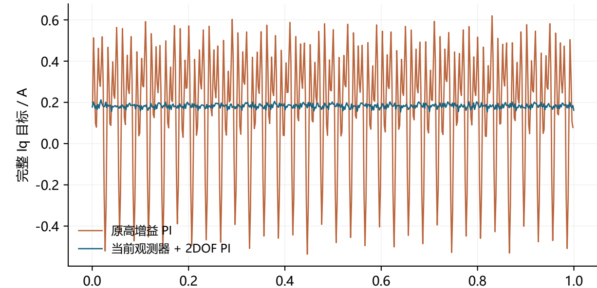
+1000 rpm 稳态
