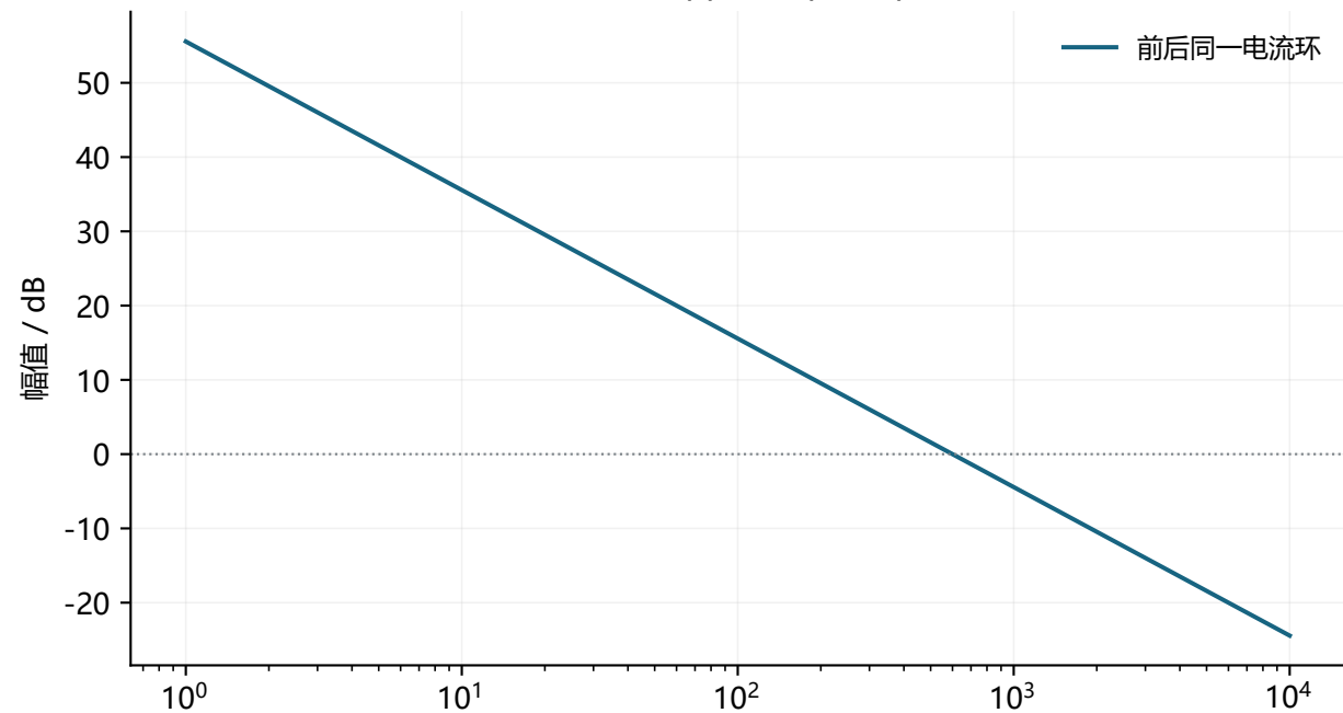
开环 C_i(s) \times 1/(Ls+R)
