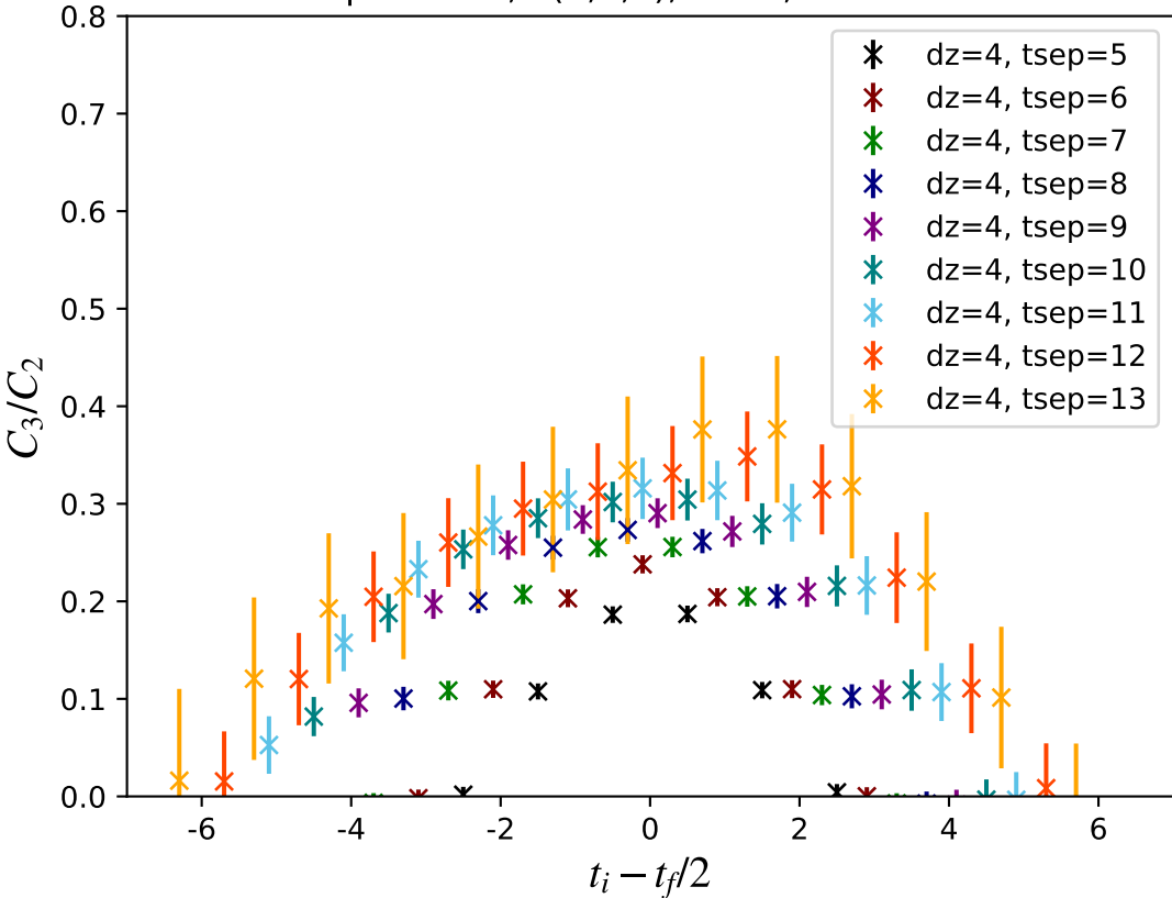
Unpolarized, P(0,0,2), z = 4 , Nconf=879
