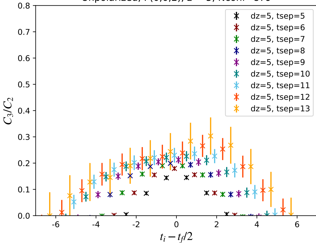
Unpolarized, P(0,0,2), z = 5 , Nconf=879
