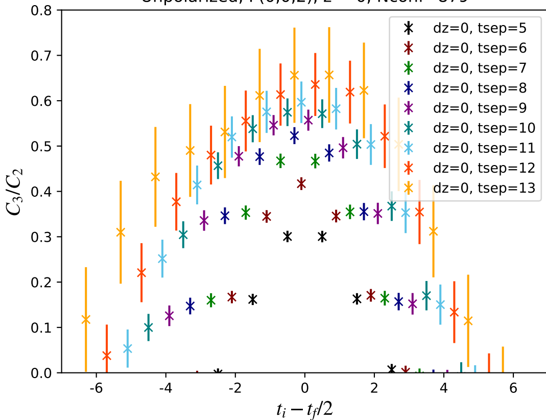
Unpolarized, P(0,0,2), z = 0 , Nconf=879
