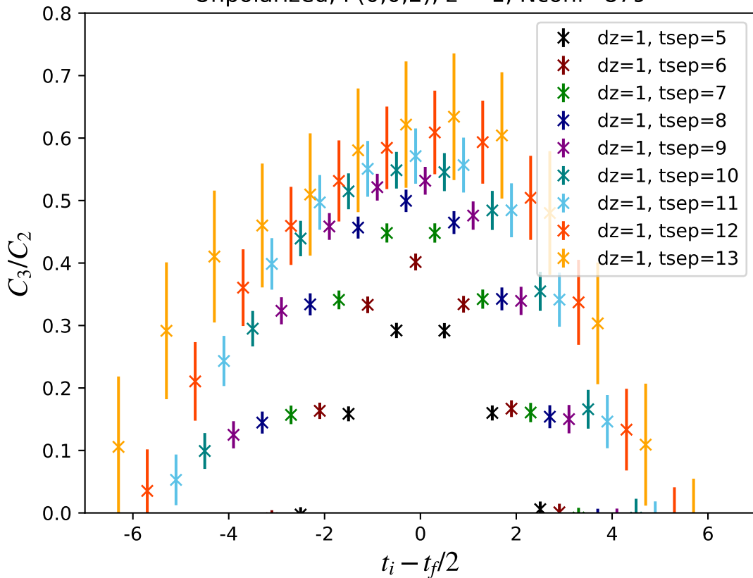
Unpolarized, P(0,0,2), z = 1 , Nconf=879
