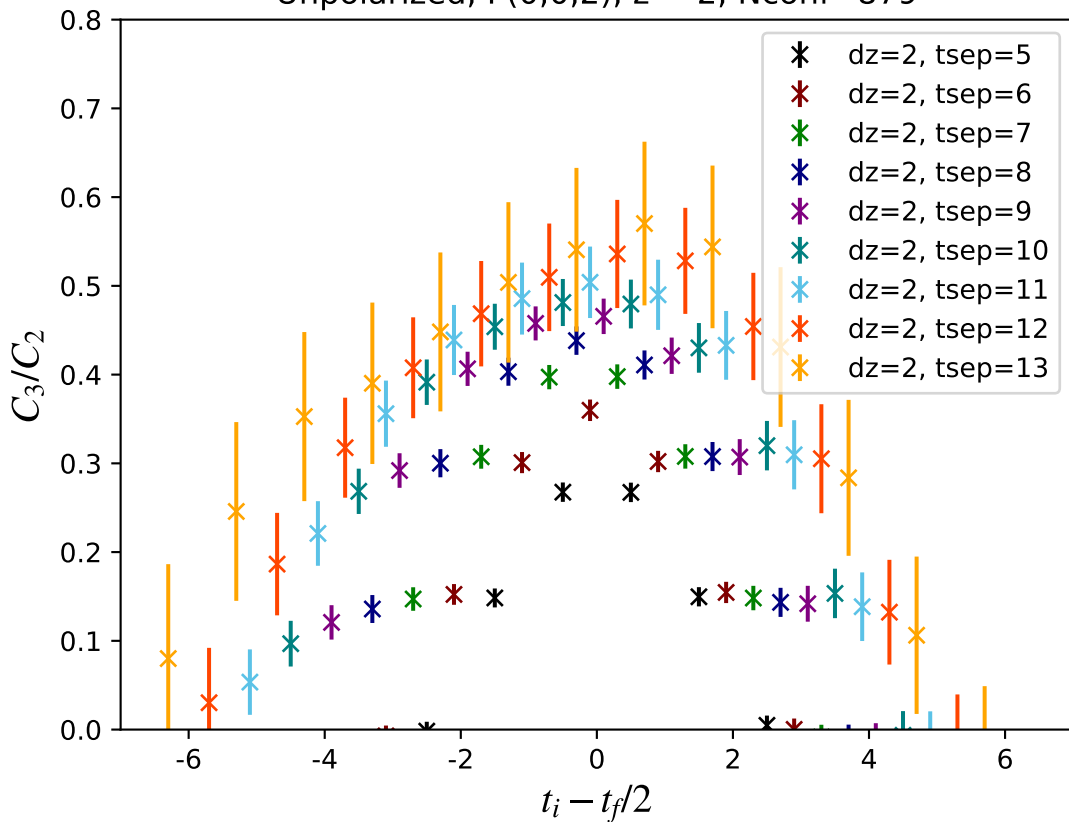
Unpolarized, P(0,0,2), z = 2 , Nconf=879
