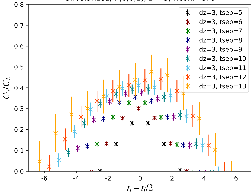
Unpolarized, P(0,0,2), z = 3 , Nconf=879
