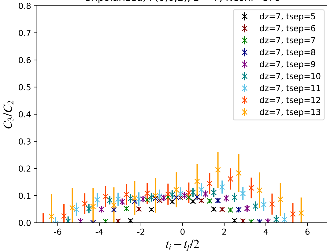
Unpolarized, P(0,0,2), z = 7 , Nconf=879
