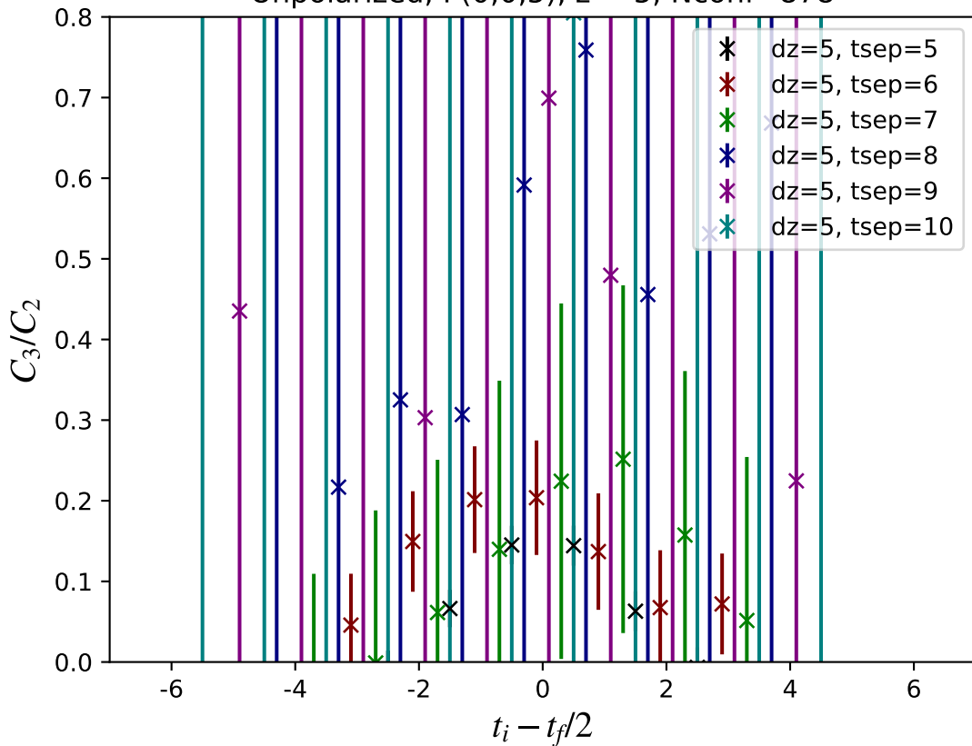
Unpolarized, P(0,0,5), z = 5 , Nconf=878
