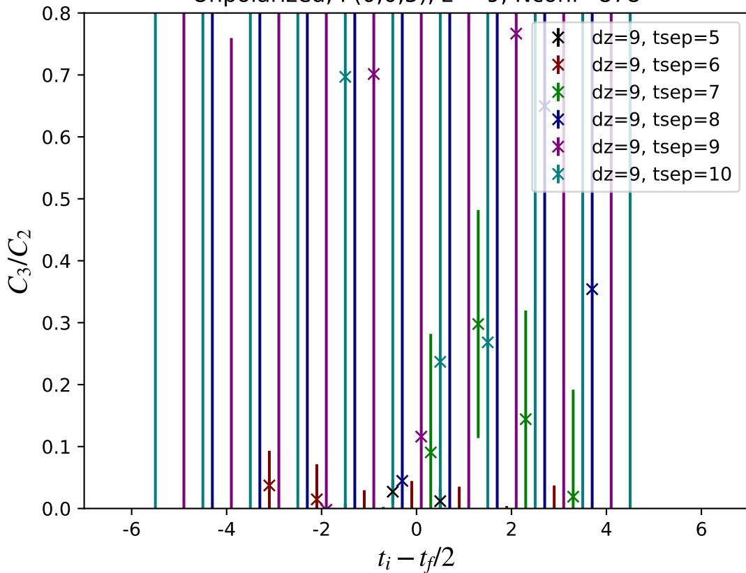
Unpolarized, P(0,0,5), z = 9 , Nconf=878
