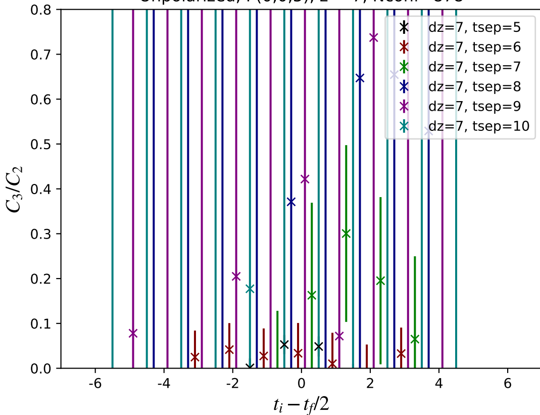
Unpolarized, P(0,0,5), z = 7 , Nconf=878
