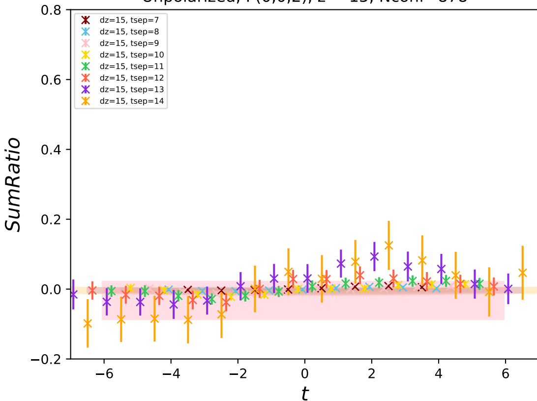
Unpolarized, P(0,0,2) , z = 15 , Nconf=878
