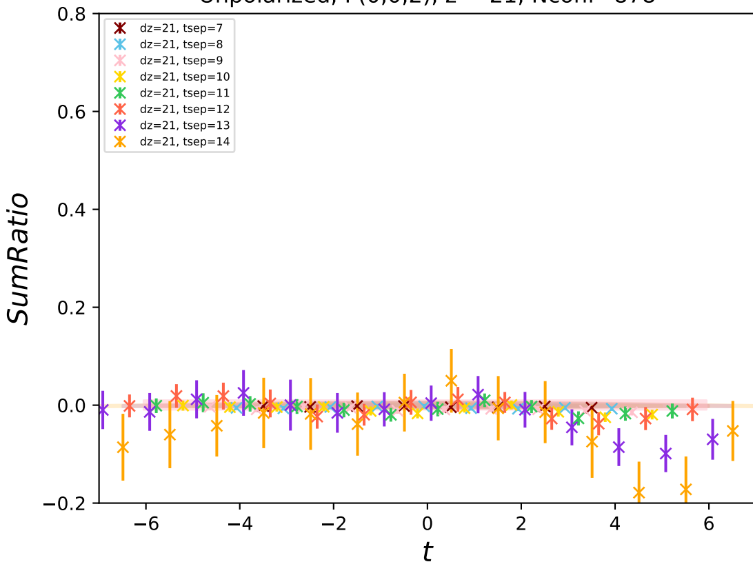
Unpolarized, P(0,0,2) , z = 21 , Nconf=878
