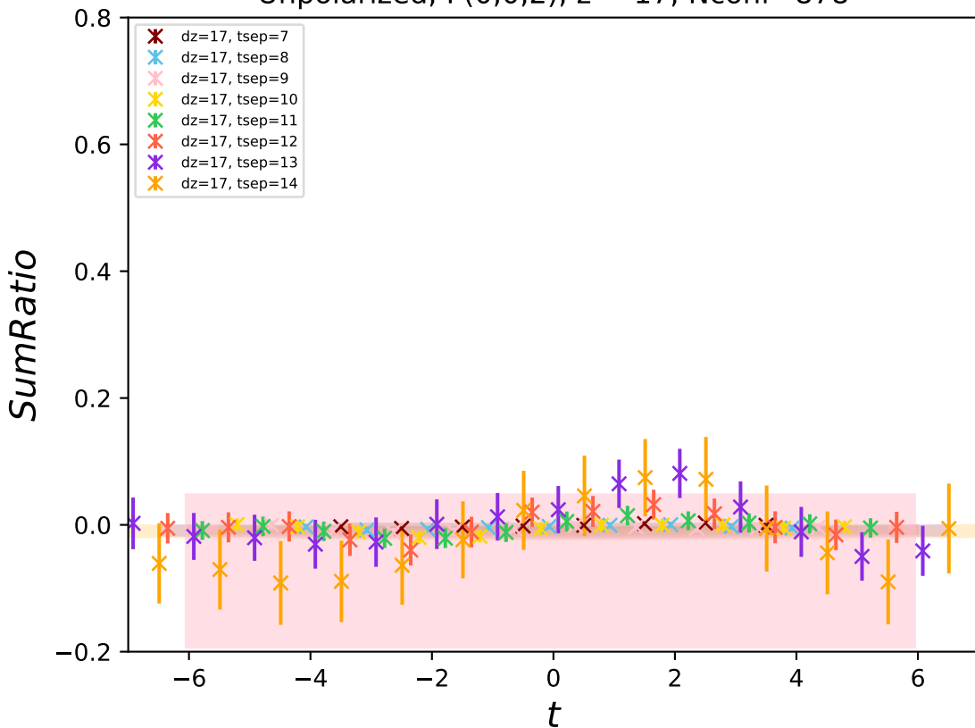
Unpolarized, P(0,0,2) , z = 17 , Nconf=878
