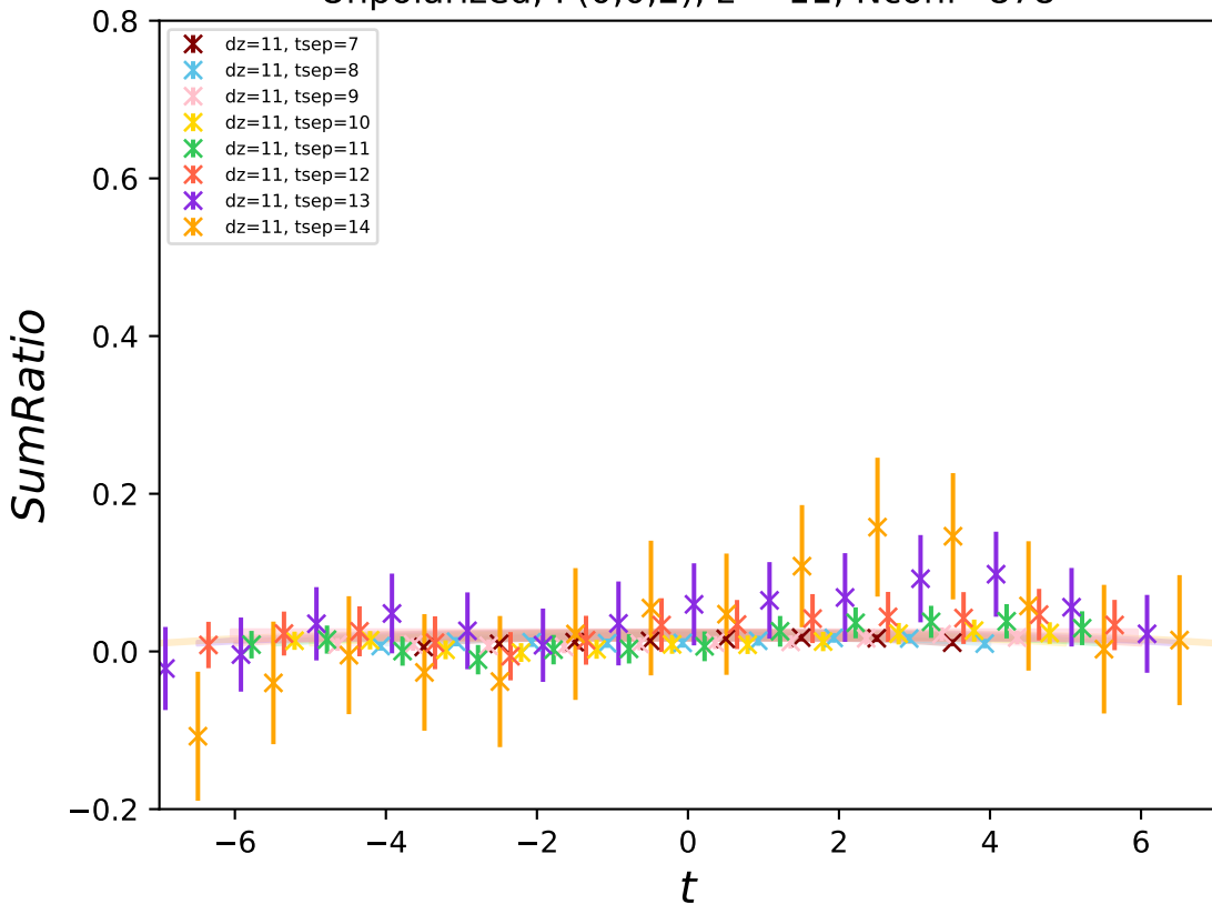
Unpolarized, P(0,0,2) , z = 11 , Nconf=878
