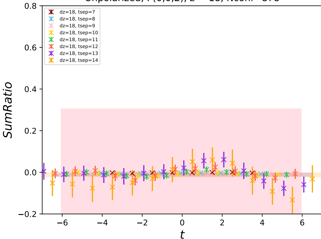
Unpolarized, P(0,0,2) , z = 18 , Nconf=878
