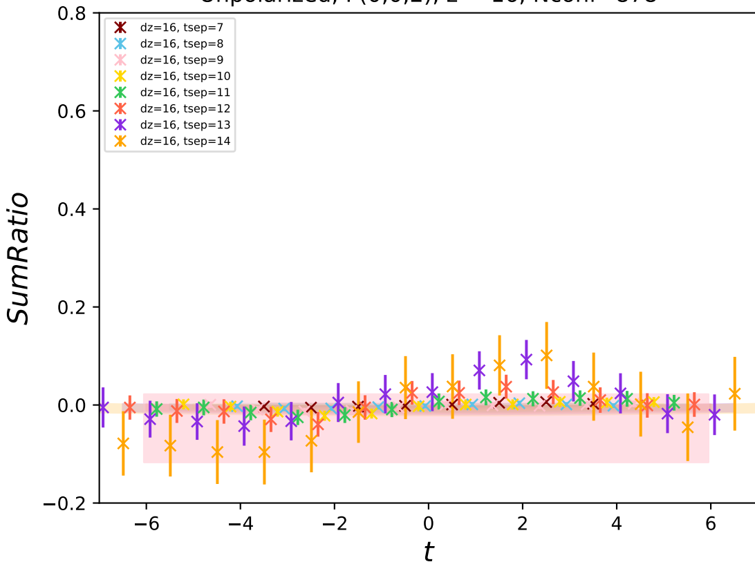
Unpolarized, P(0,0,2) , z = 16 , Nconf=878
