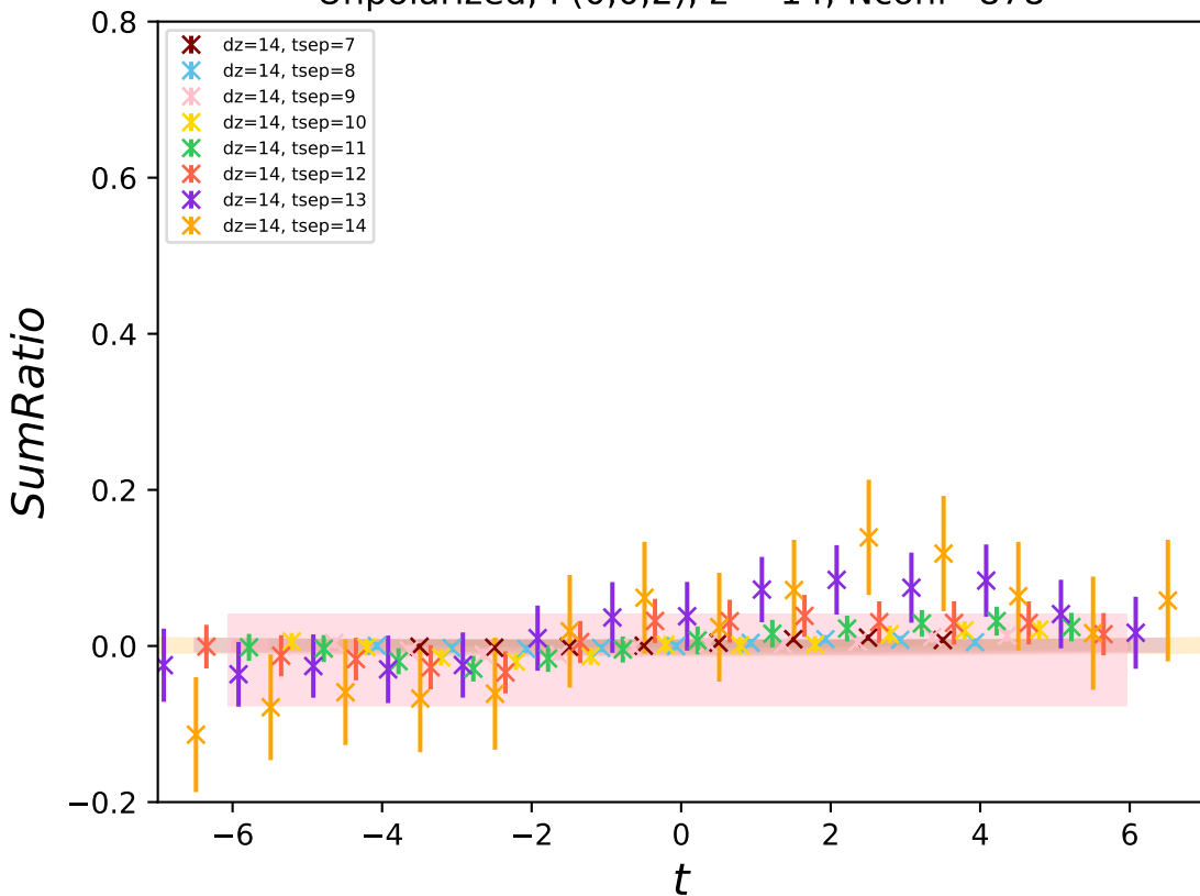
Unpolarized, P(0,0,2) , z = 14 , Nconf=878
