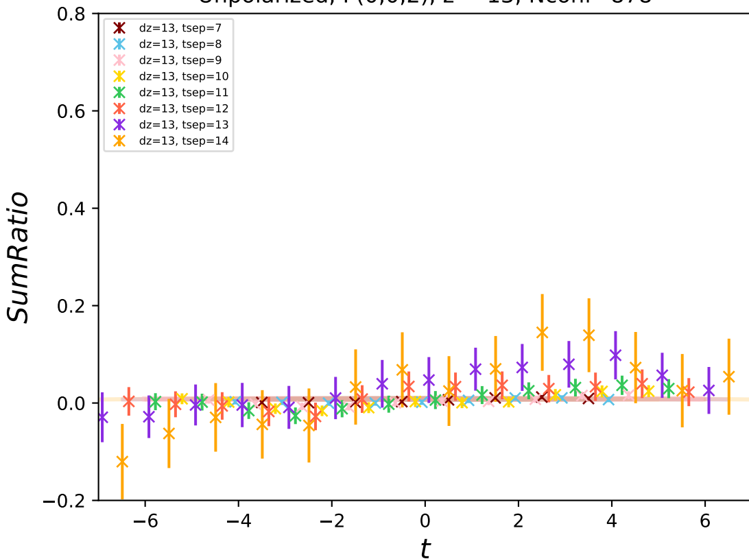
Unpolarized, P(0,0,2) , z = 13 , Nconf=878
