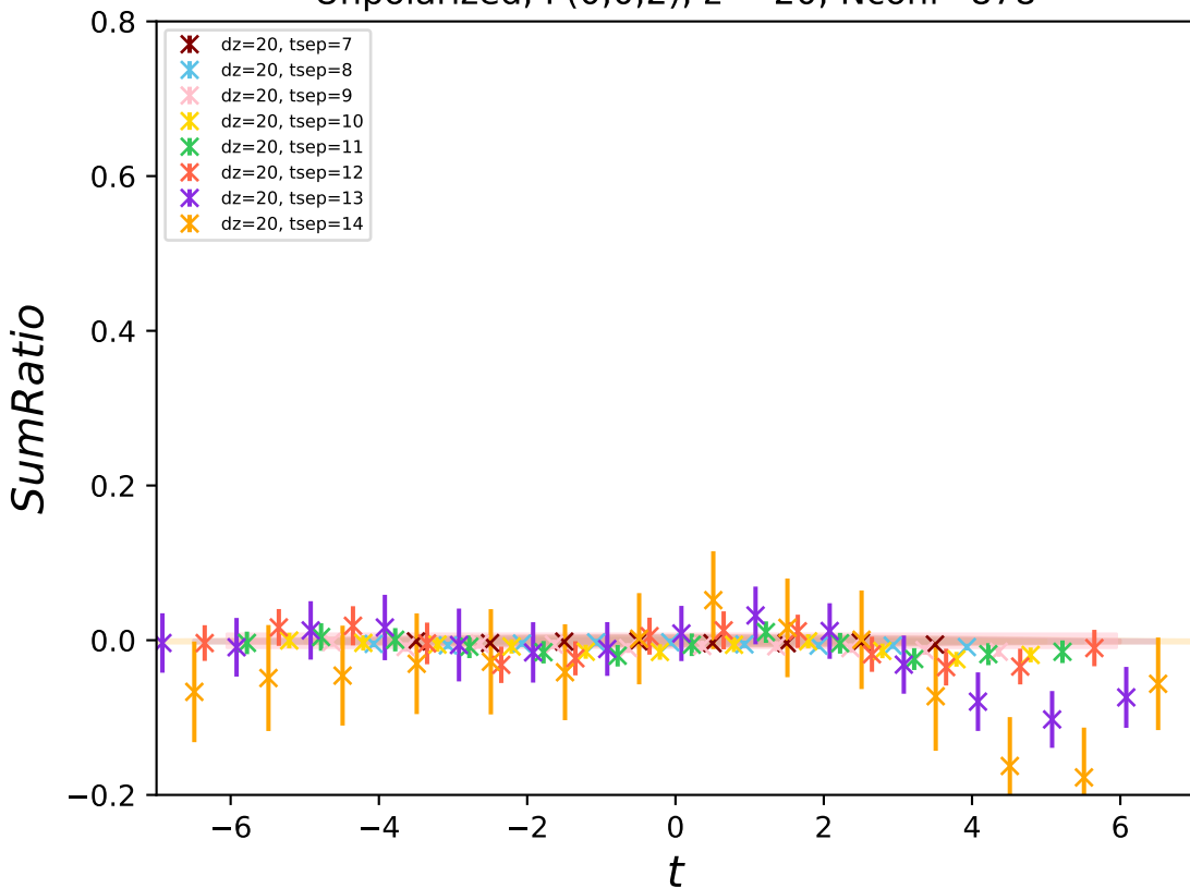
Unpolarized, P(0,0,2) , z = 20 , Nconf=878
