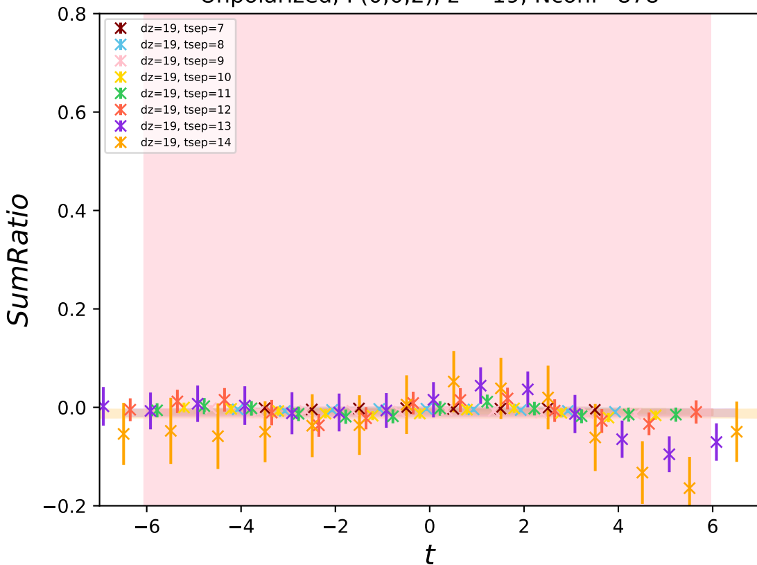
Unpolarized, P(0,0,2) , z = 19 , N_{\text{conf}}=878
