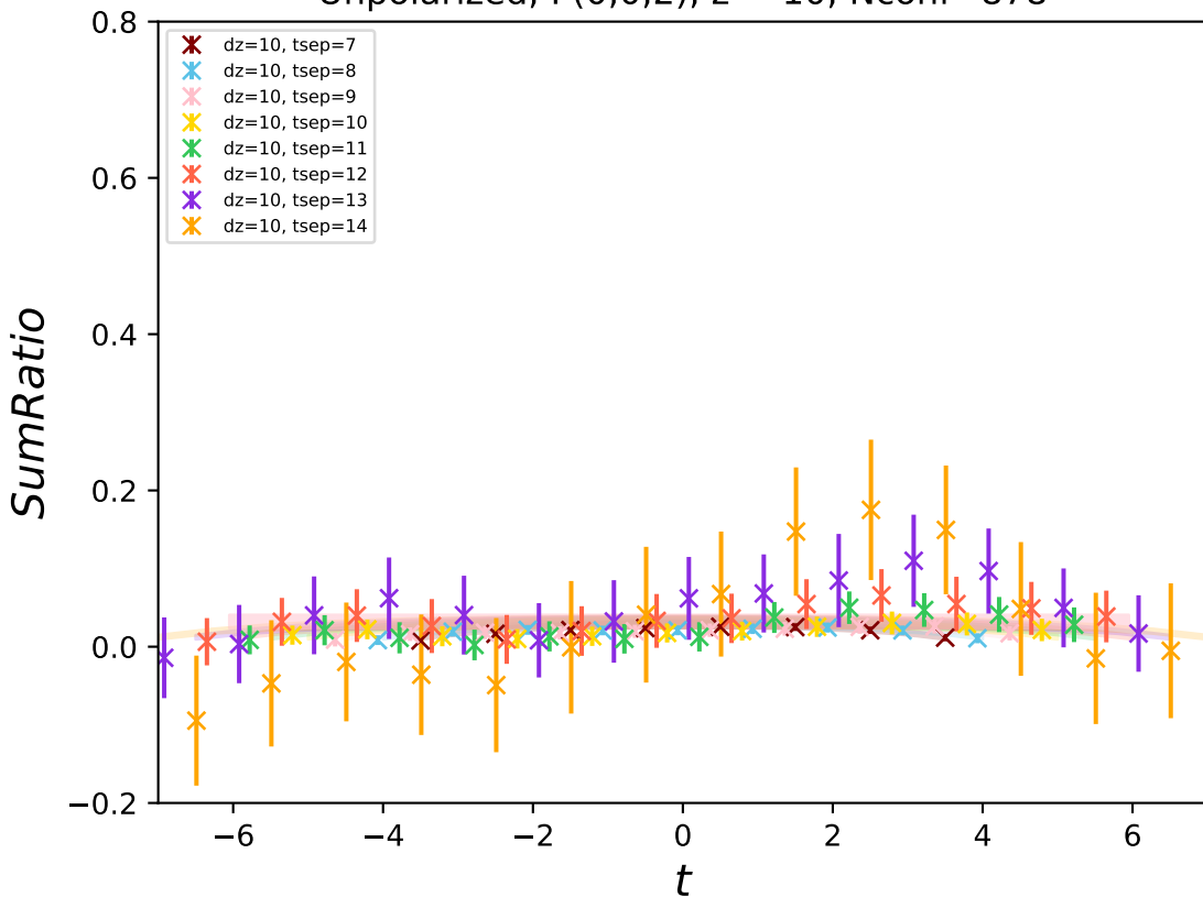
Unpolarized, P(0,0,2) , z = 10 , Nconf=878
