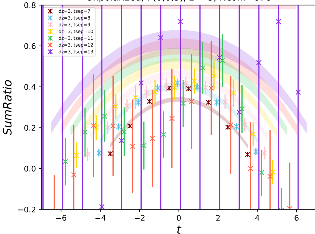
Unpolarized, P(0,0,3) , z = 3 , Nconf=878
