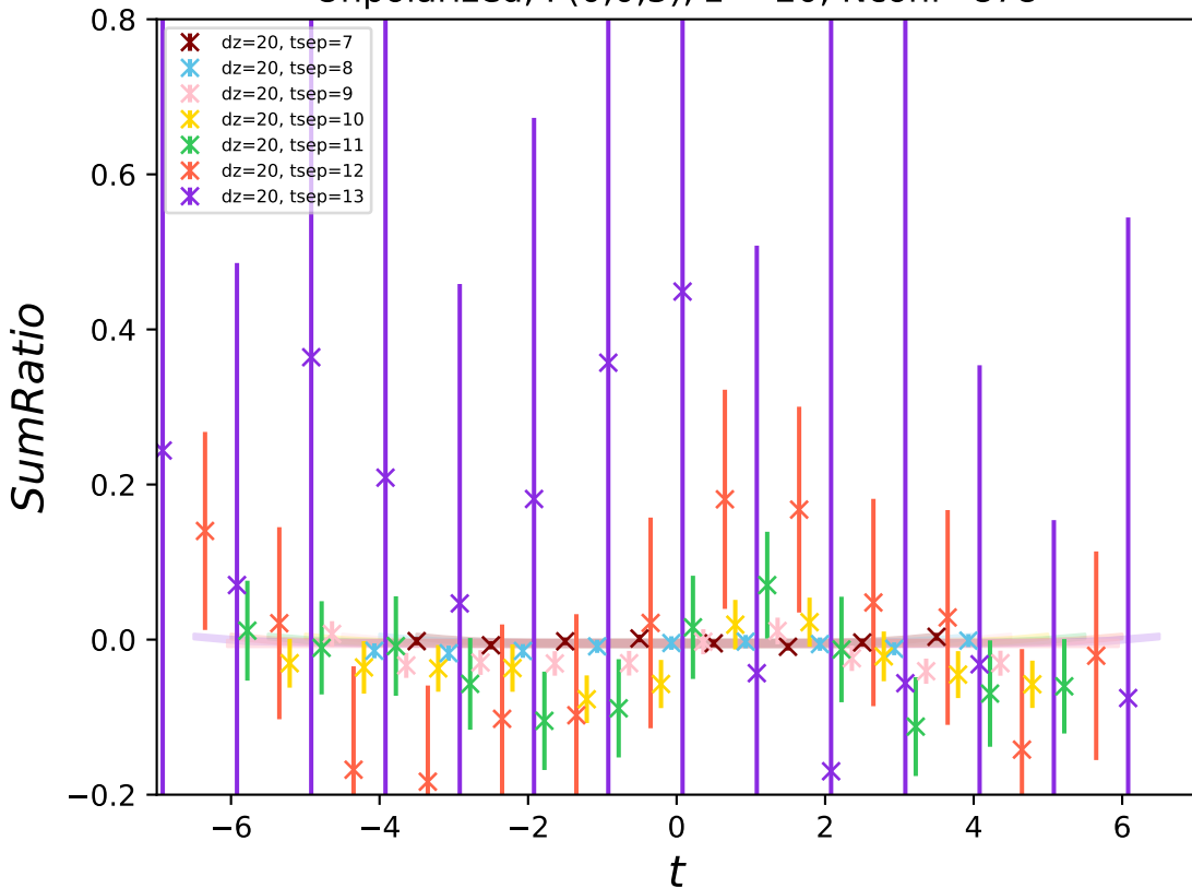
Unpolarized, P(0,0,3), z = 20 , Nconf=878
