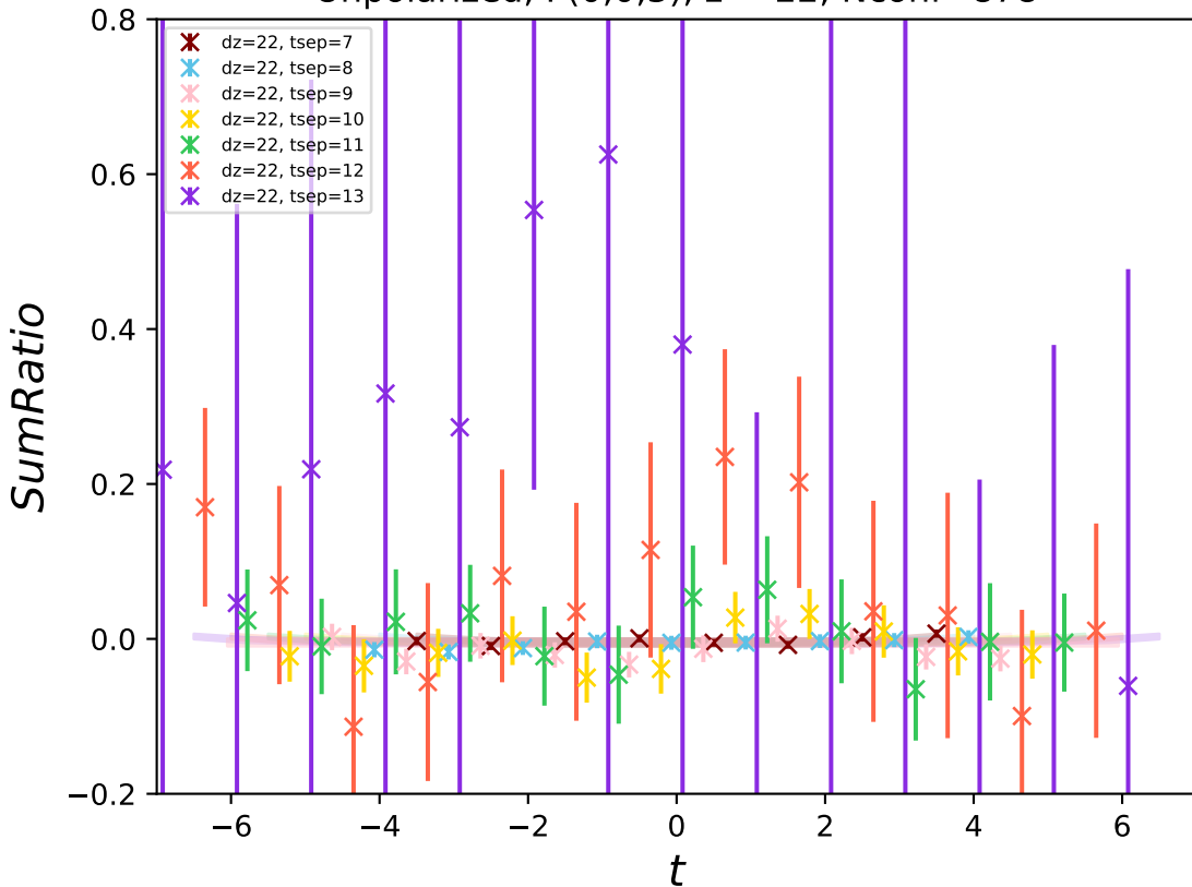
Unpolarized, P(0,0,3) , z = 22 , Nconf=878
