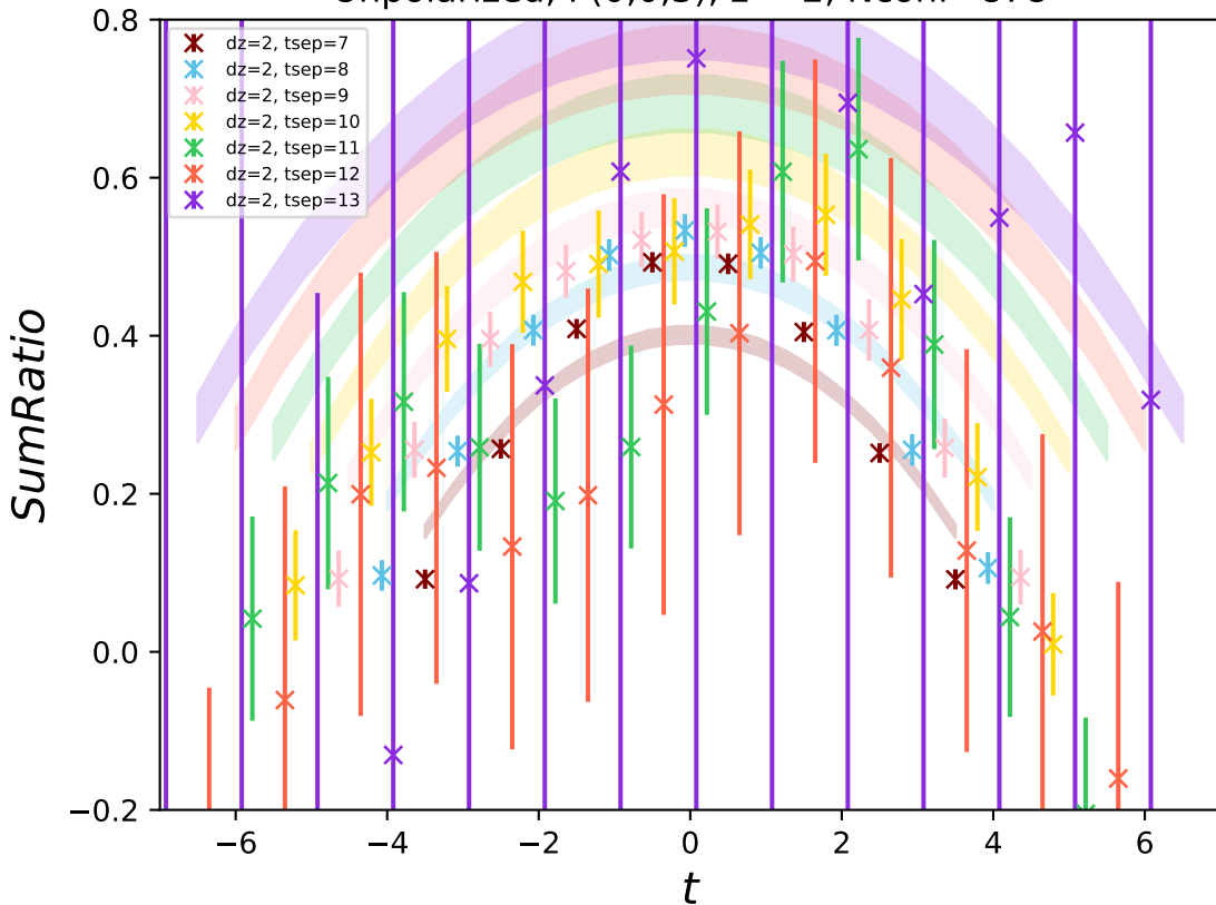
Unpolarized, P(0,0,3) , z = 2 , N_{\text{conf}}=878
