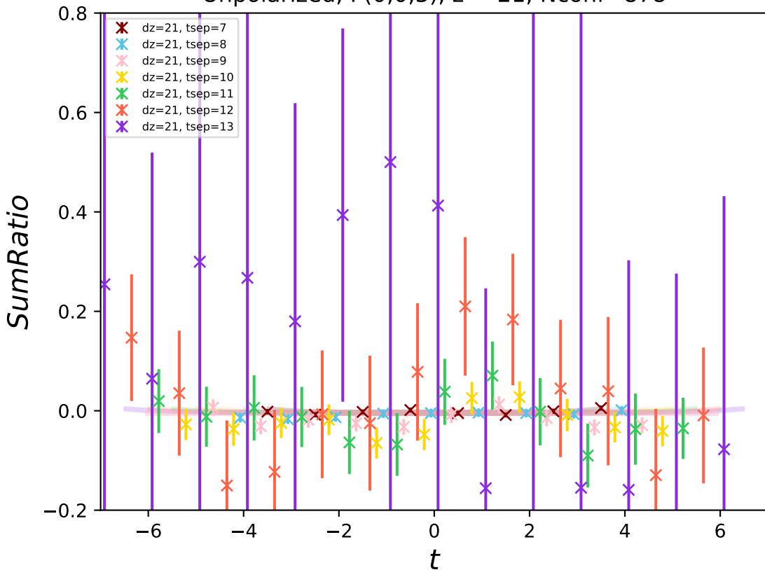
Unpolarized, P(0,0,3) , z = 21 , Nconf=878
