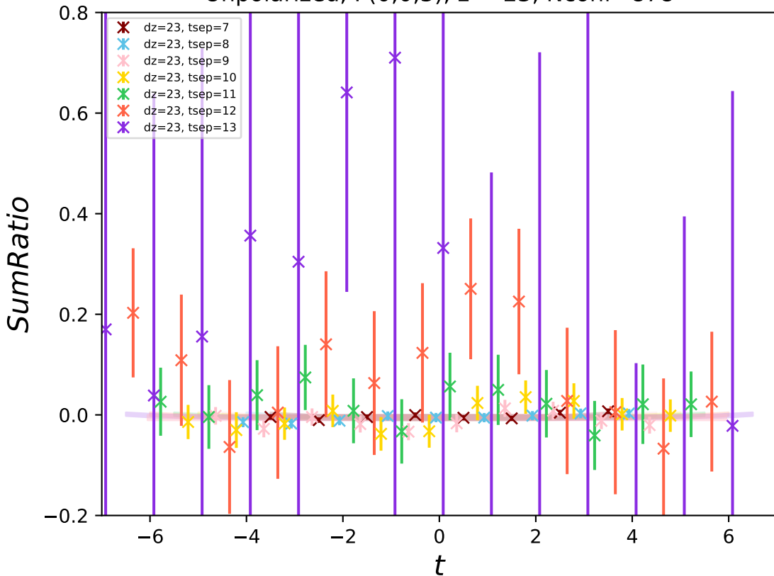
Unpolarized, P(0,0,3) , z = 23 , Nconf=878
