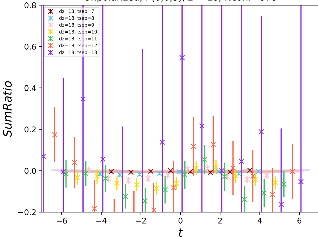
Unpolarized, P(0,0,3), z = 18 , Nconf=878
