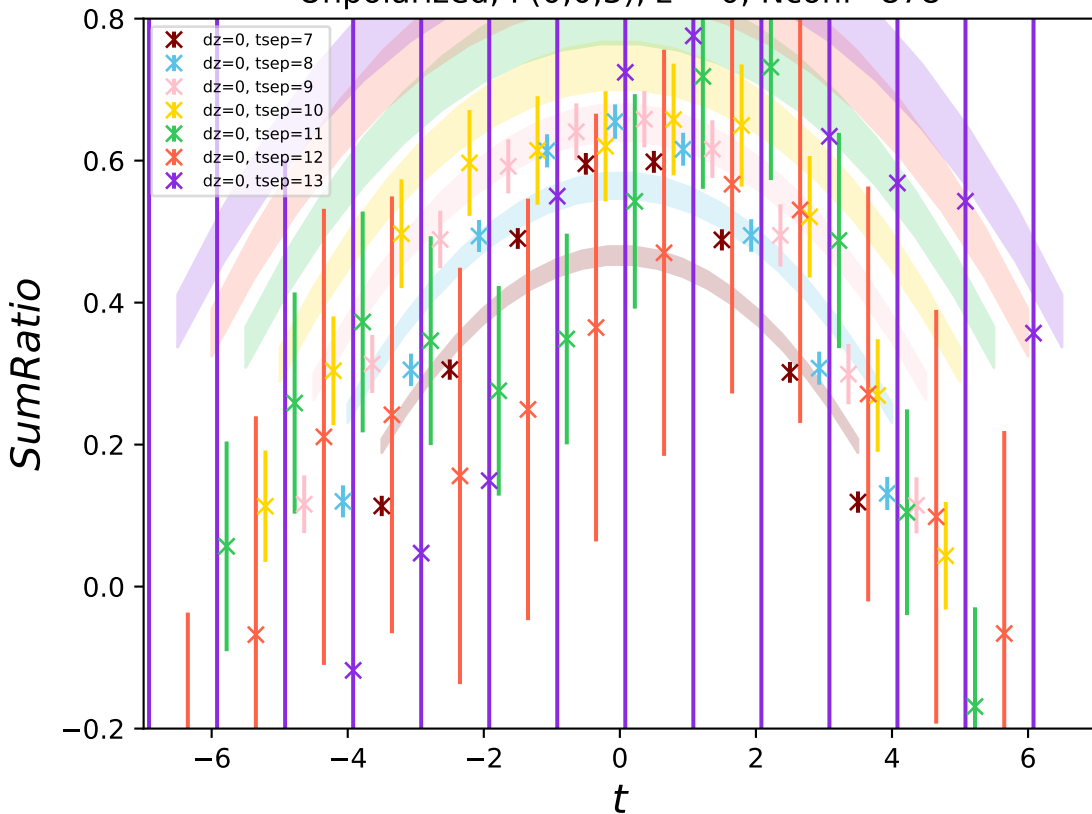
Unpolarized, P(0,0,3) , z = 0 , N_{\text{conf}}=878
