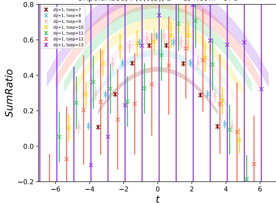
Unpolarized, P(0,0,3) , z = 1 , Nconf=878
