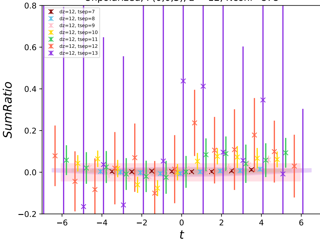
Unpolarized, P(0,0,3) , z = 12 , N_{\text{conf}}=878
