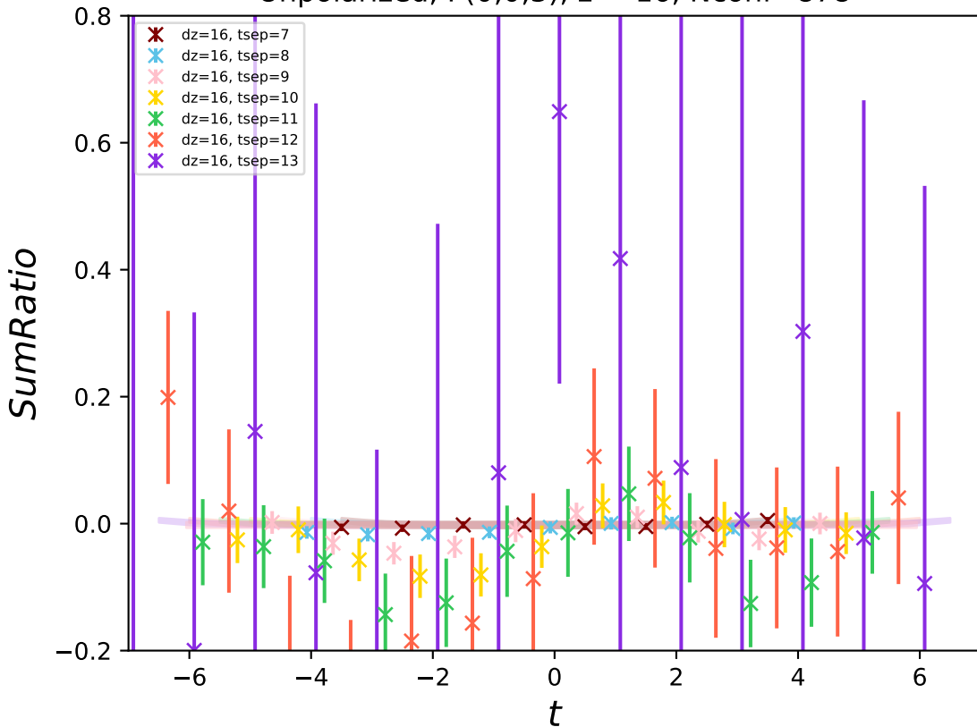
Unpolarized, P(0,0,3) , z = 16 , N_{\text{conf}}=878
