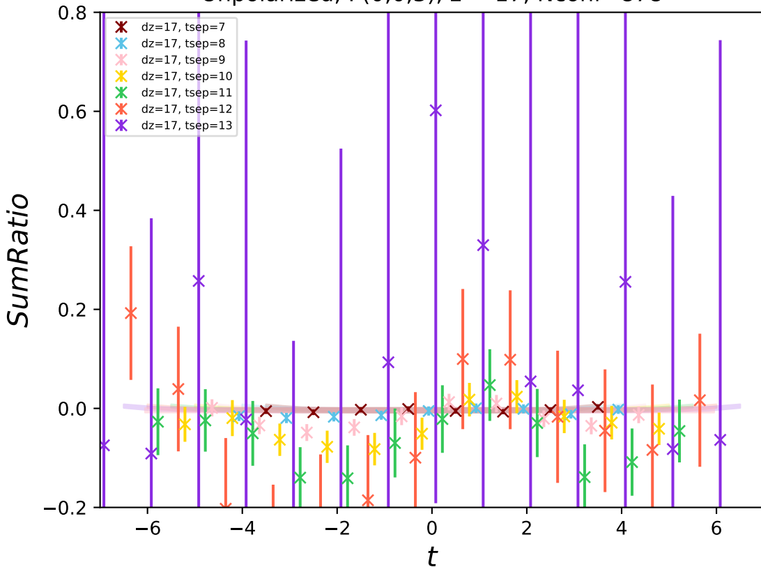
Unpolarized, P(0,0,3) , z = 17 , Nconf=878
