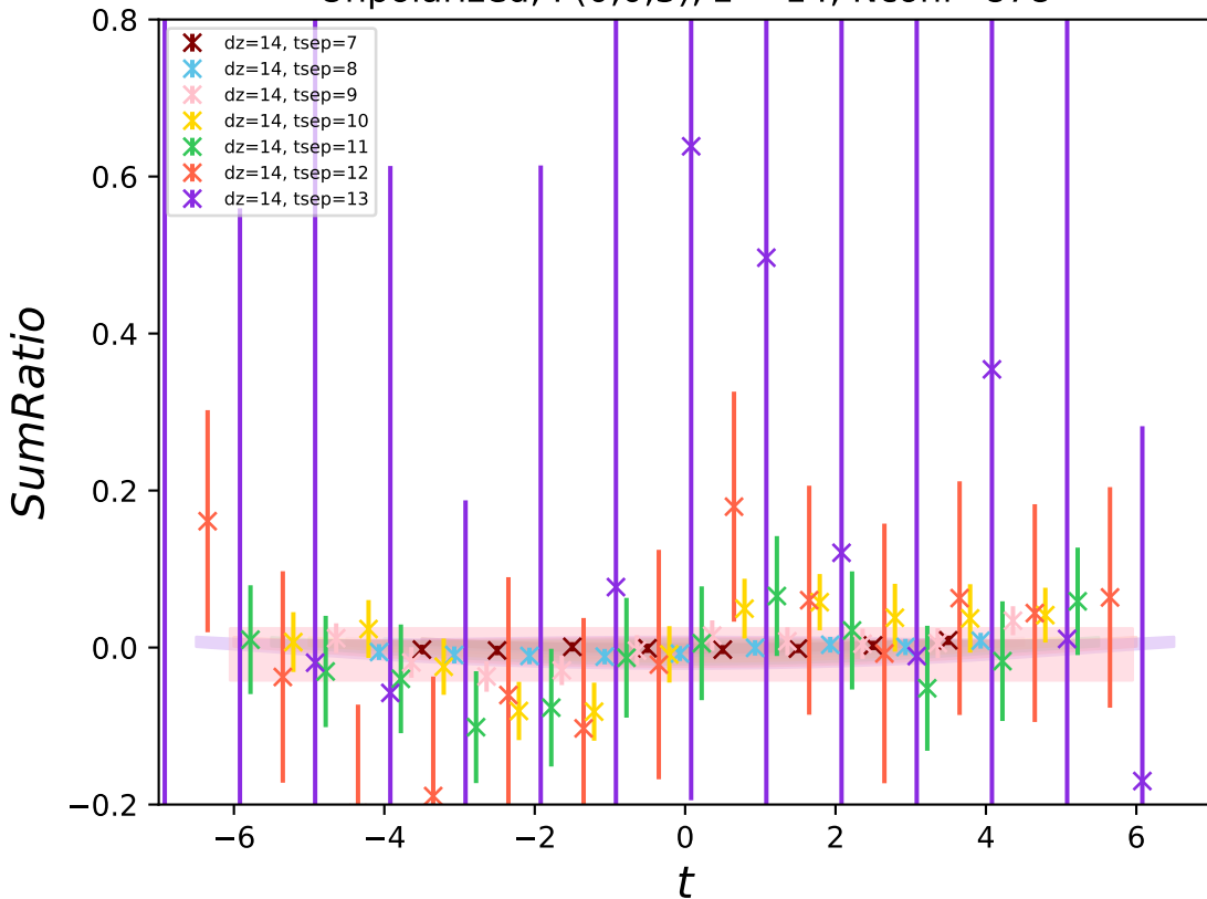
Unpolarized, P(0,0,3) , z = 14 , N_{\text{conf}}=878
