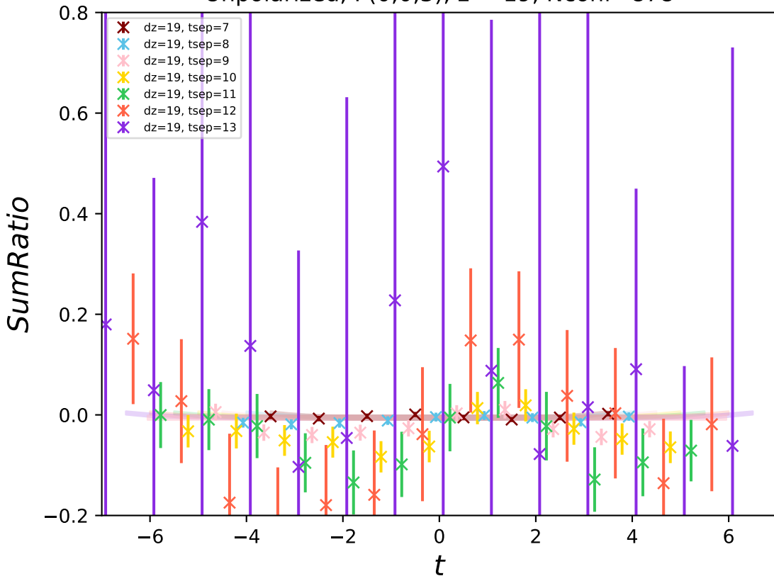
Unpolarized, P(0,0,3) , z = 19 , N_{\text{conf}}=878
