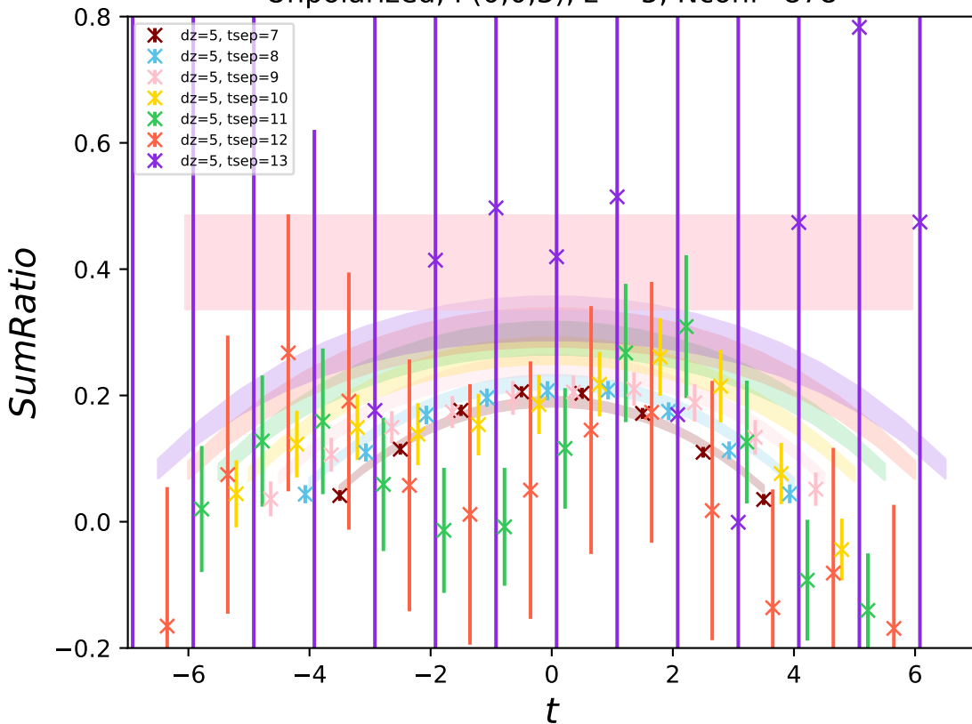
Unpolarized, P(0,0,3) , z = 5 , Nconf=878
