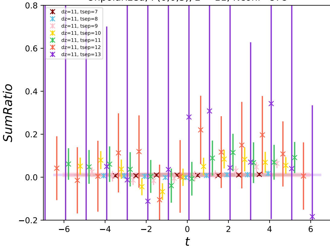
Unpolarized, P(0,0,3) , z = 11 , N_{\text{conf}}=878
