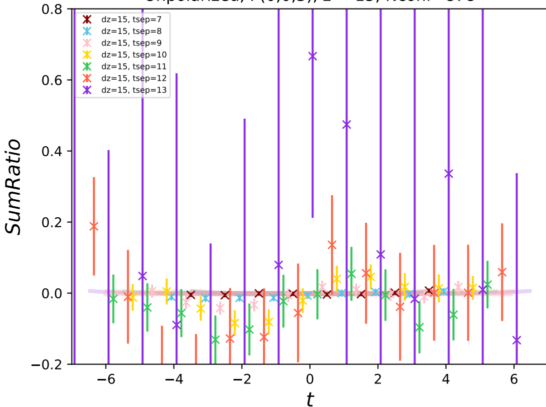
Unpolarized, P(0,0,3) , z = 15 , N_{\text{conf}}=878
