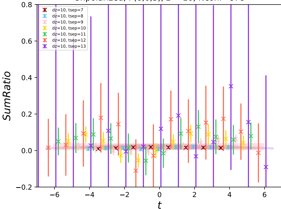
Unpolarized, P(0,0,3) , z = 10 , N_{\text{conf}}=878
