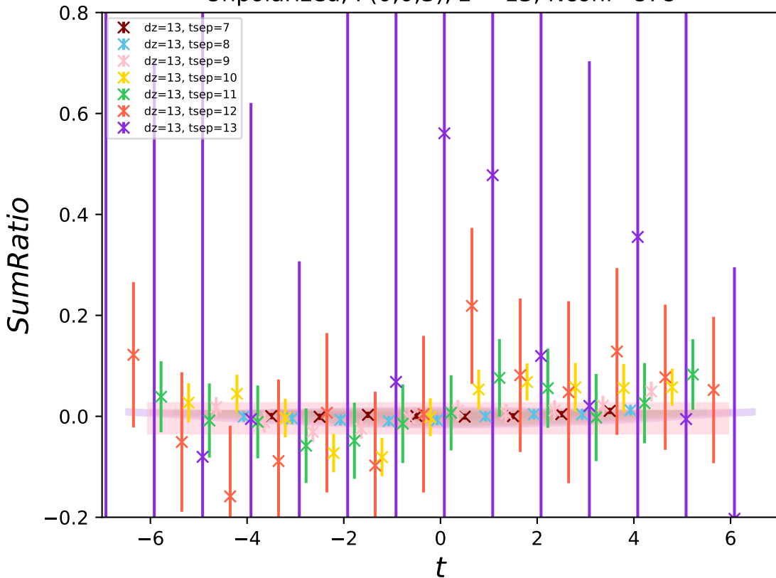
Unpolarized, P(0,0,3) , z = 13 , Nconf=878
