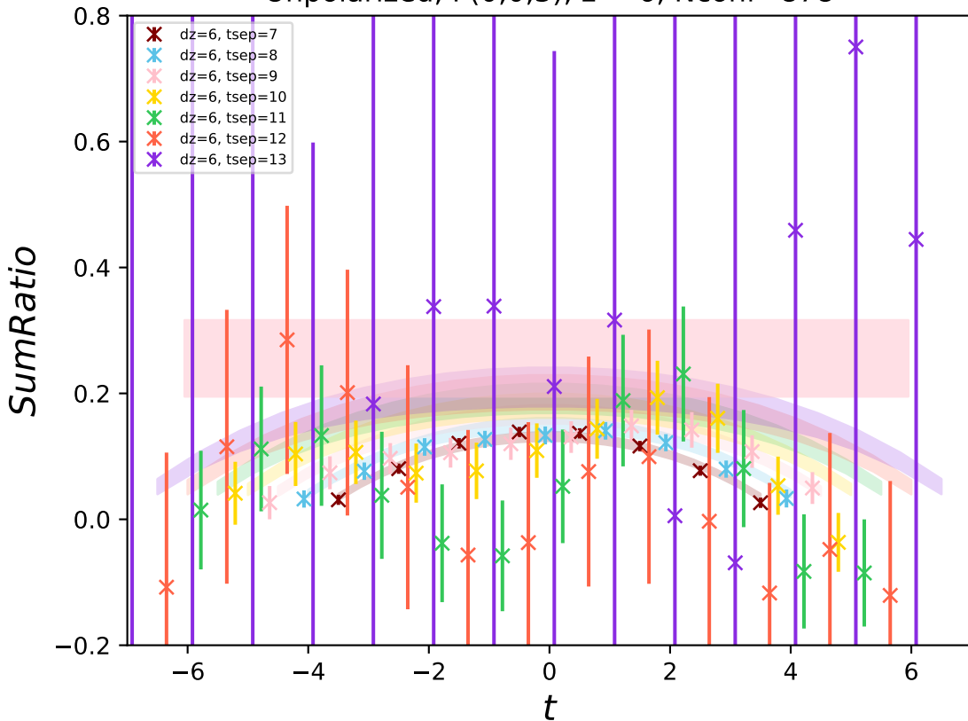
Unpolarized, P(0,0,3) , z = 6 , Nconf=878
