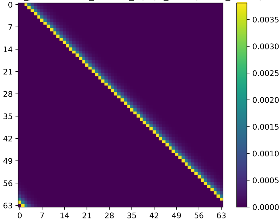
Real Part of two_point/L32x64_C32P23_Cg5g4_Pix0Piy0Piz2_Pfx0Pfy0Pfz2
