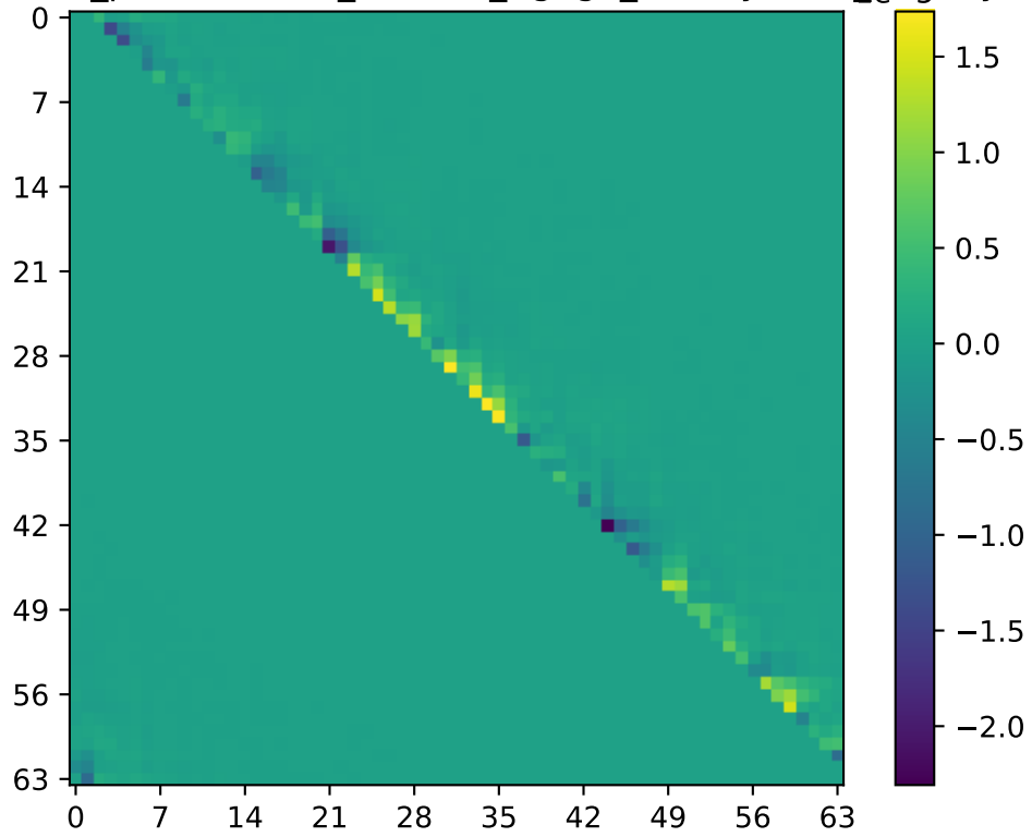
Real Part of two_point/L32x64_C32P23_Cg5g4_Pix0Piy0Piz2_1eL5_Pfx1Pfy1Pfx2
