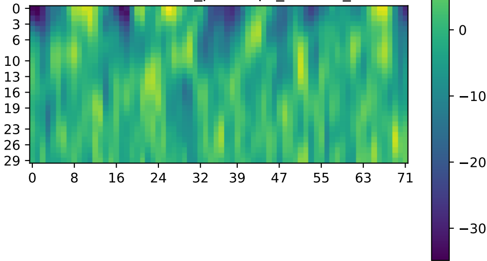
Real Part of two_point/ops_L24x72_cc
