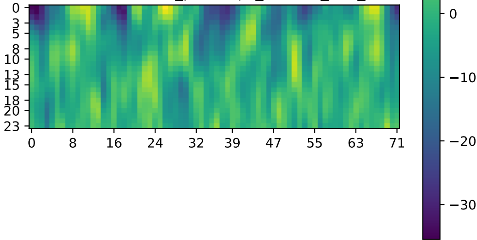
Real Part of two_point/ops_L24x72_dhx_ti
