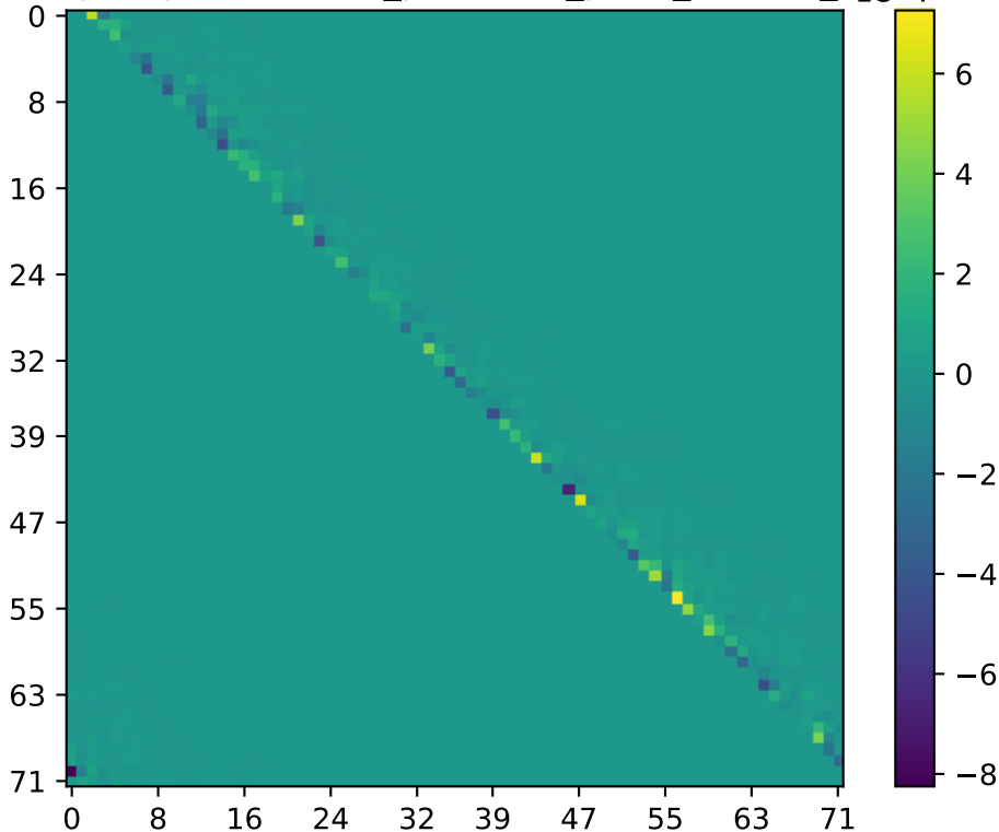
Imaginary Part of two_point/two_point_L24x72_dhx_7
