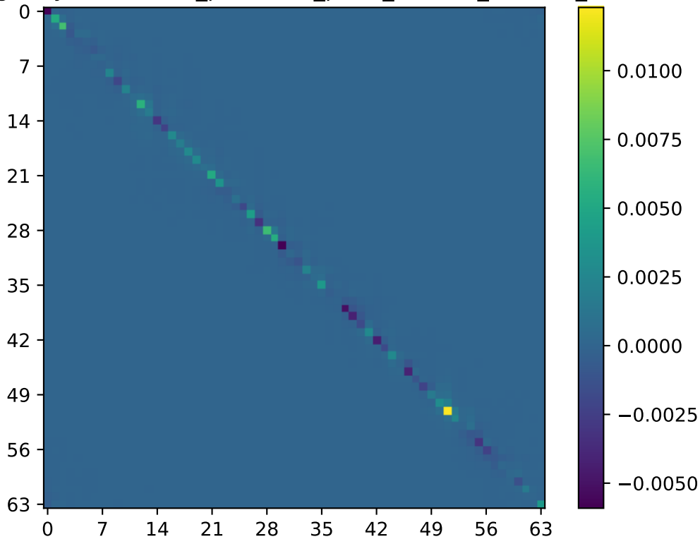
Imaginary Part of two_point/two_point_L32x64_C32P23_GPD
