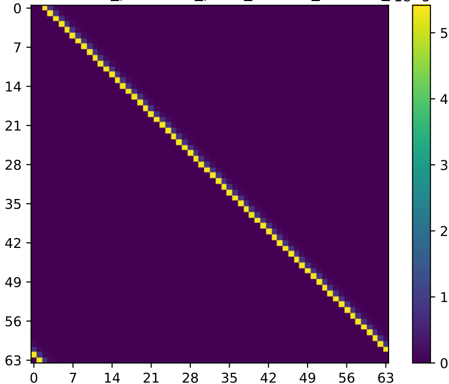
Real Part of two_point/two_point_L32x64_C32P23_mean
