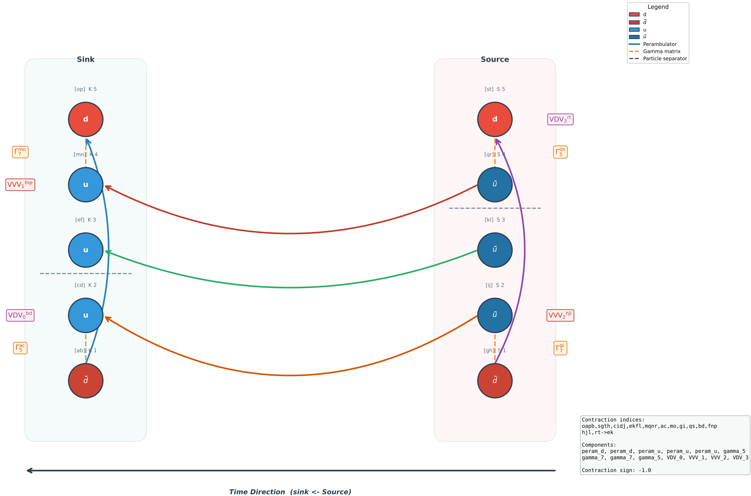
Wick Contraction Diagram #0 (2pt, sign = -1.0)
