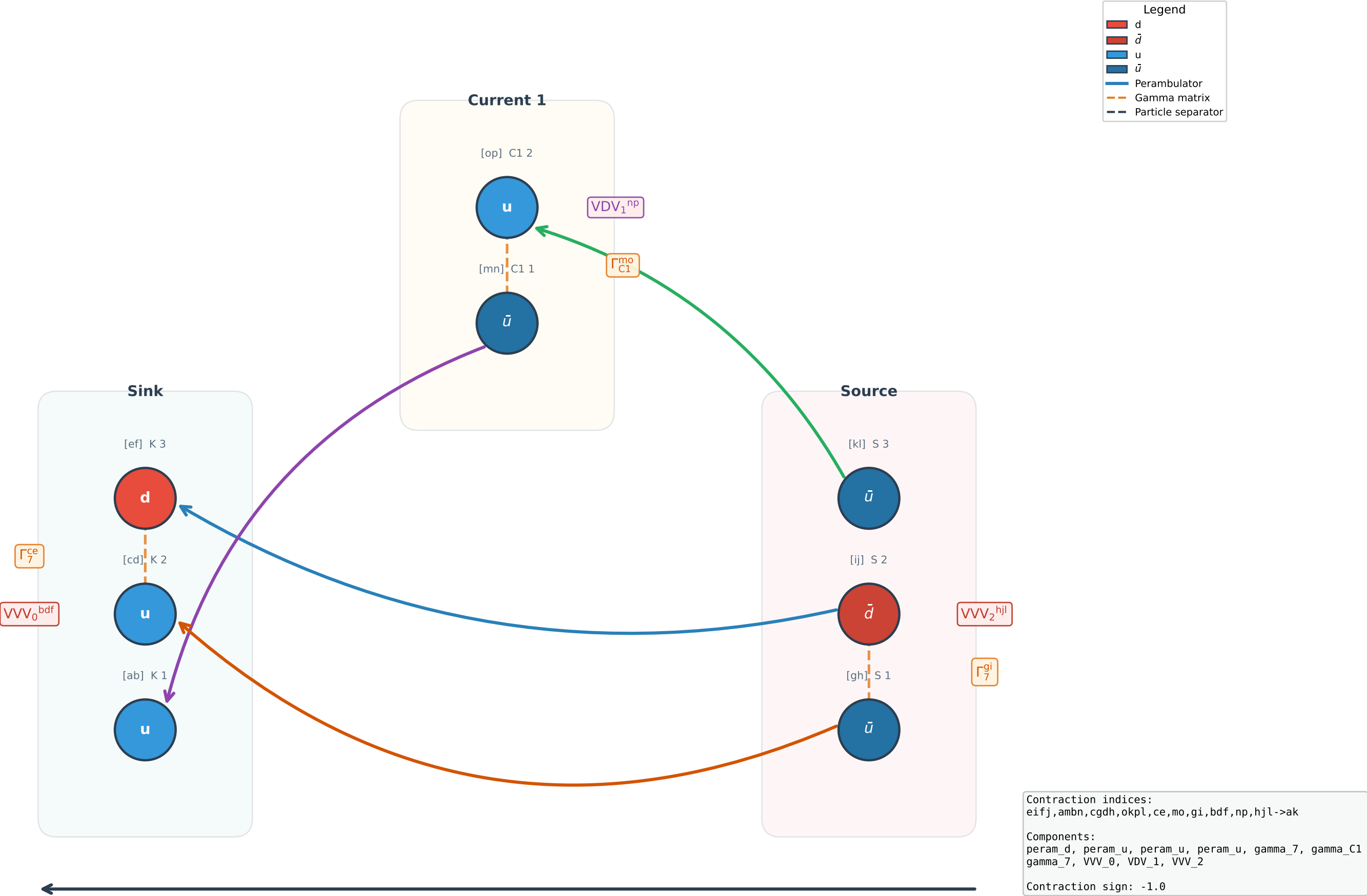
Wick Contraction Diagram #0 (3pt, sign = -1.0)
