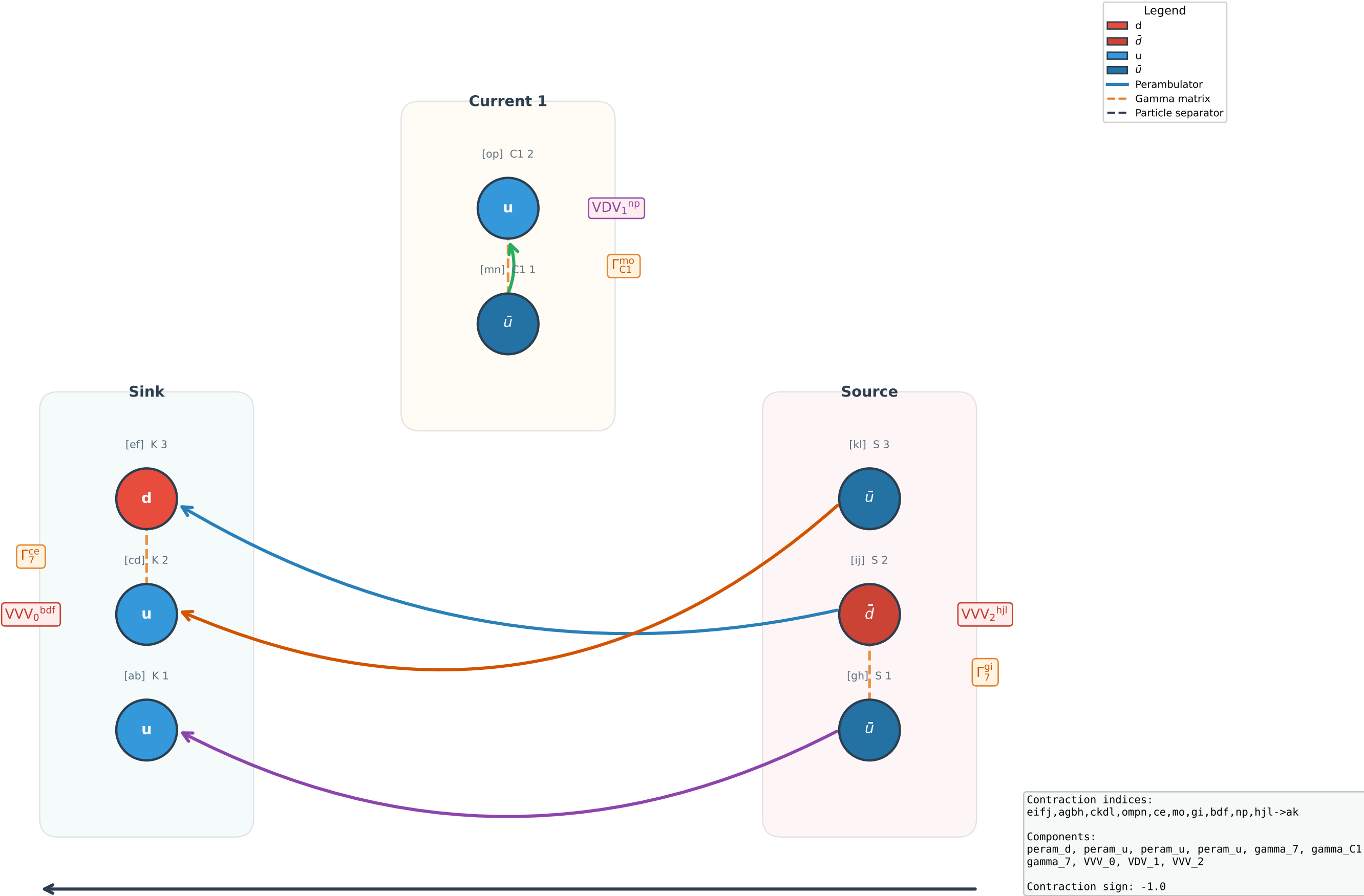
Wick Contraction Diagram #3 (3pt, sign = -1.0)
