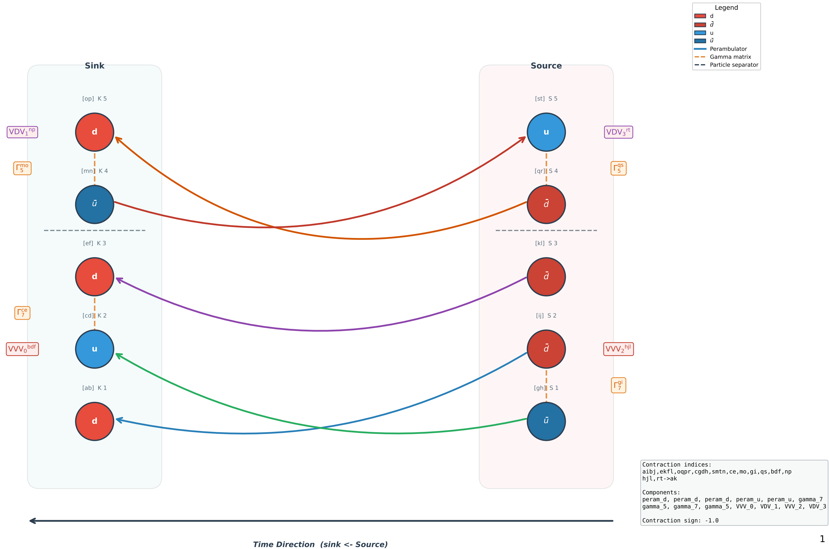
Wick Contraction Diagram #1 (2pt, sign = -1.0)
