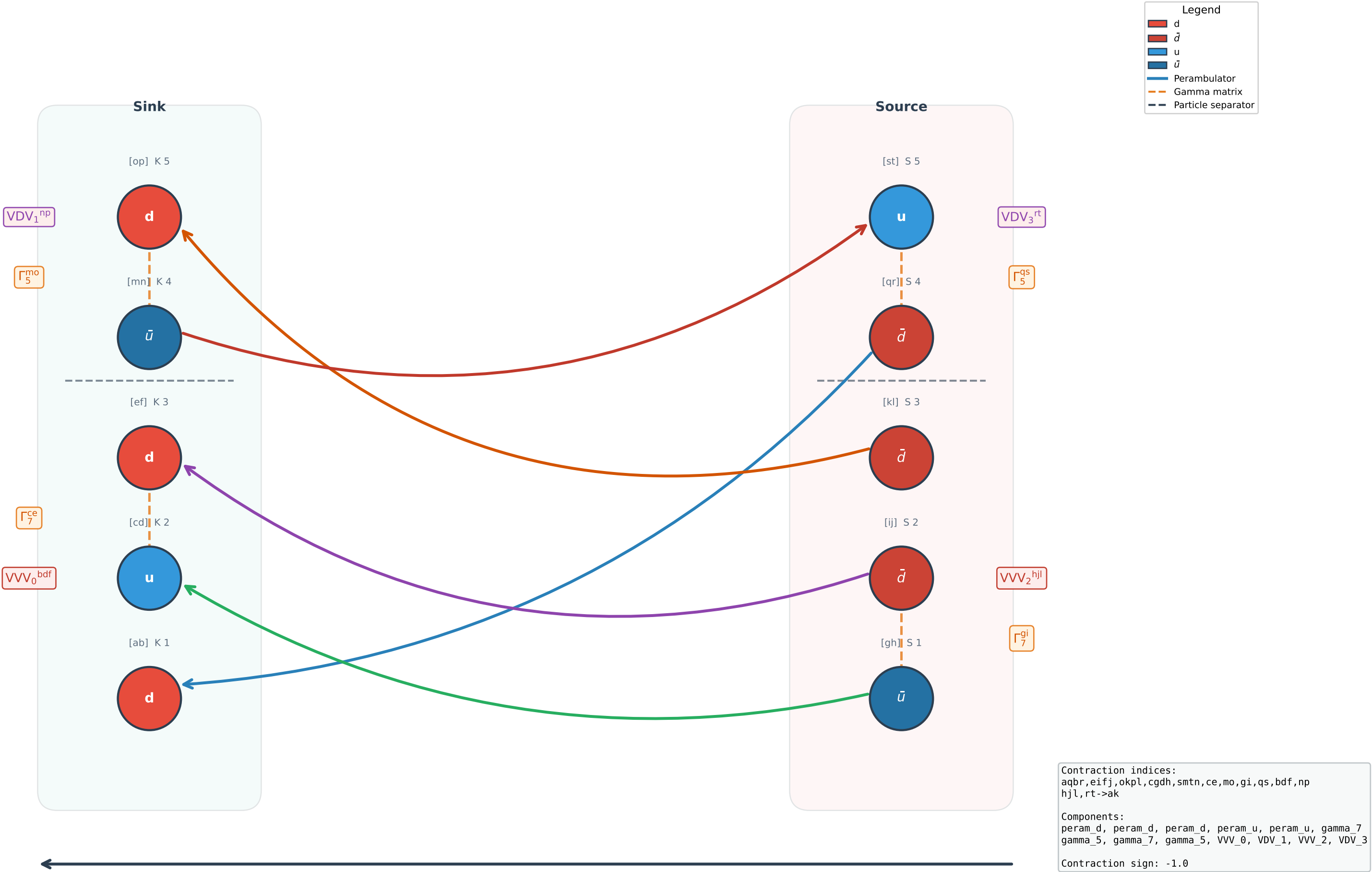
Wick Contraction Diagram #9 (2pt, sign = -1.0)
