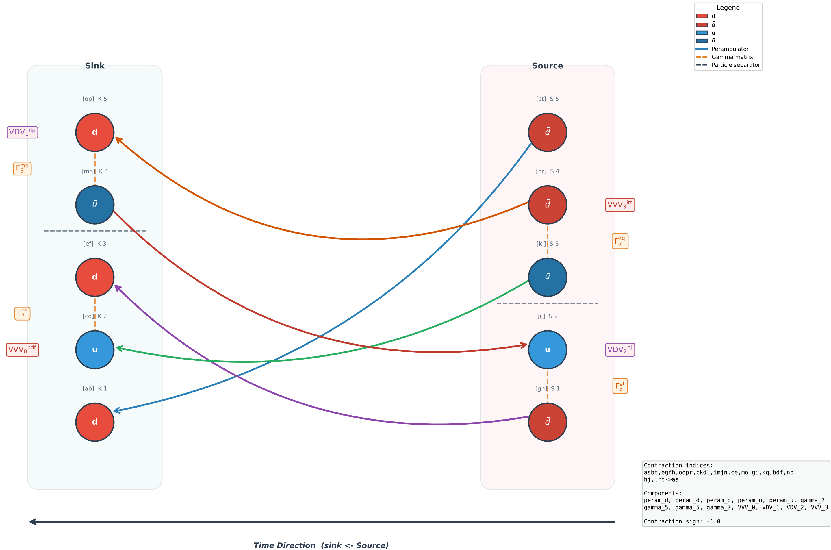
Wick Contraction Diagram #9 (2pt, sign = -1.0)
