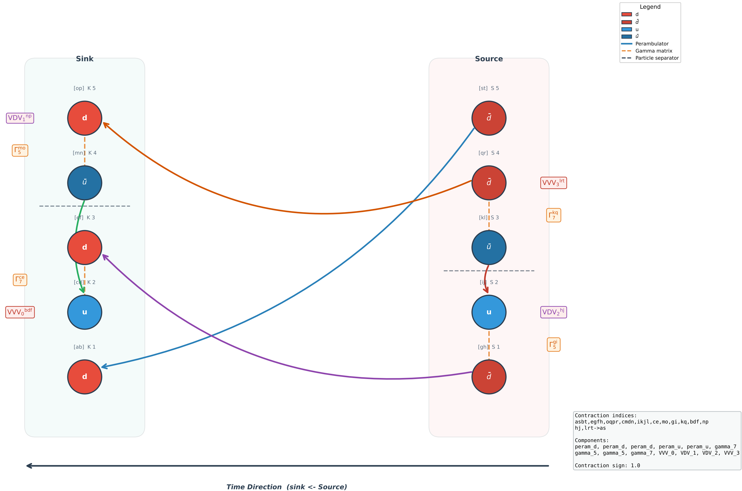
Wick Contraction Diagram #8 (2pt, sign = 1.0)
