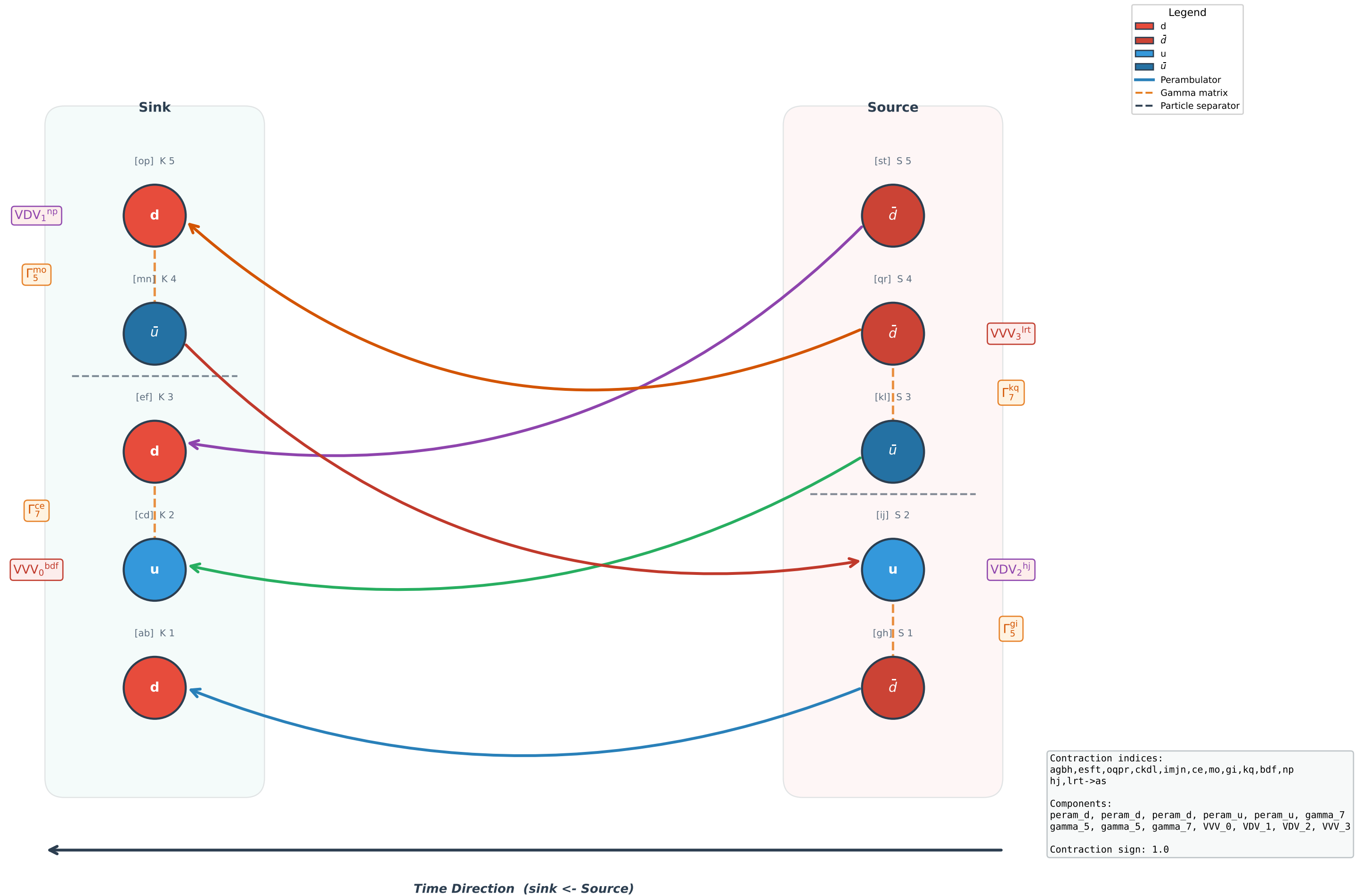
Wick Contraction Diagram #3 (2pt, sign = 1.0)
