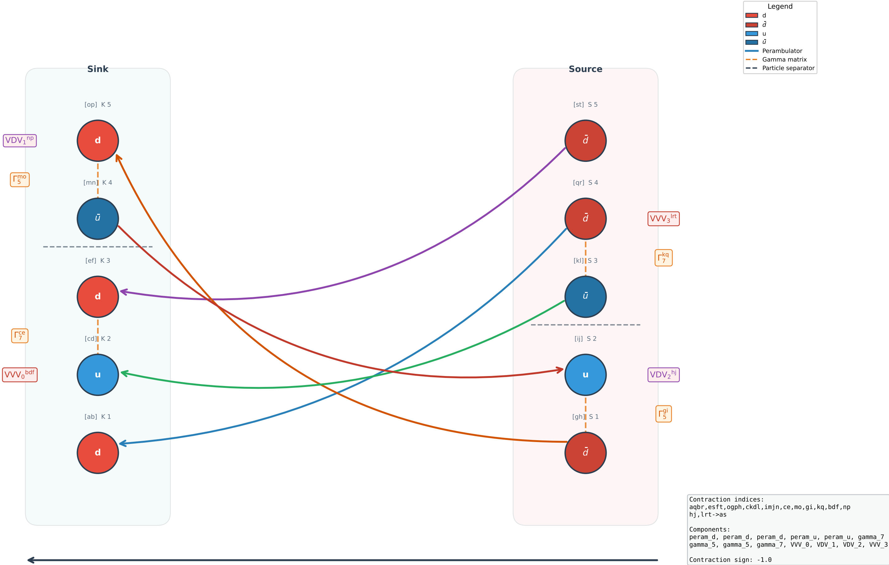
Wick Contraction Diagram #7 (2pt, sign = -1.0)
