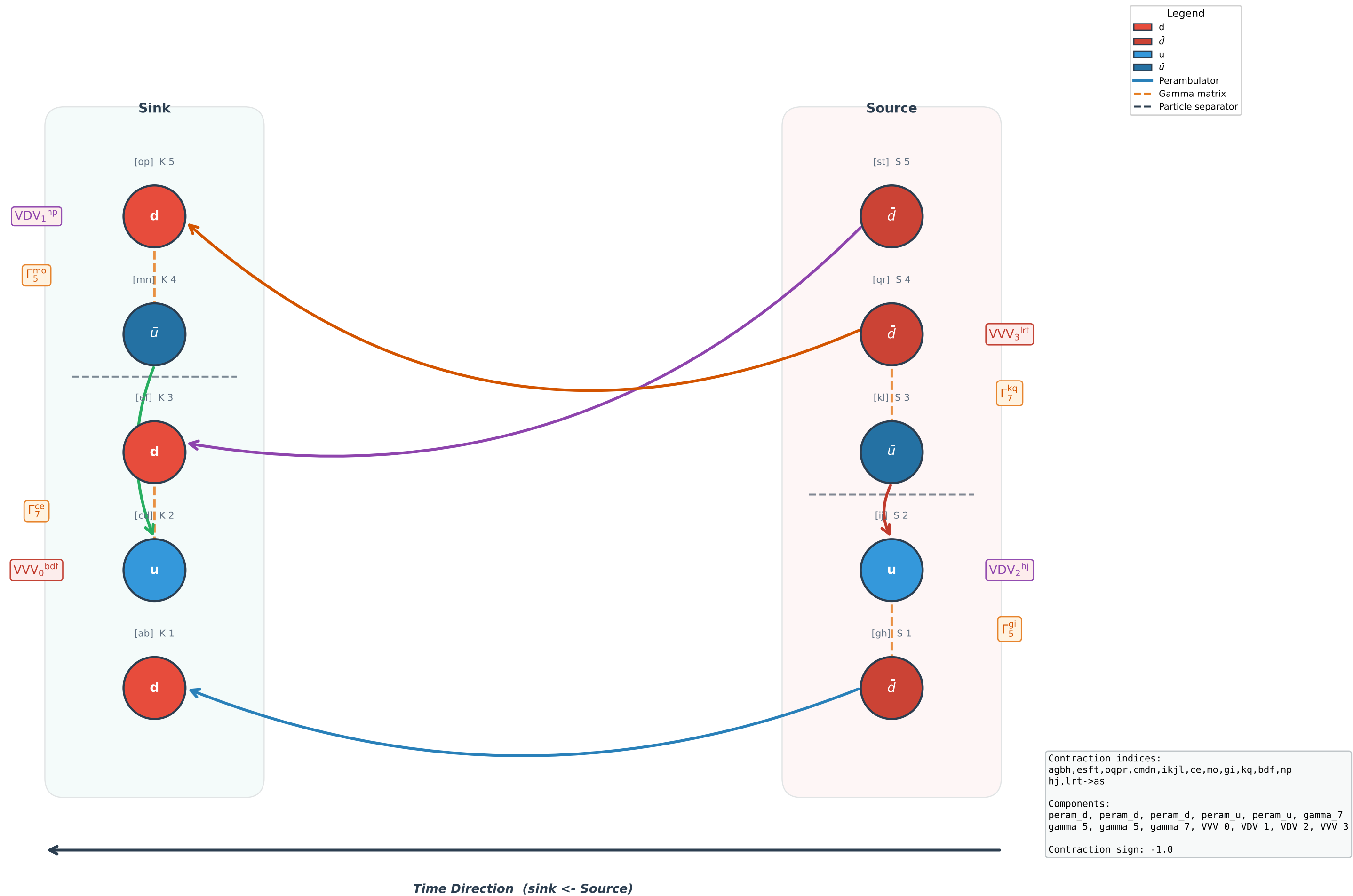
Wick Contraction Diagram #2 (2pt, sign = -1.0)
