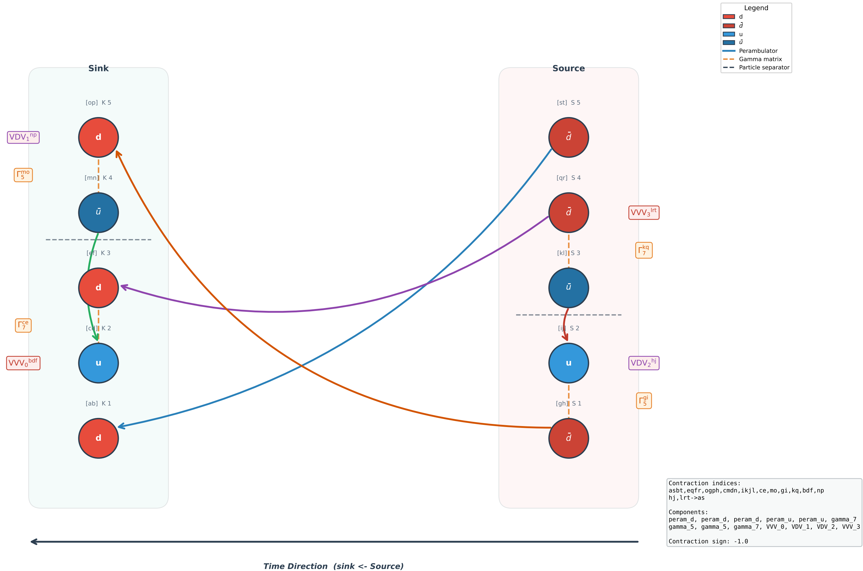
Wick Contraction Diagram #10 (2pt, sign = -1.0)
