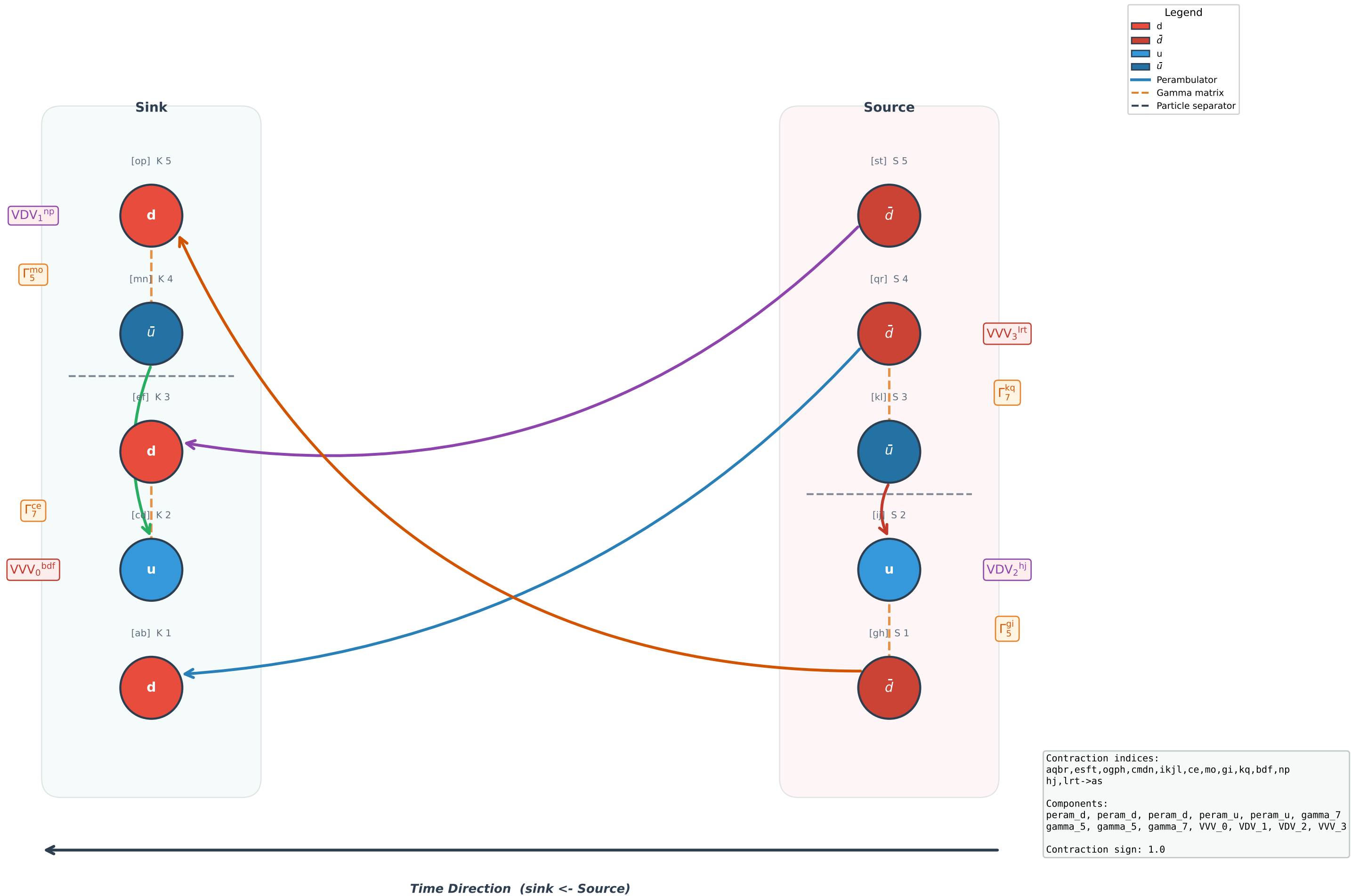
Wick Contraction Diagram #6 (2pt, sign = 1.0)
