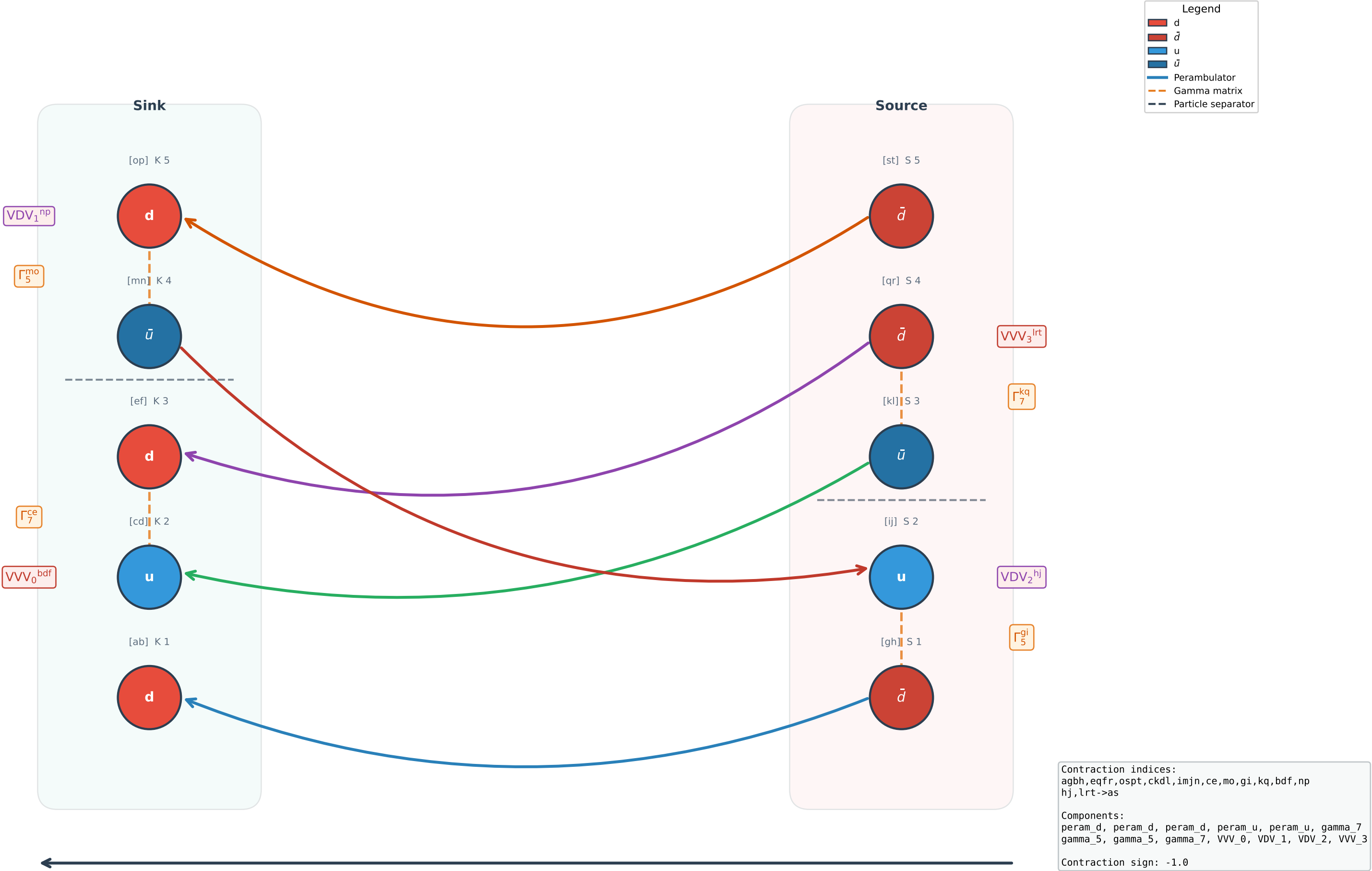
Wick Contraction Diagram #1 (2pt, sign = -1.0)
