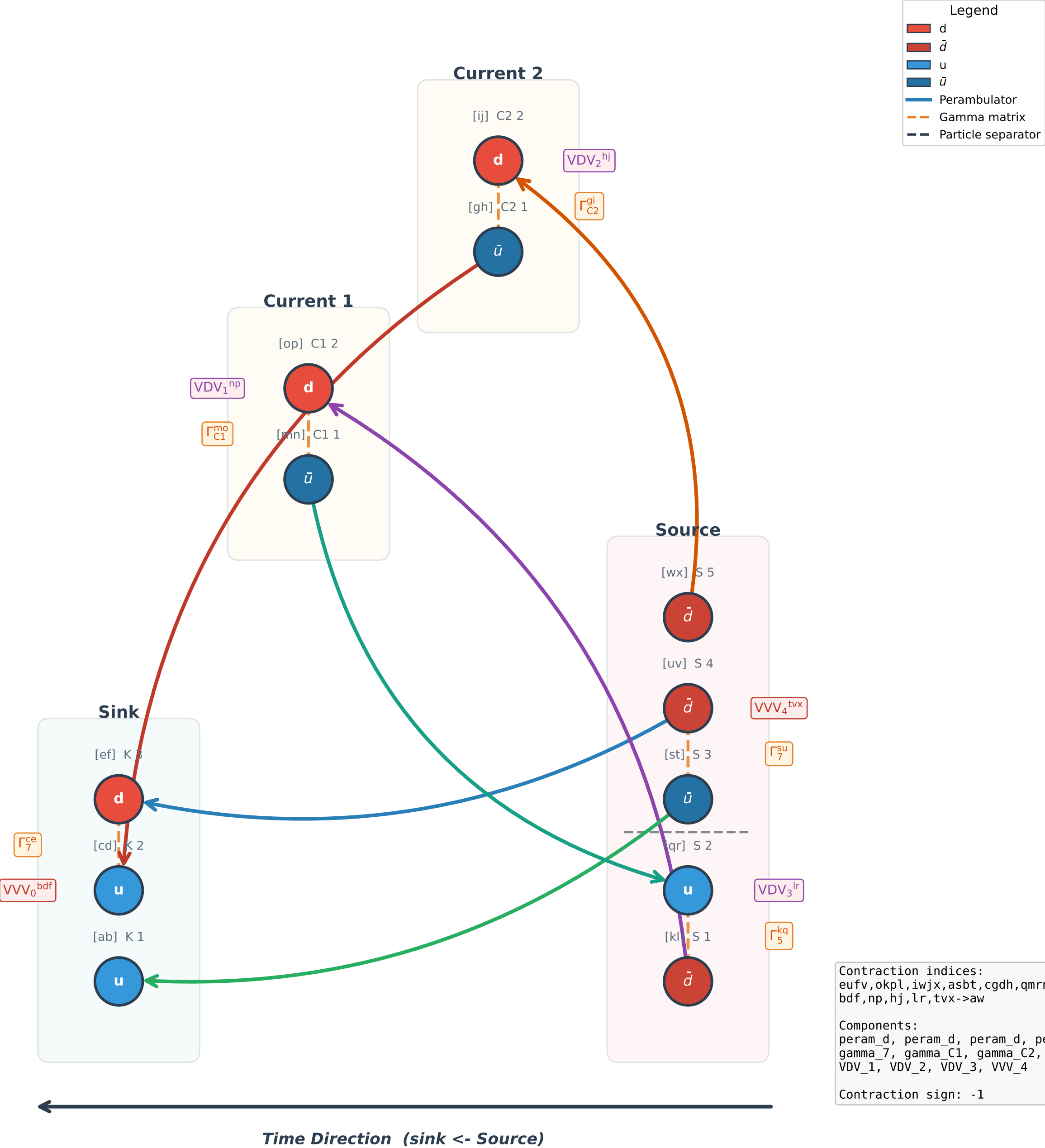
Wick Contraction Diagram #18 (3pt, sign = -1)
