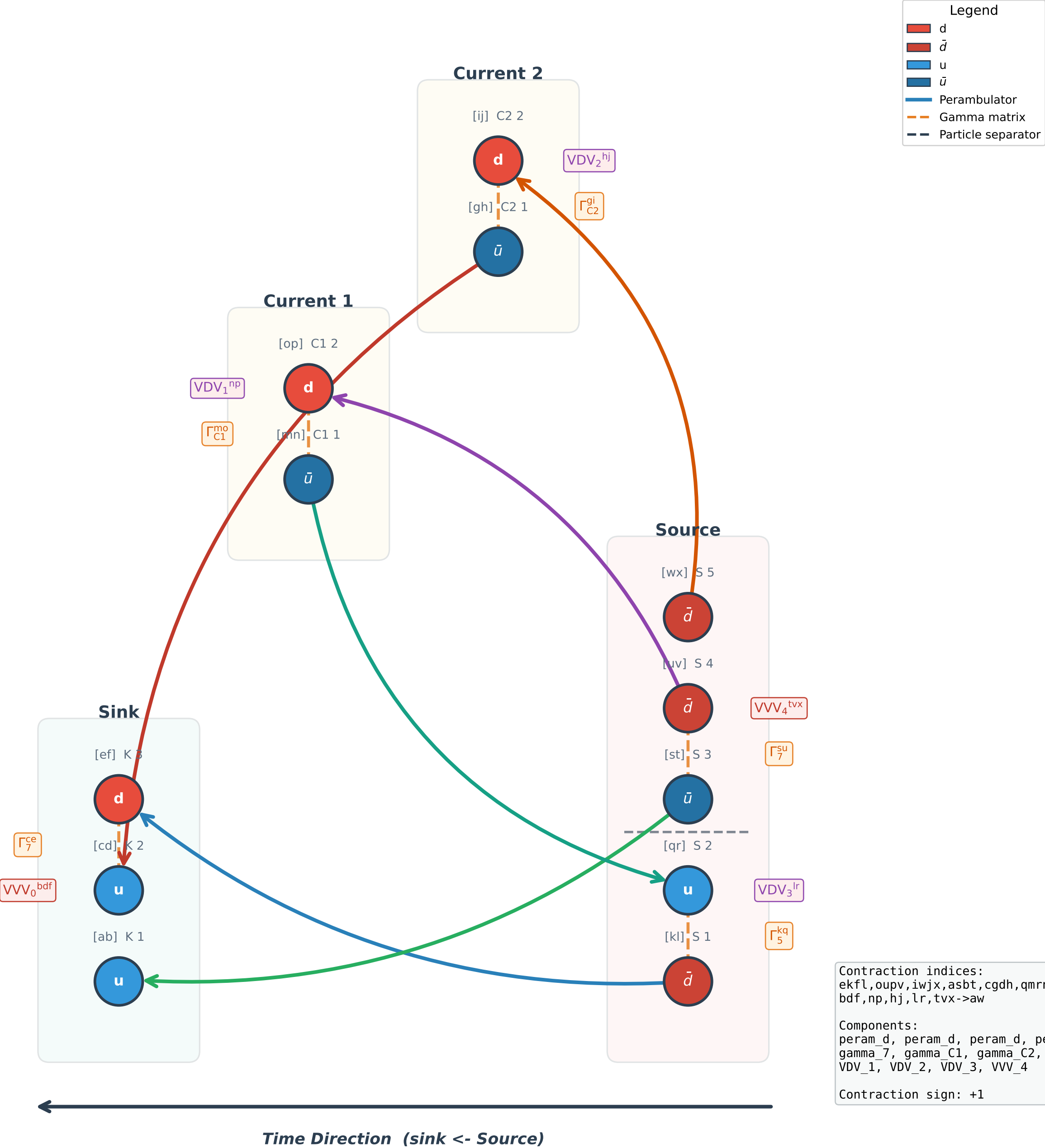
Wick Contraction Diagram #6 (3pt, sign = +1)
