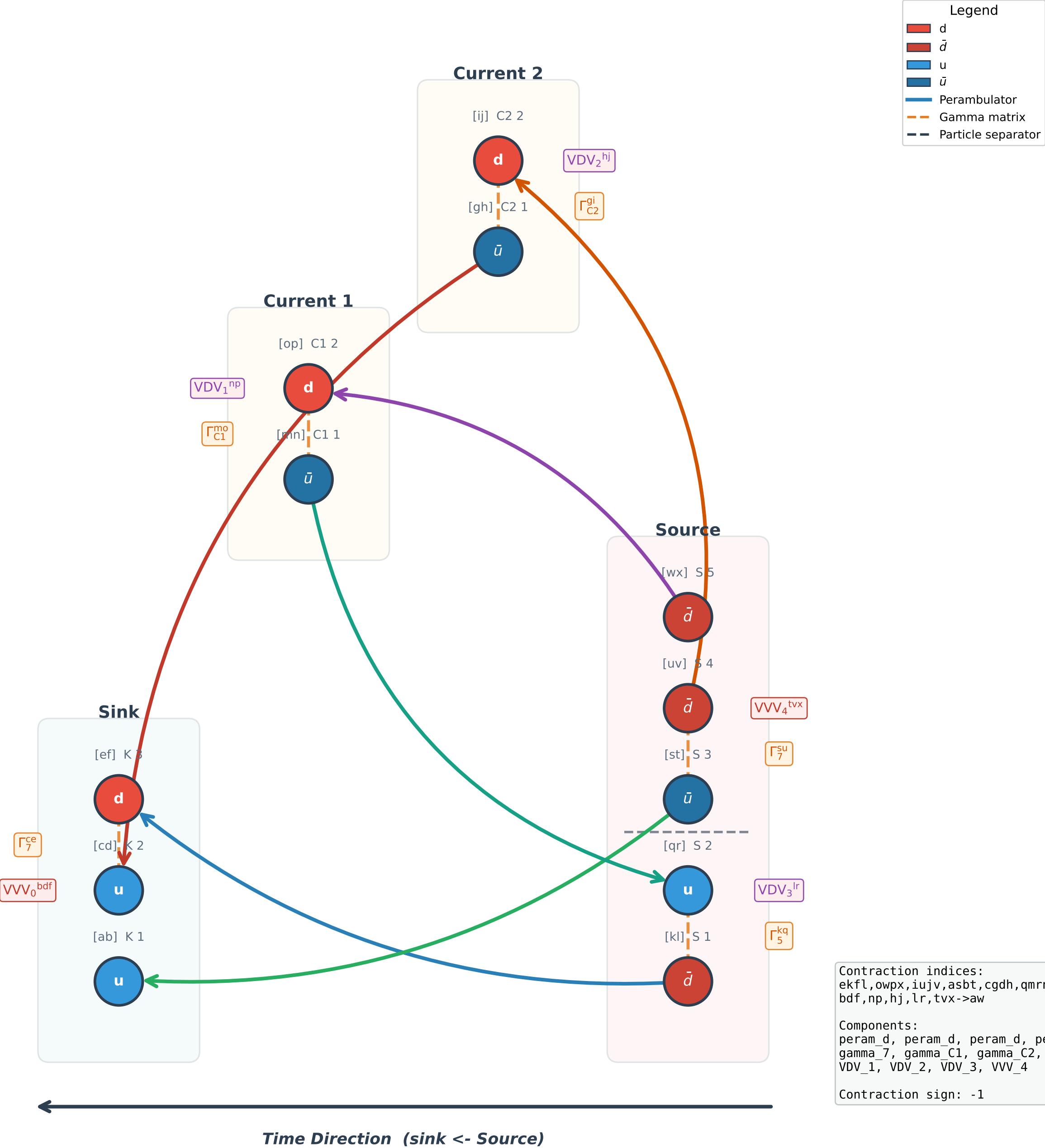
Wick Contraction Diagram #12 (3pt, sign = -1)
