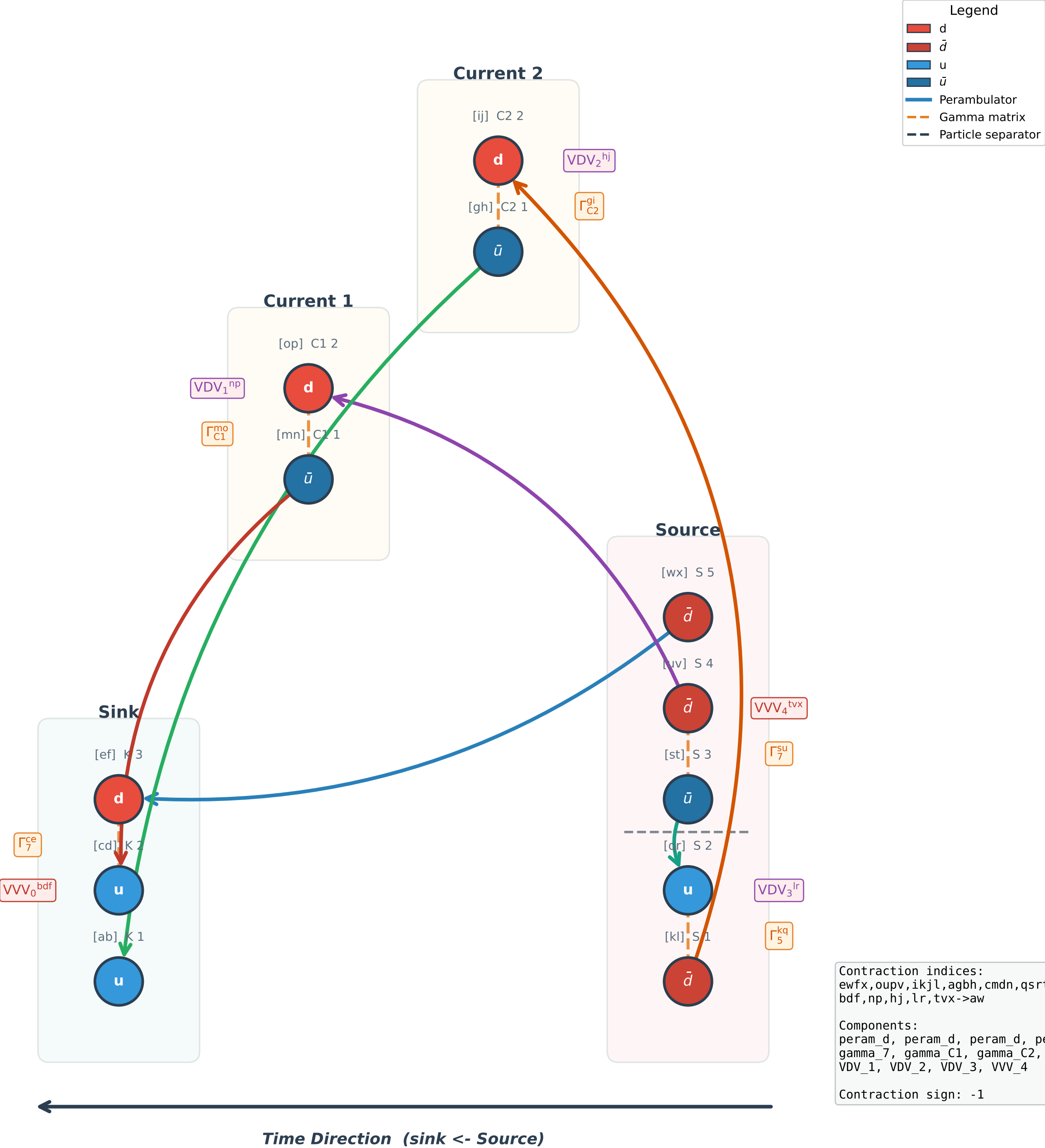
Wick Contraction Diagram #33 (3pt, sign = -1)
