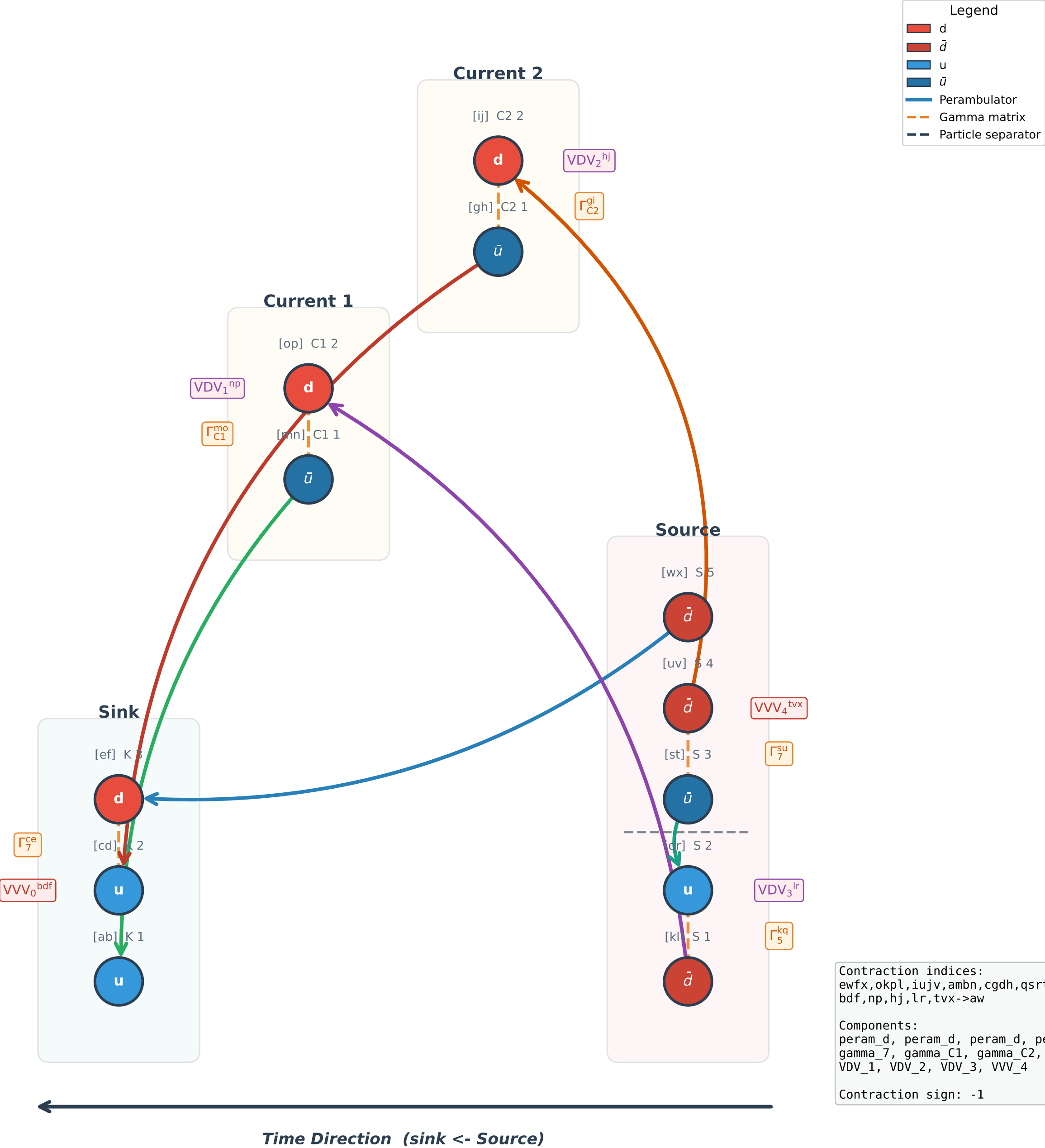
Wick Contraction Diagram #25 (3pt, sign = -1)
