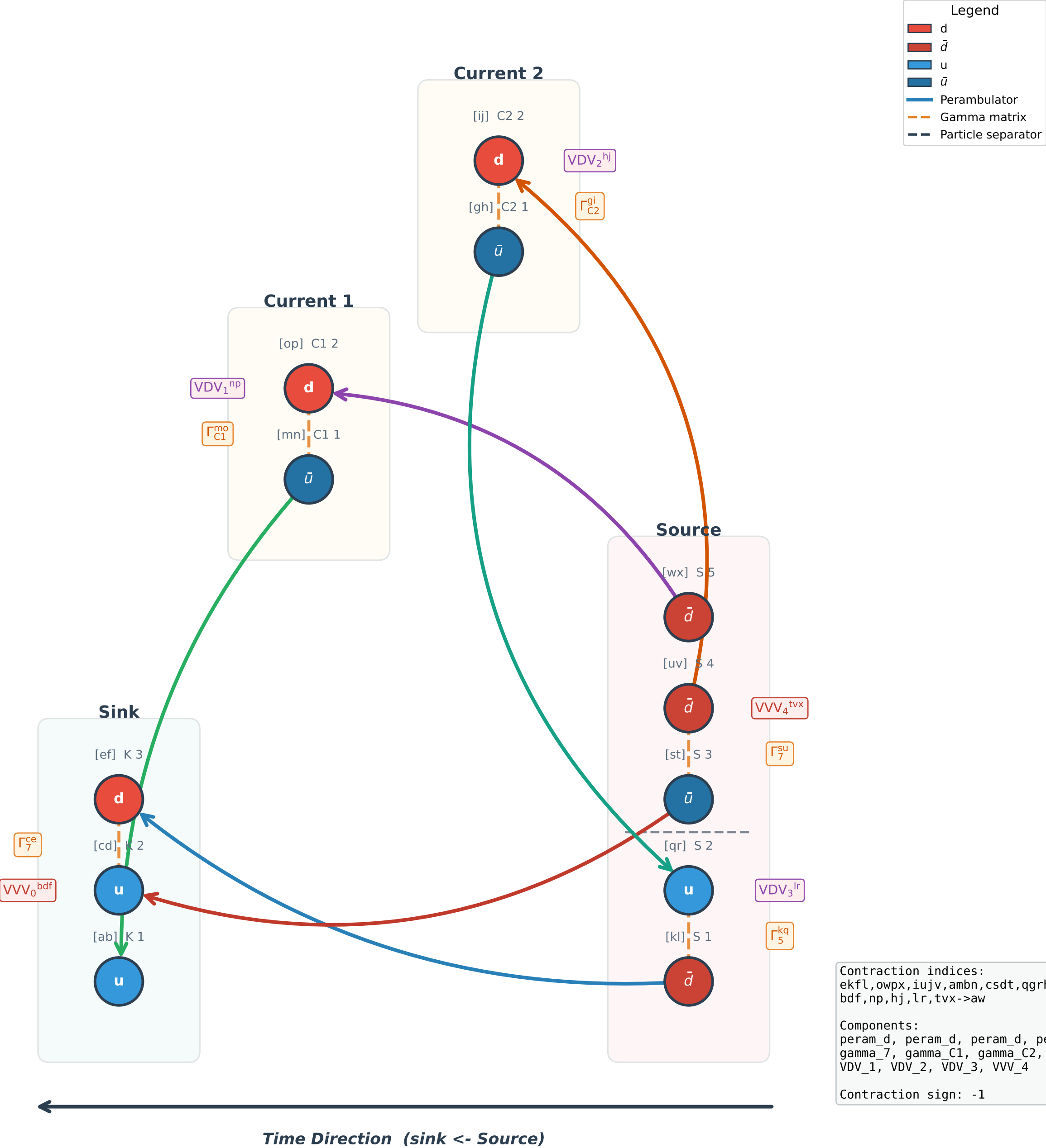
Wick Contraction Diagram #8 (3pt, sign = -1)
