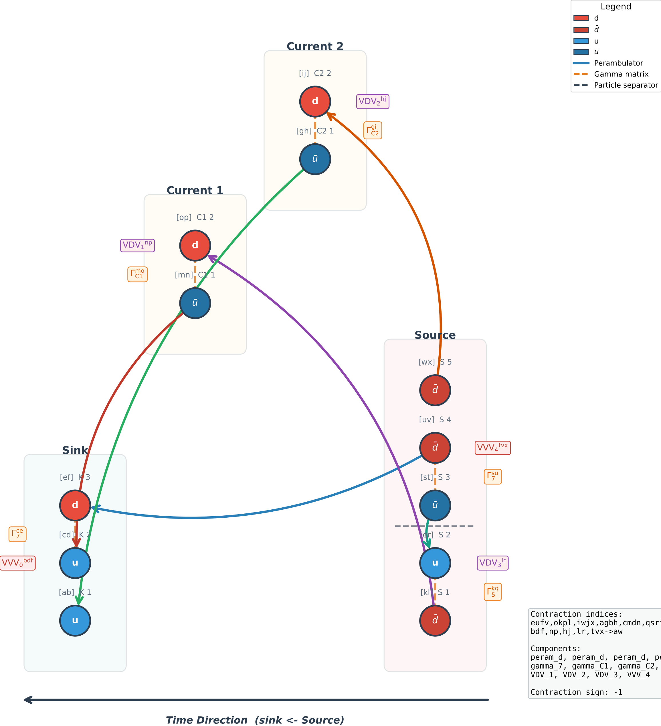
Wick Contraction Diagram #15 (3pt, sign = -1)
