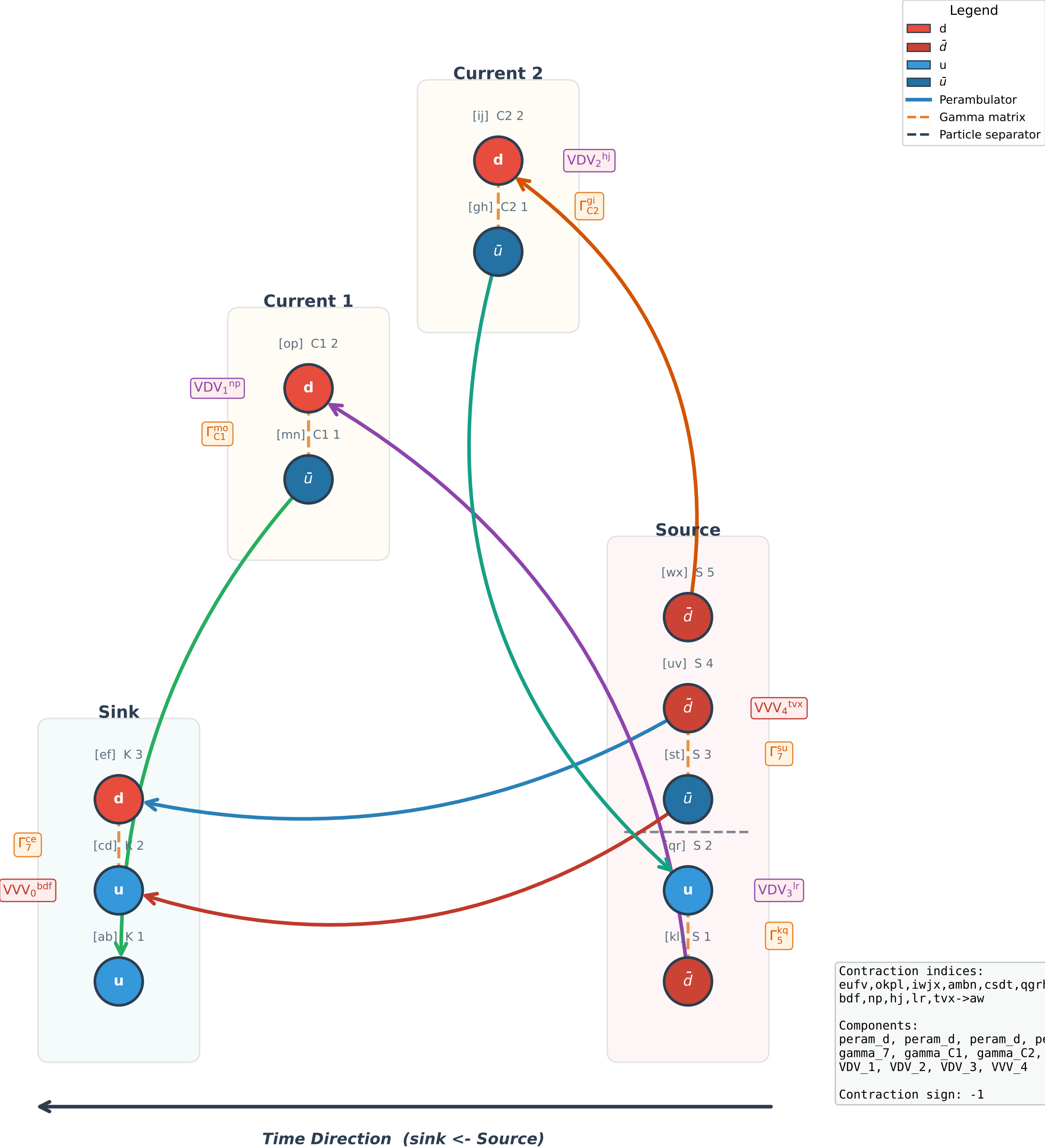
Wick Contraction Diagram #14 (3pt, sign = -1)
