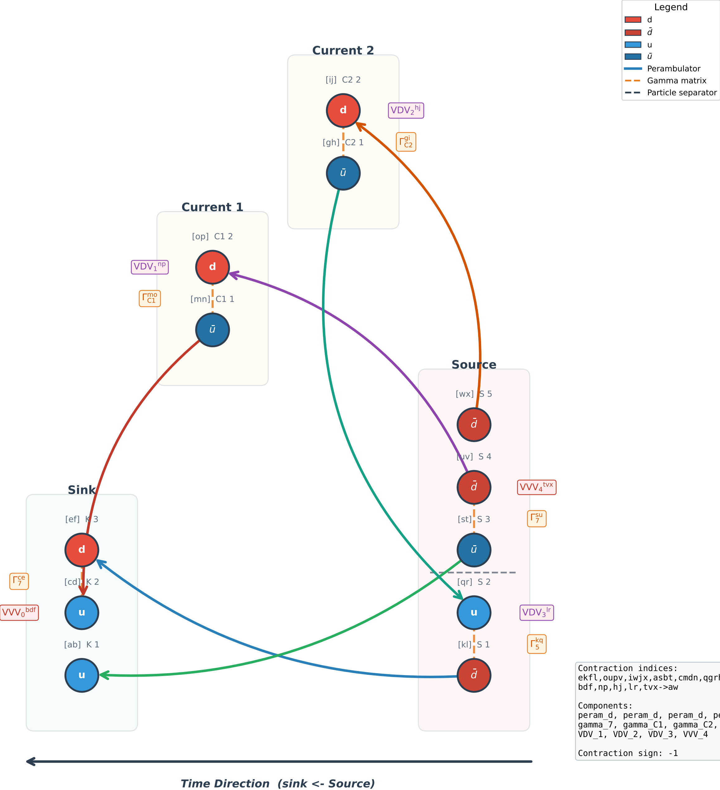
Wick Contraction Diagram #5 (3pt, sign = -1)
