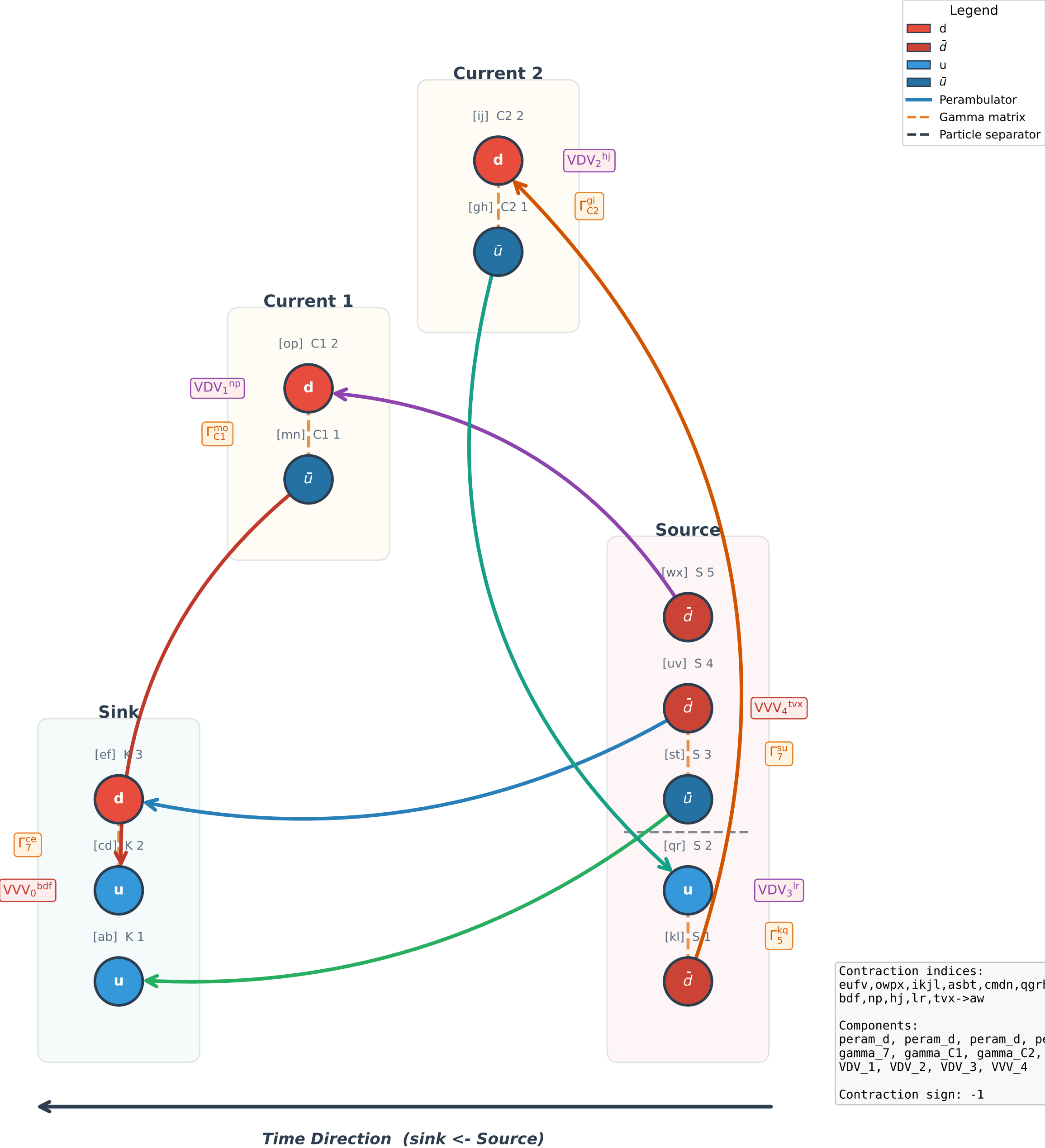
Wick Contraction Diagram #23 (3pt, sign = -1)
