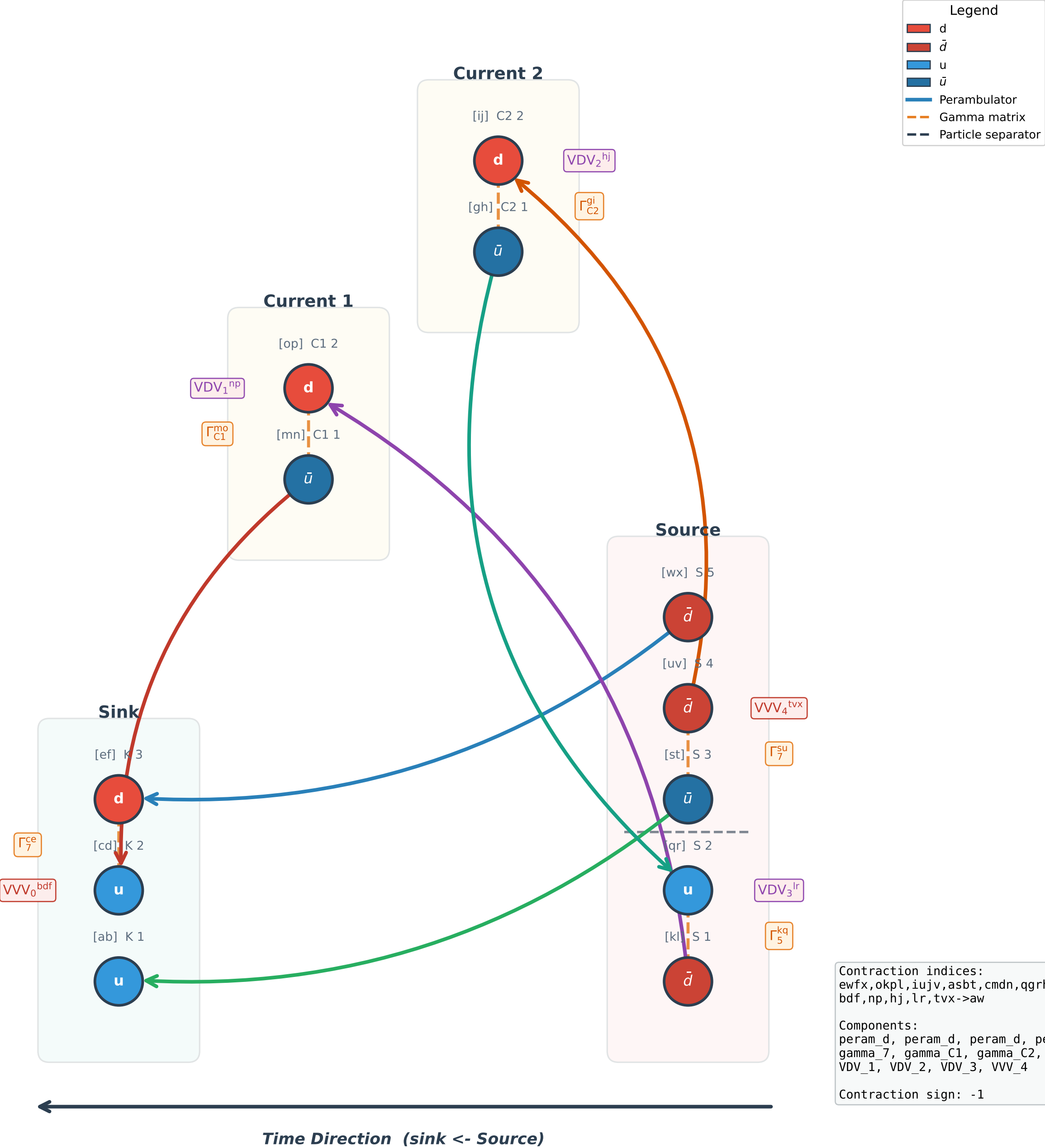
Wick Contraction Diagram #29 (3pt, sign = -1)
