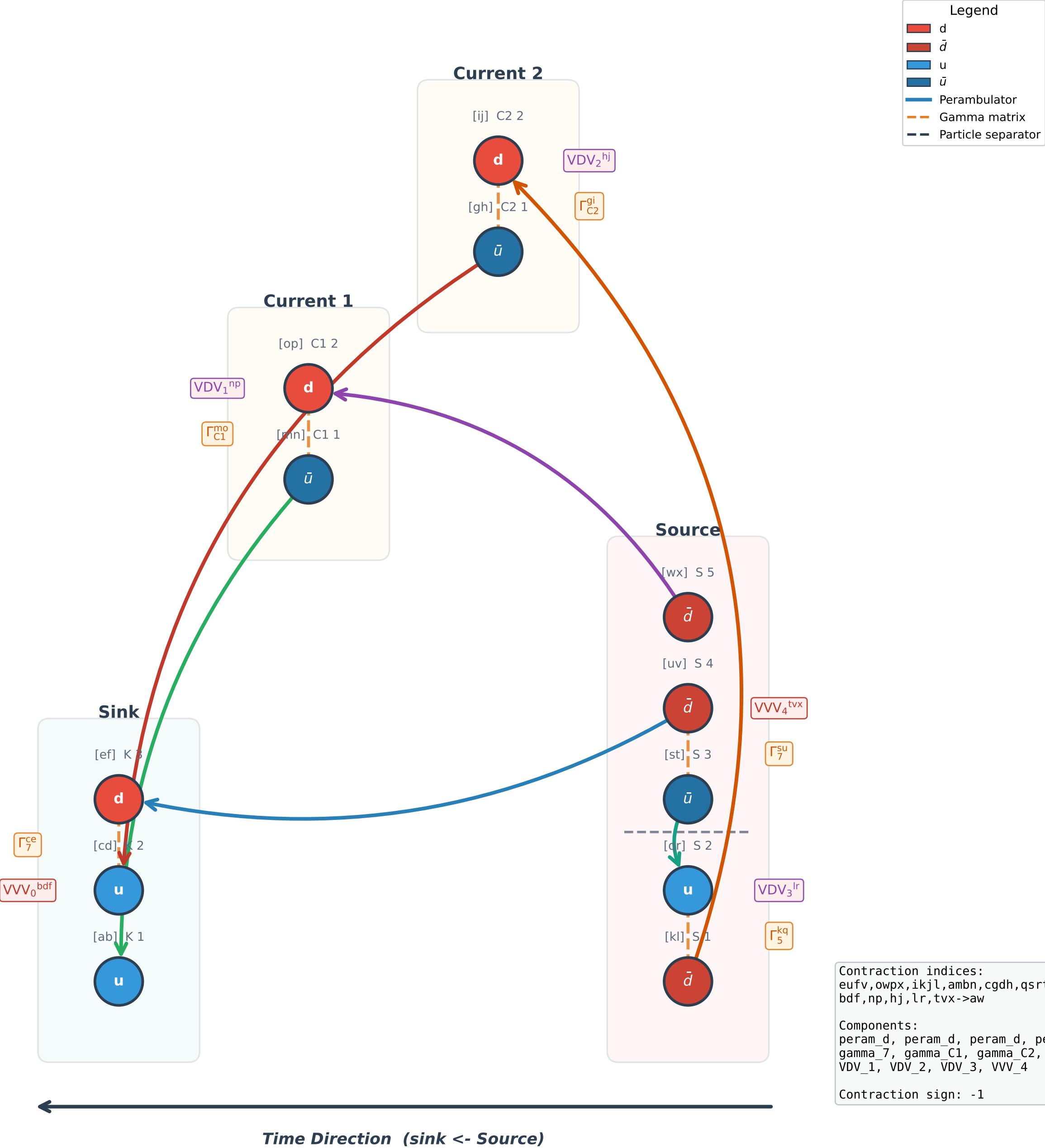
Wick Contraction Diagram #19 (3pt, sign = -1)
