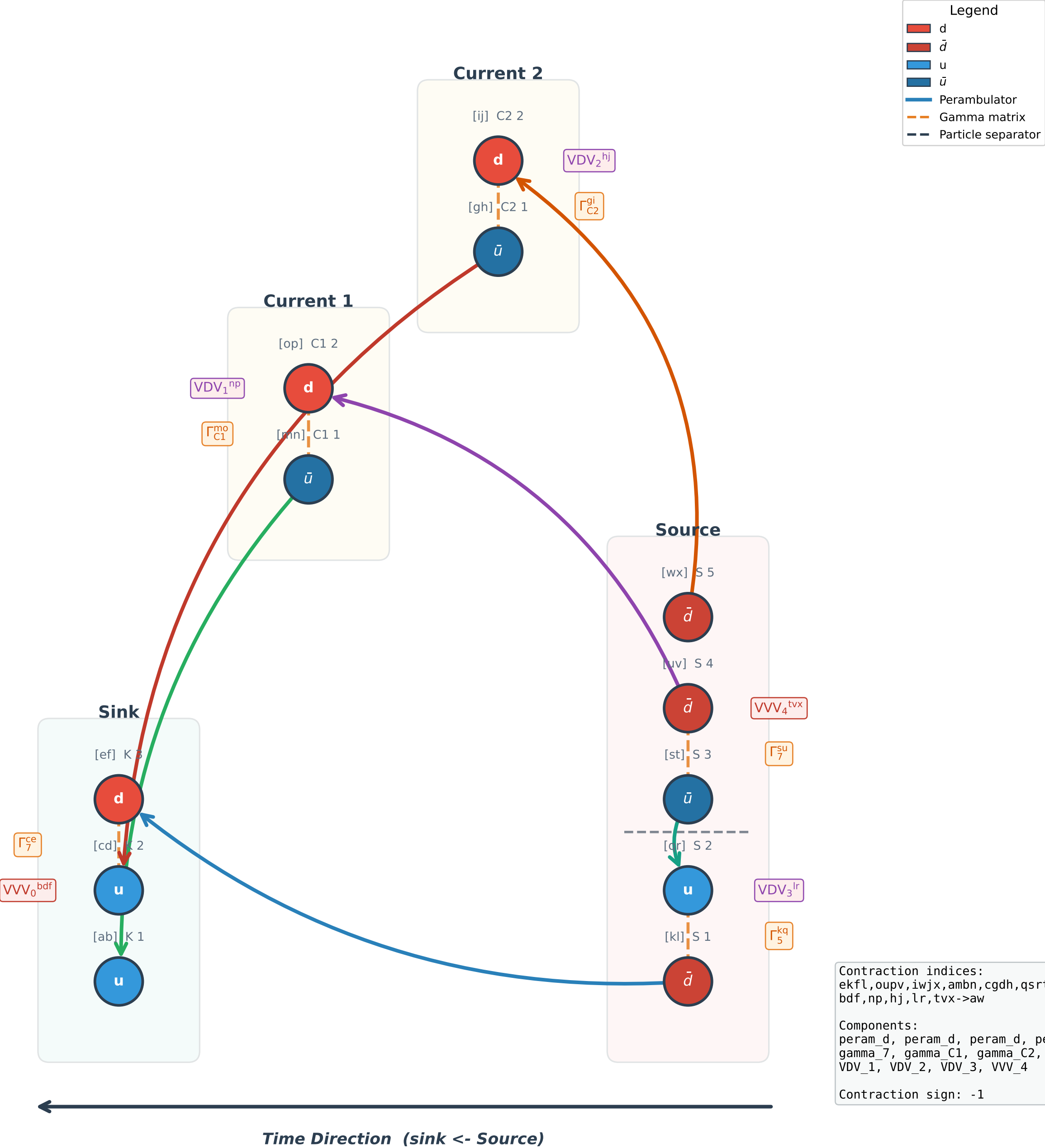
Wick Contraction Diagram #1 (3pt, sign = -1)
