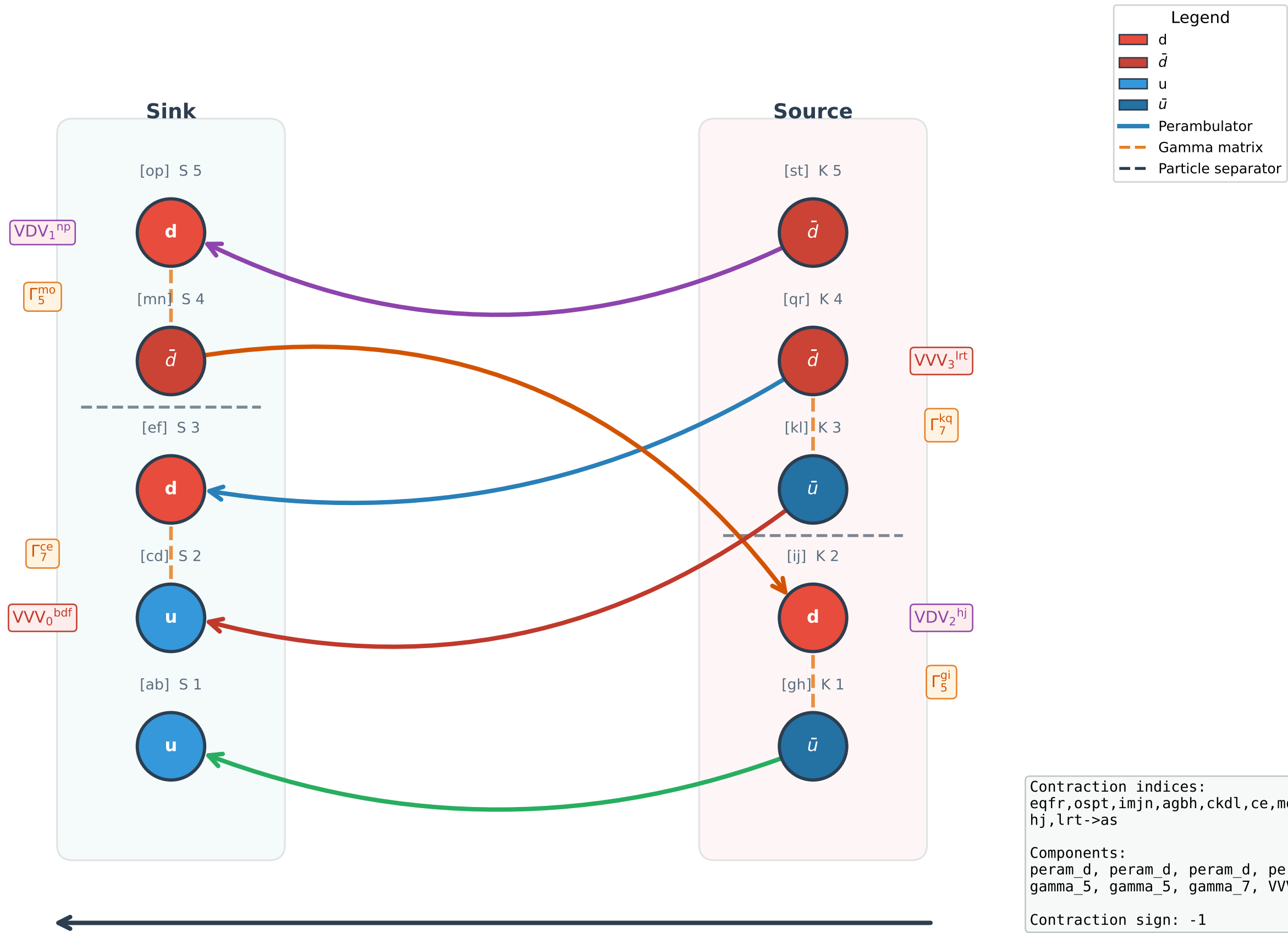
Wick Contraction Diagram #7 (2pt, sign = -1)
