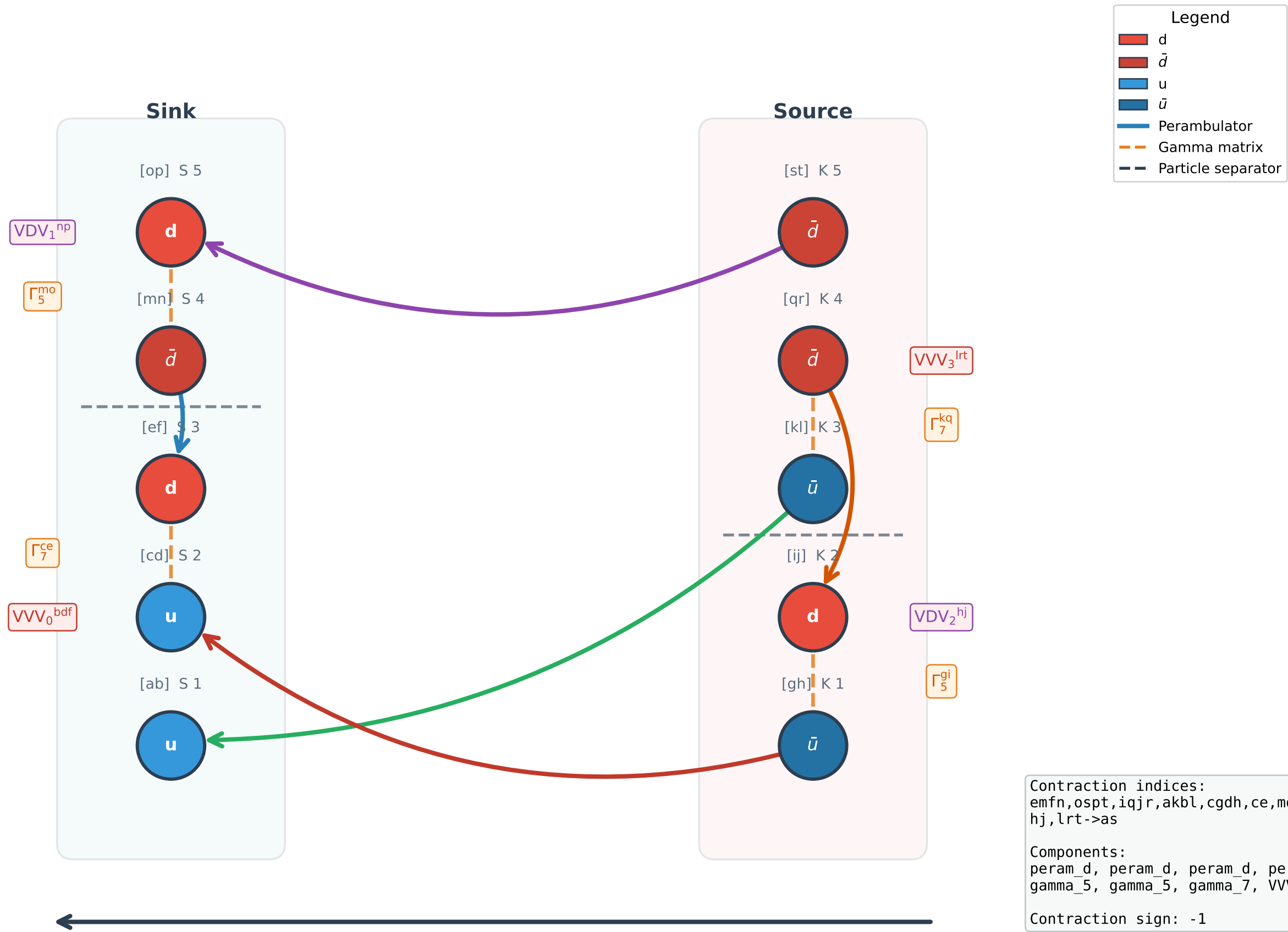
Wick Contraction Diagram #4 (2pt, sign = -1)
