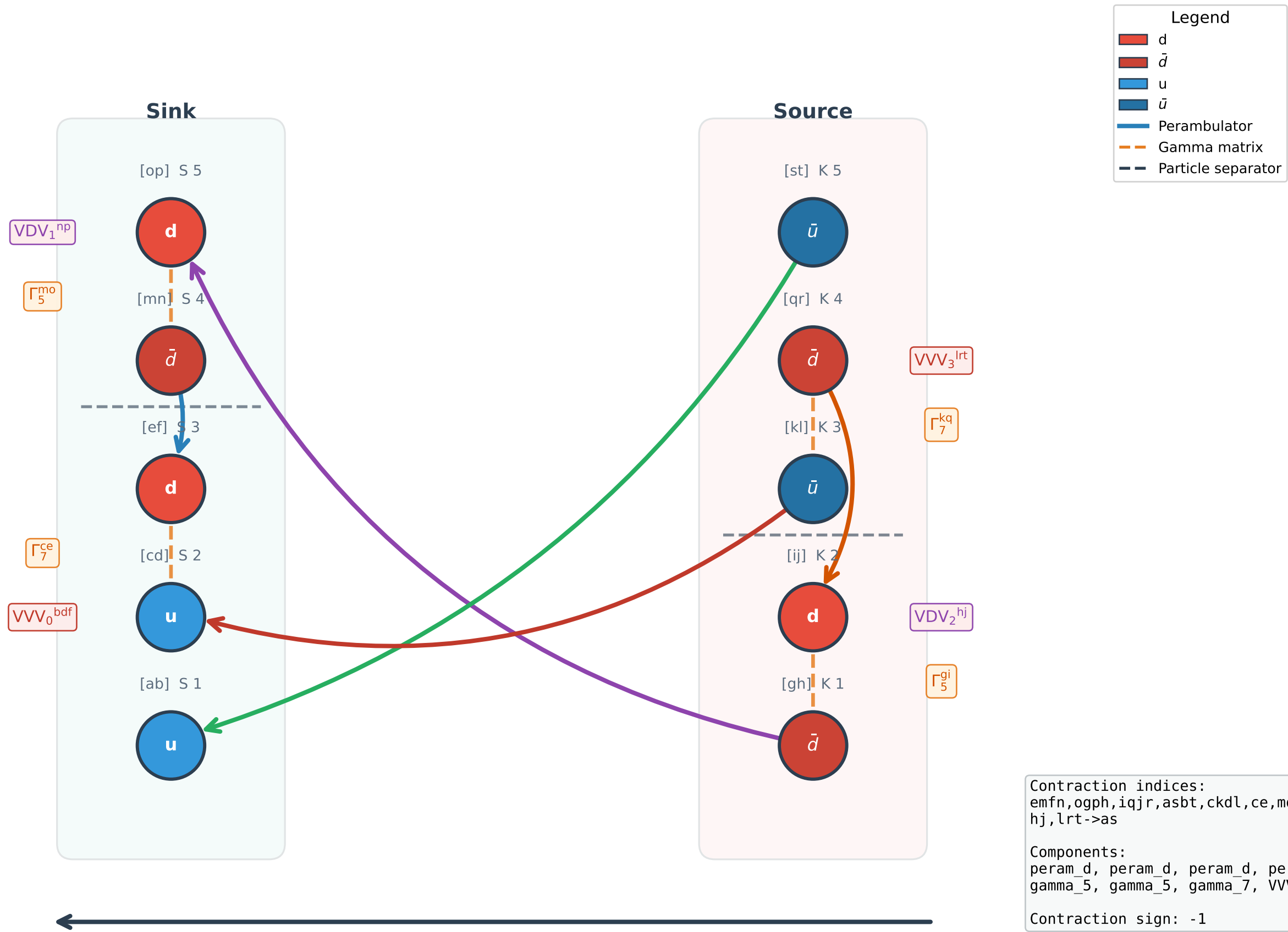
Wick Contraction Diagram #2 (2pt, sign = -1)
