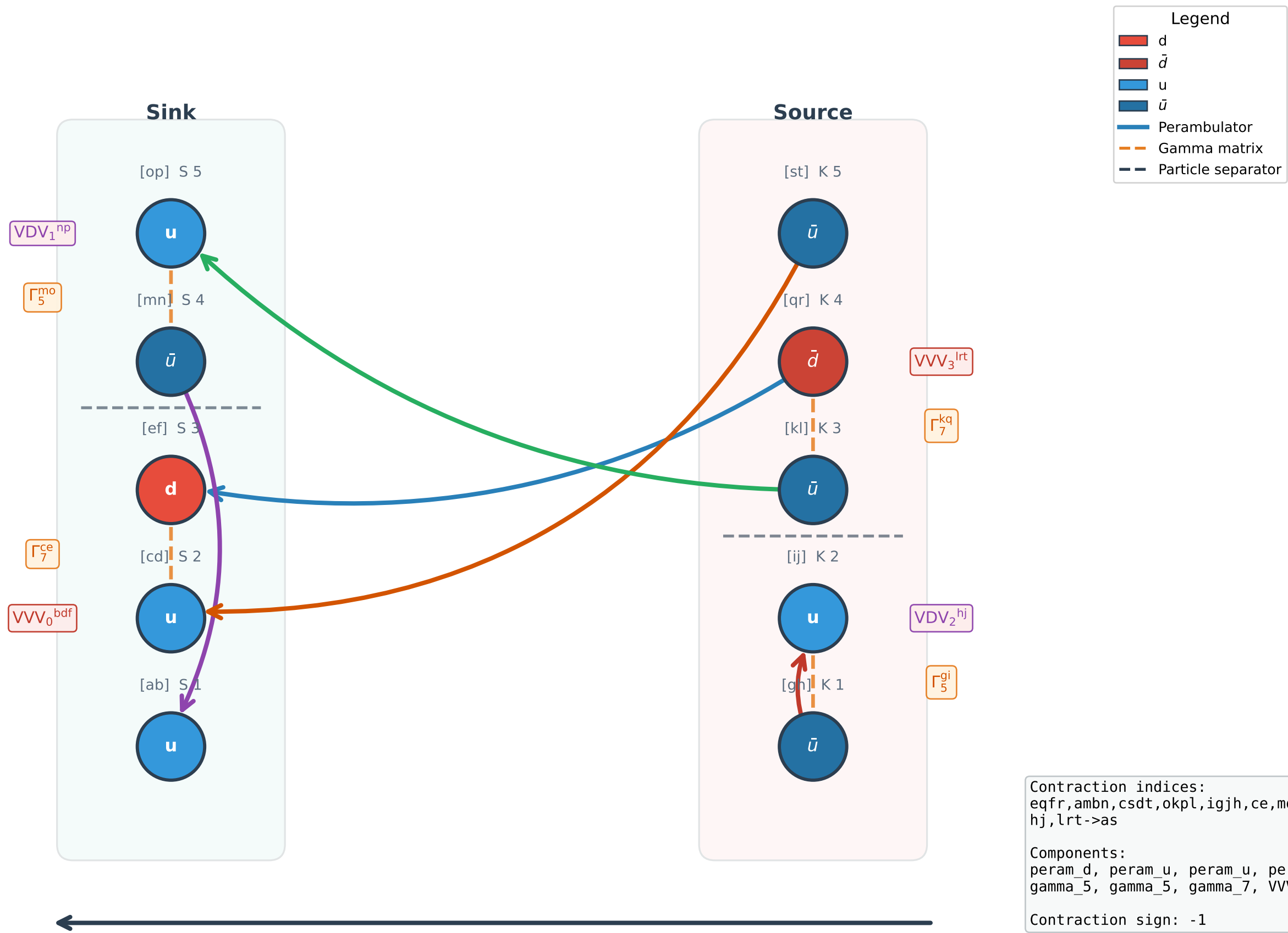
Wick Contraction Diagram #6 (2pt, sign = -1)
