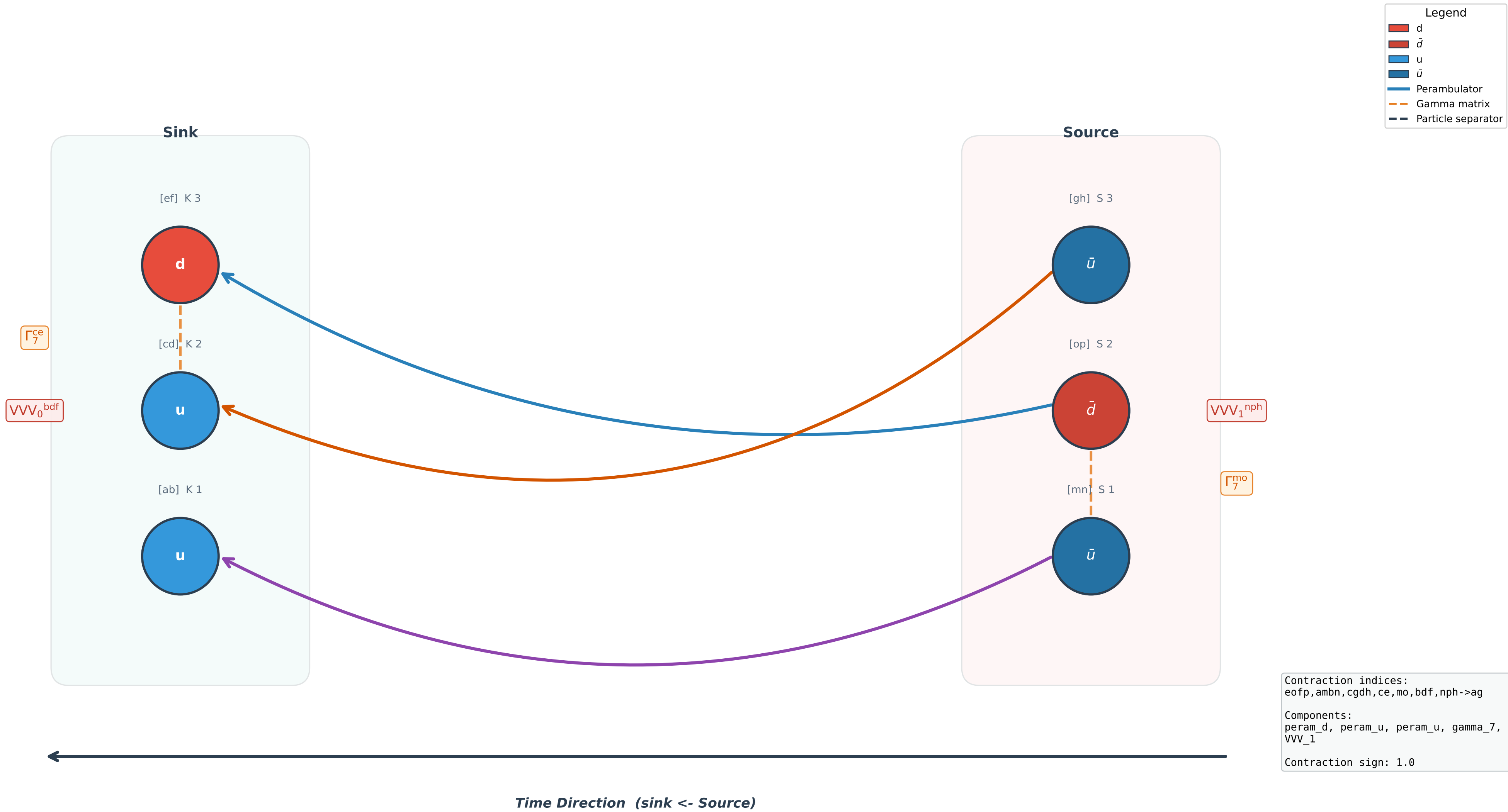
Wick Contraction Diagram #0 (2pt, sign = 1.0)
