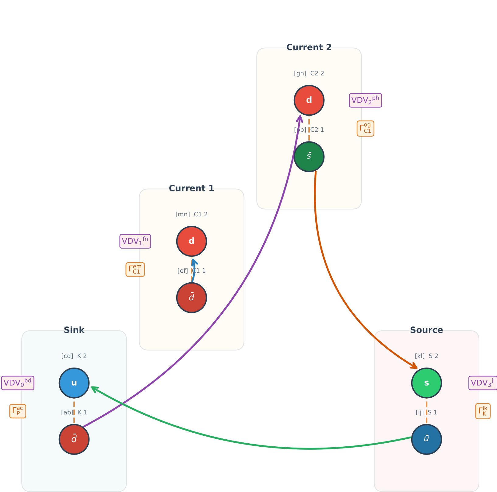
Wick Contraction Diagram #1 (3pt, sign = 1.0)
