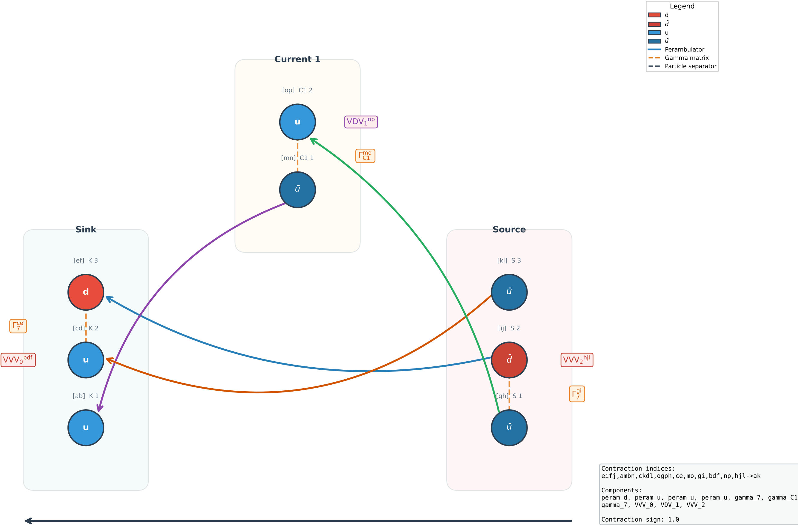
Wick Contraction Diagram #1 (3pt, sign = 1.0)
