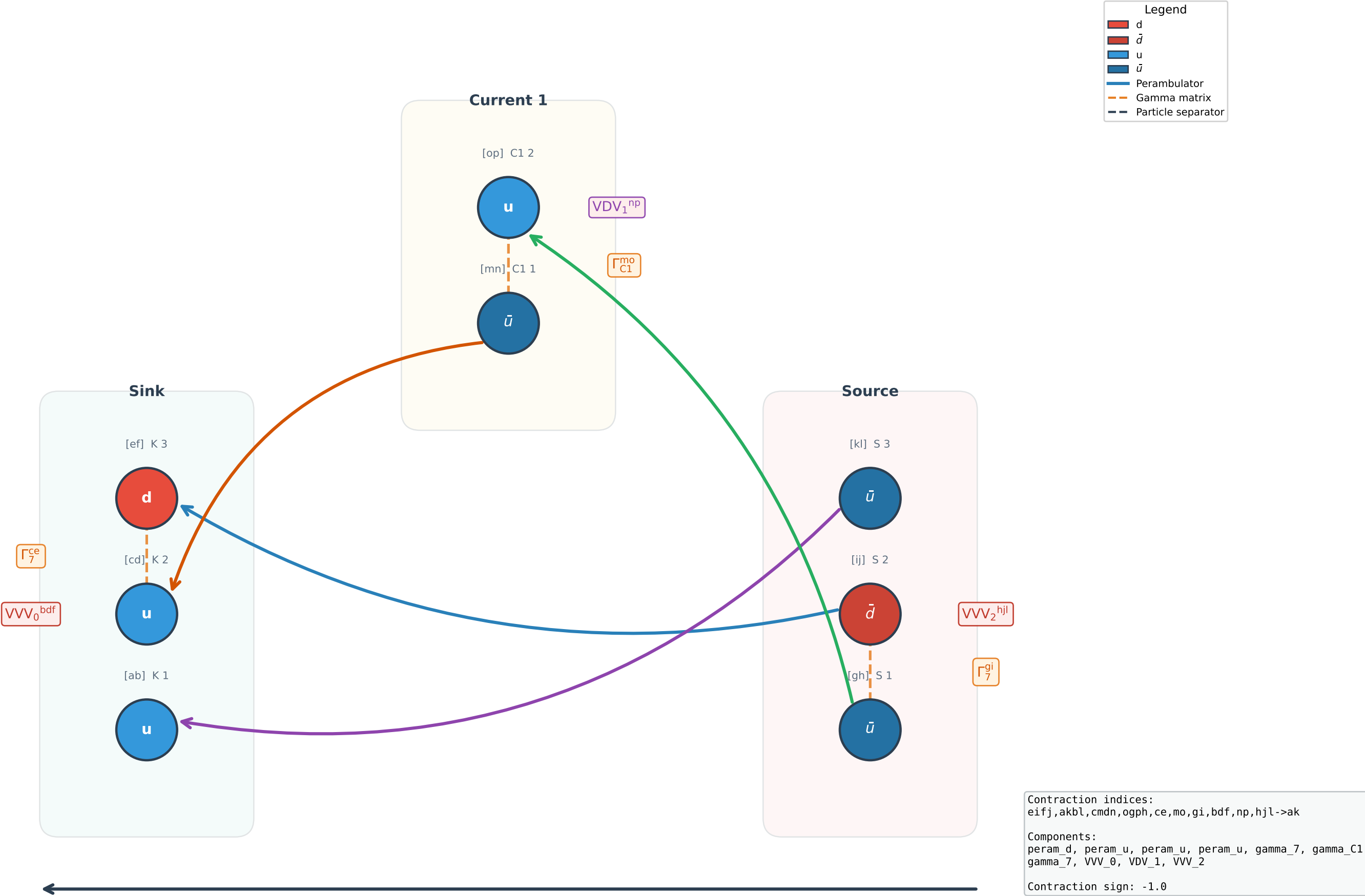
Wick Contraction Diagram #4 (3pt, sign = -1.0)
