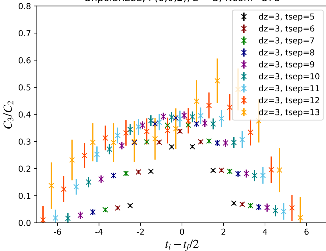
Unpolarized, P(0,0,2), z = 3 , Nconf=878
