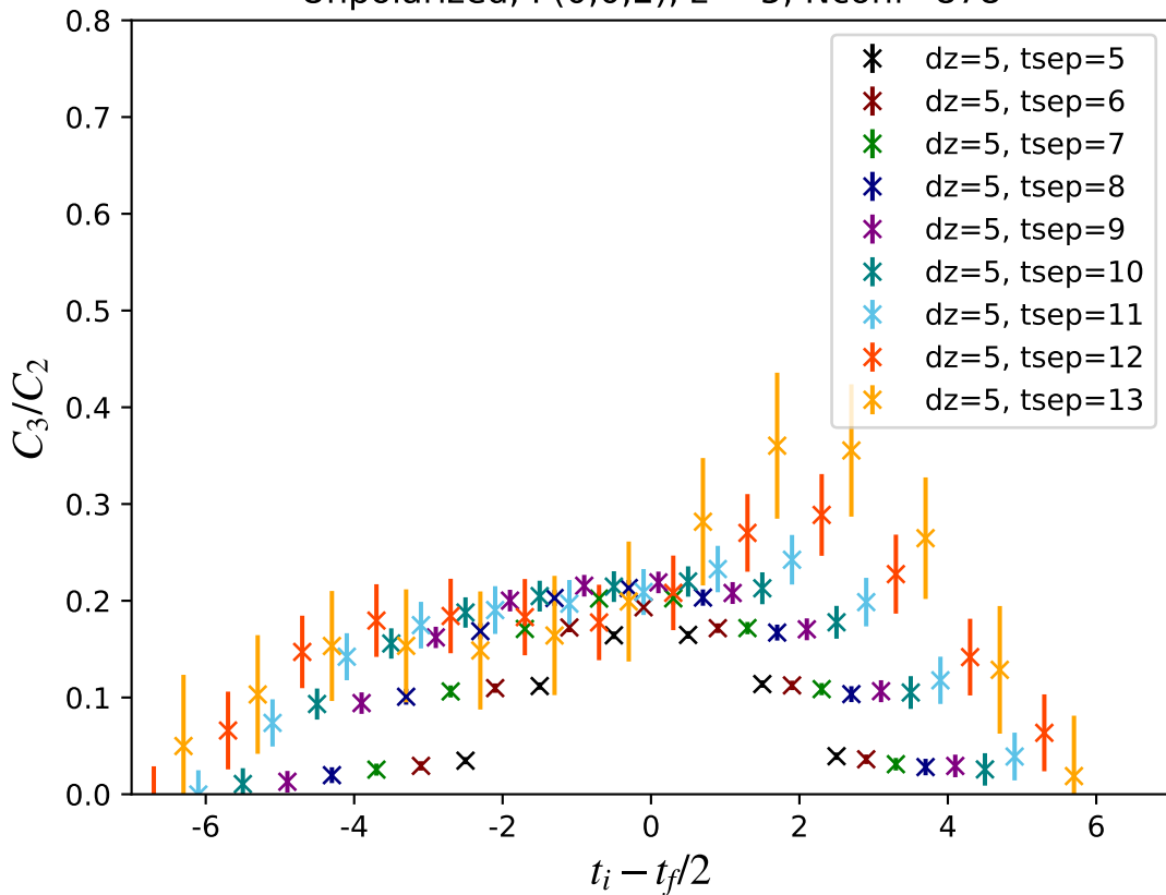
Unpolarized, P(0,0,2), z = 5 , Nconf=878
