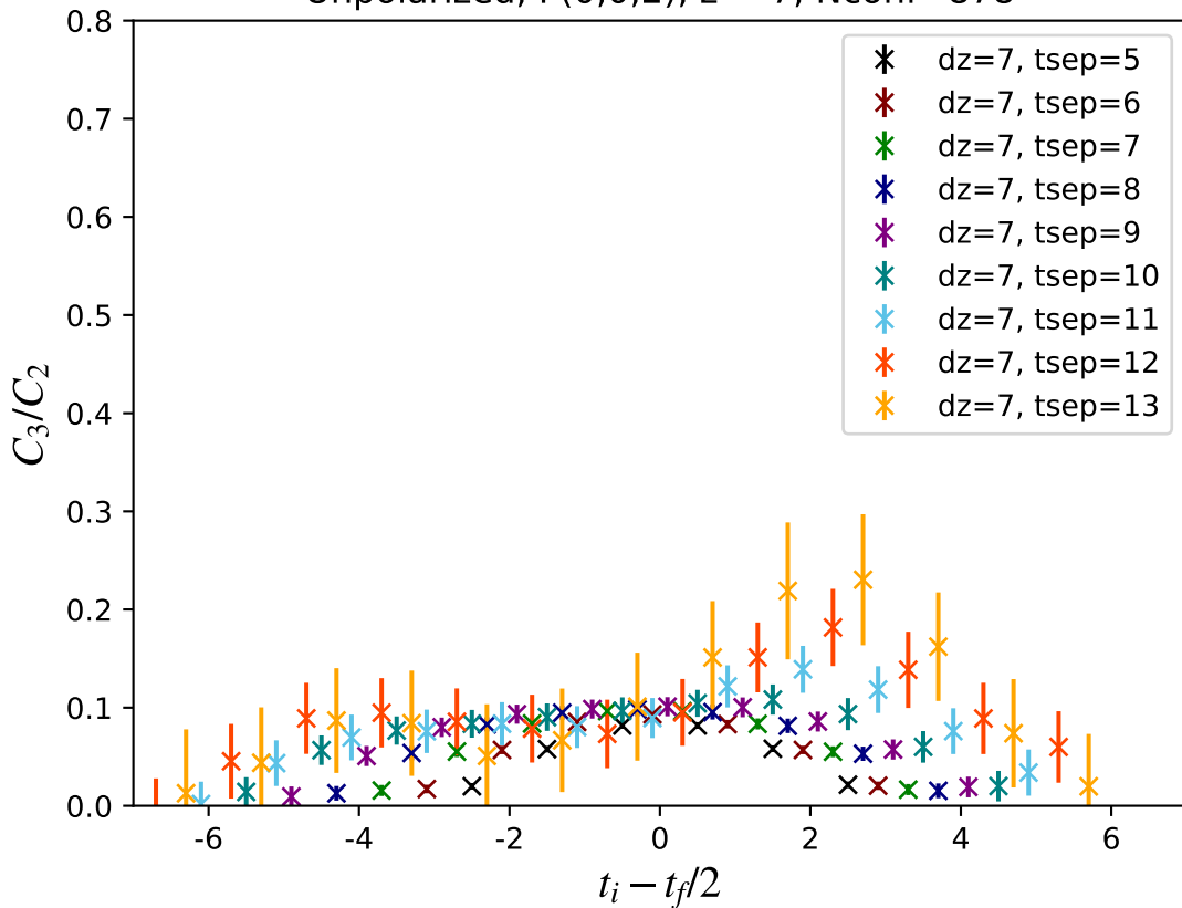
Unpolarized, P(0,0,2), z = 7 , Nconf=878
