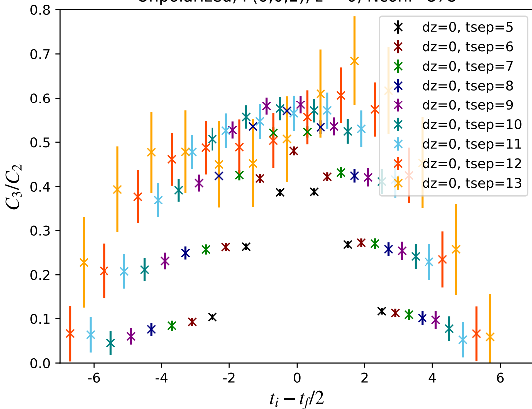
Unpolarized, P(0,0,2), z = 0 , Nconf=878
