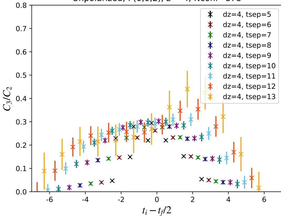
Unpolarized, P(0,0,2), z = 4 , Nconf=878
