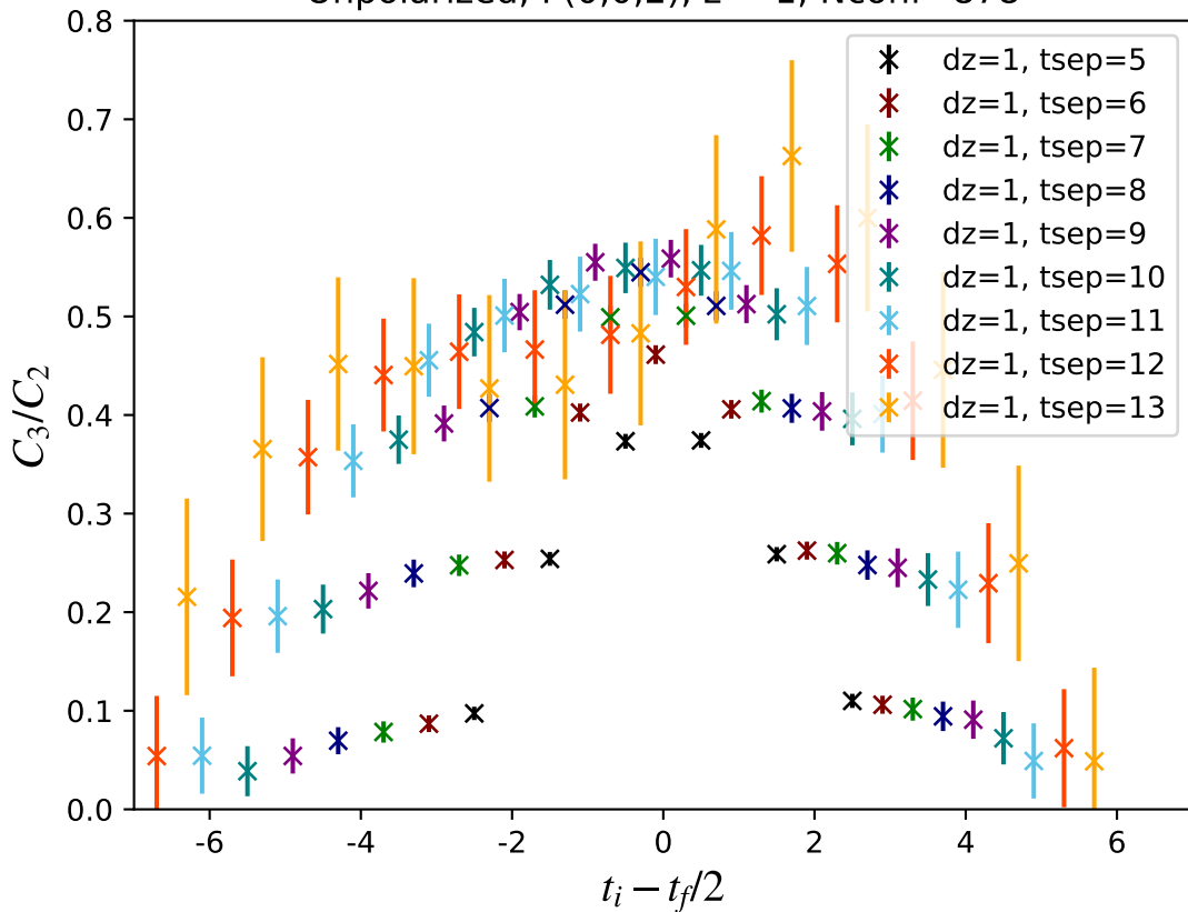
Unpolarized, P(0,0,2), z = 1 , Nconf=878
