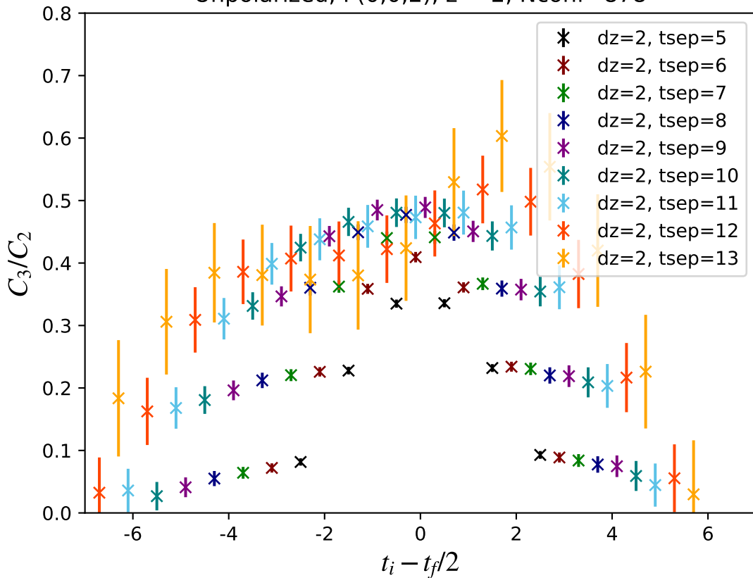
Unpolarized, P(0,0,2), z = 2 , Nconf=878
